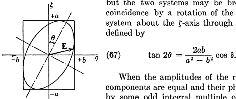
FIG. 46.—Polarization ellipse.
