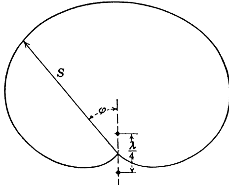
FIG. 82.—Radiation pattern in the equatorial plane of two half-wave oscillators 90 deg. out of phase and with quarter-wave spacing.
