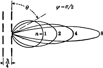
FIG. 84.—Radiation patterns in the meridian plane for a vertical set of half-wave oscillators backed by reflectors. (Holtmann.)
