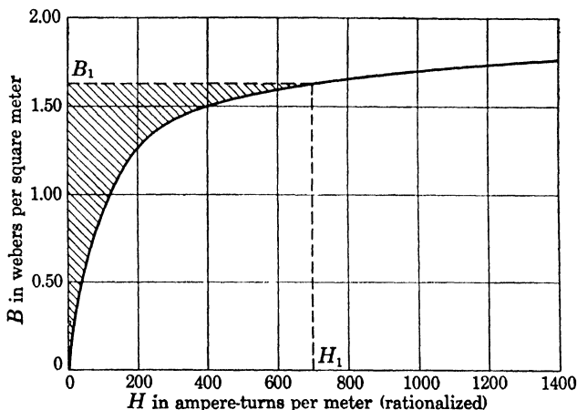
FIG. 20.—Typical magnetization curve for annealed sheet steel.
