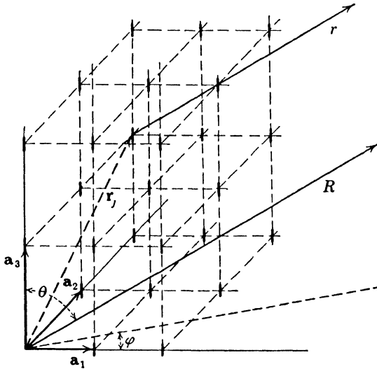
FIG. 80.—A system of half-wave oscillators arrayed in a regular lattice structure defined by the base vectors \mathbf{a}_1 , \mathbf{a}_2 , \mathbf{a}_3 .
