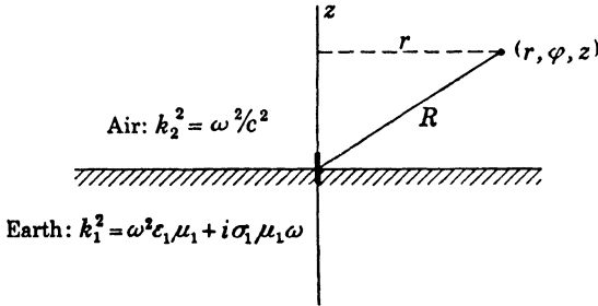
FIG. 113.—Vertical electric dipole located at the surface of a plane, finitely conducting earth.
