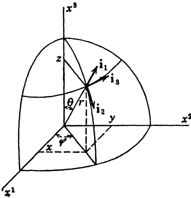
FIG. 8.—Spherical coordinates.
