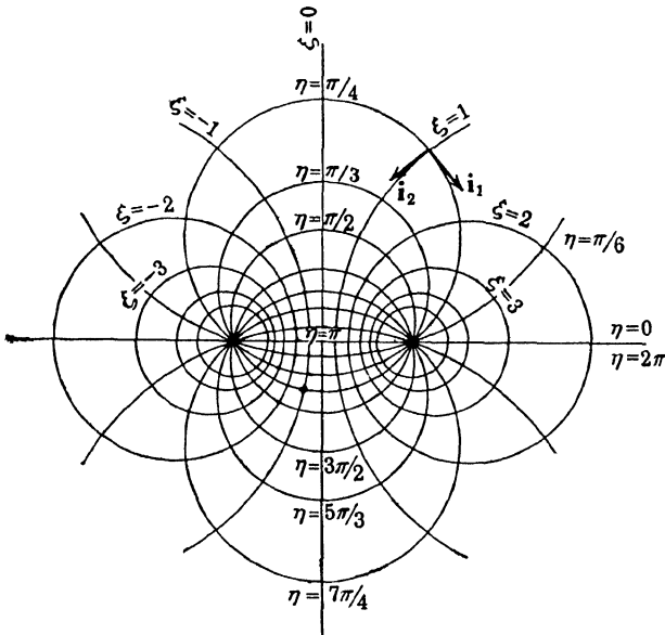
FIG. 11.—Bipolar coordinates.
