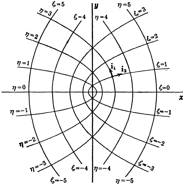
FIG. 10.—Parabolic coordinates.
