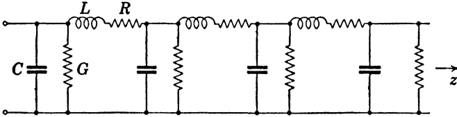
FIG. 109.—Schematic representation of a distributed parameter transmission line.
