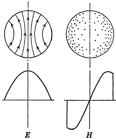
FIG. 111.—The lowest electric mode of oscillation in a spherical resonator, showing the field in a meridian plane.
