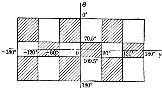
FIG. 69.—Nodes of the function \sin 3\phi P_3^3(\cos \theta) on the developed surface of a sphere. The function has negative values over the shaded areas.
