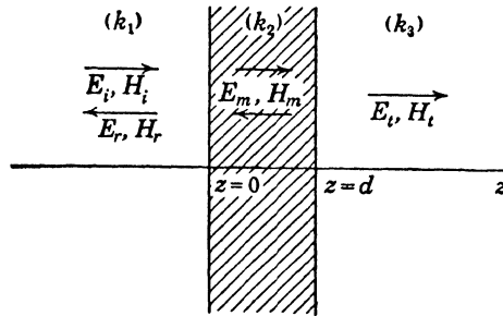
FIG. 96.—Reflection and transmission of plane waves by a plane sheet at normal incidence. Three arbitrary homogeneous media characterized by the propagation factors k_1, k_2, k_3 are separated by plane boundaries as shown in Fig. 96. We need deal only with the magnitudes of the vectors and write for the incident and reflected waves in medium (1):
