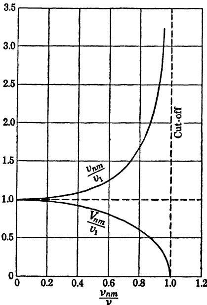
FIG. 106.—Phase and group velocities in a hollow pipe. v_1 = 1/\sqrt{\epsilon_1\mu_1} .
