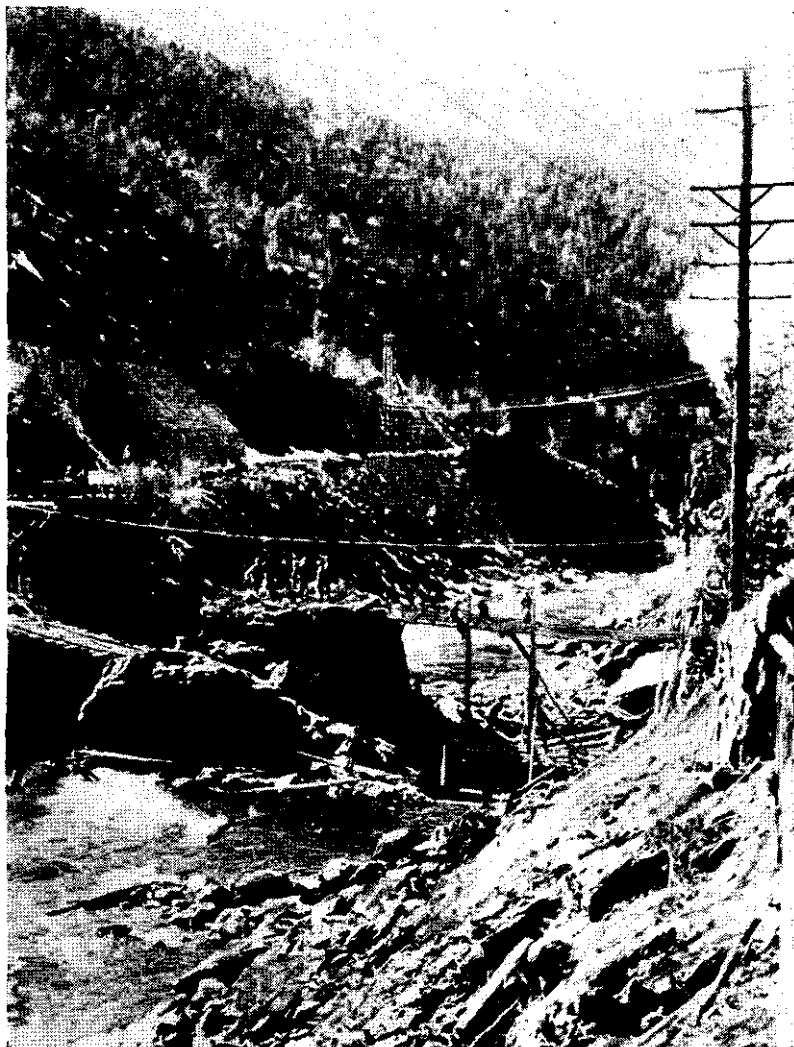
Figure 12.—Bridging a mountain stream during the Norwegian Campaign (1940).
