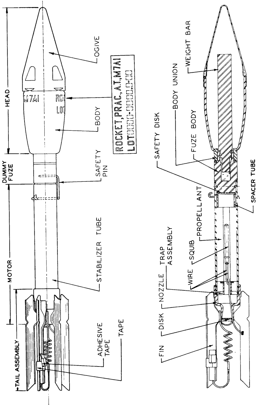
FIGURE 16. - ROCKET, PRACTICE, 2.36", M7A1
