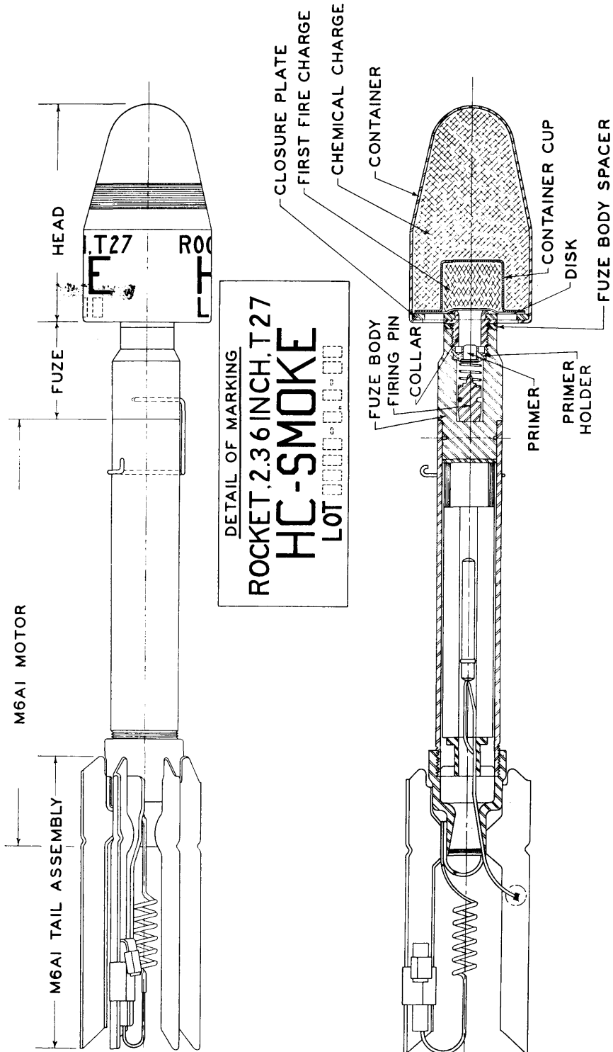
FIGURE 30. - ROCKET, SMOKE, HC, 2.36", T27
