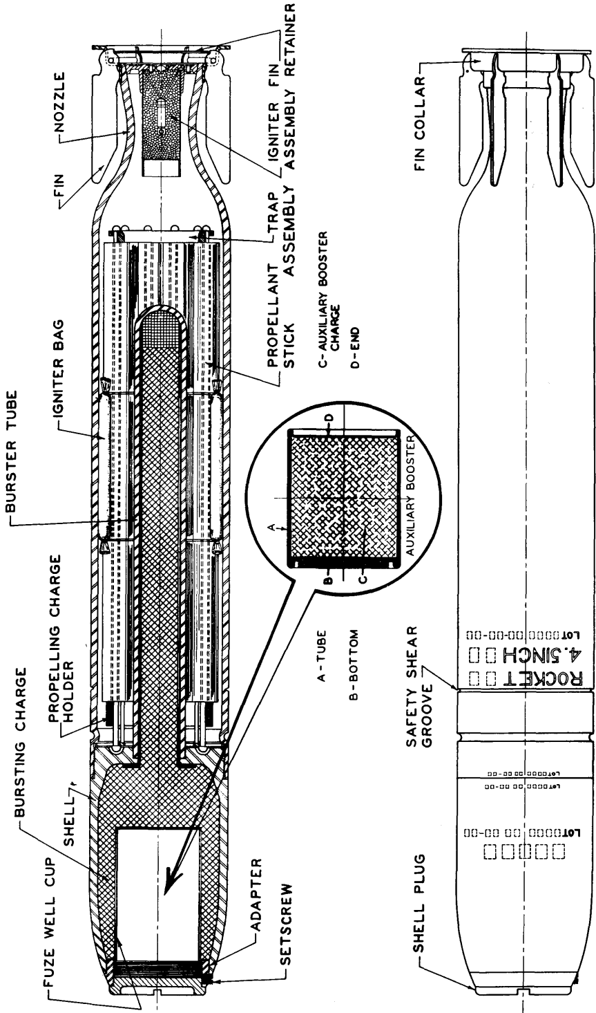
FIGURE 45. - ROCKET, H.E., 4.5", M8
