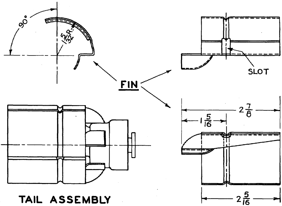
FIG.-18 TAIL ASSEMBLY SECTION IV
