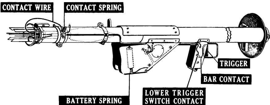
FIGURE 7. - ROCKET LAUNCHER, M1A1
