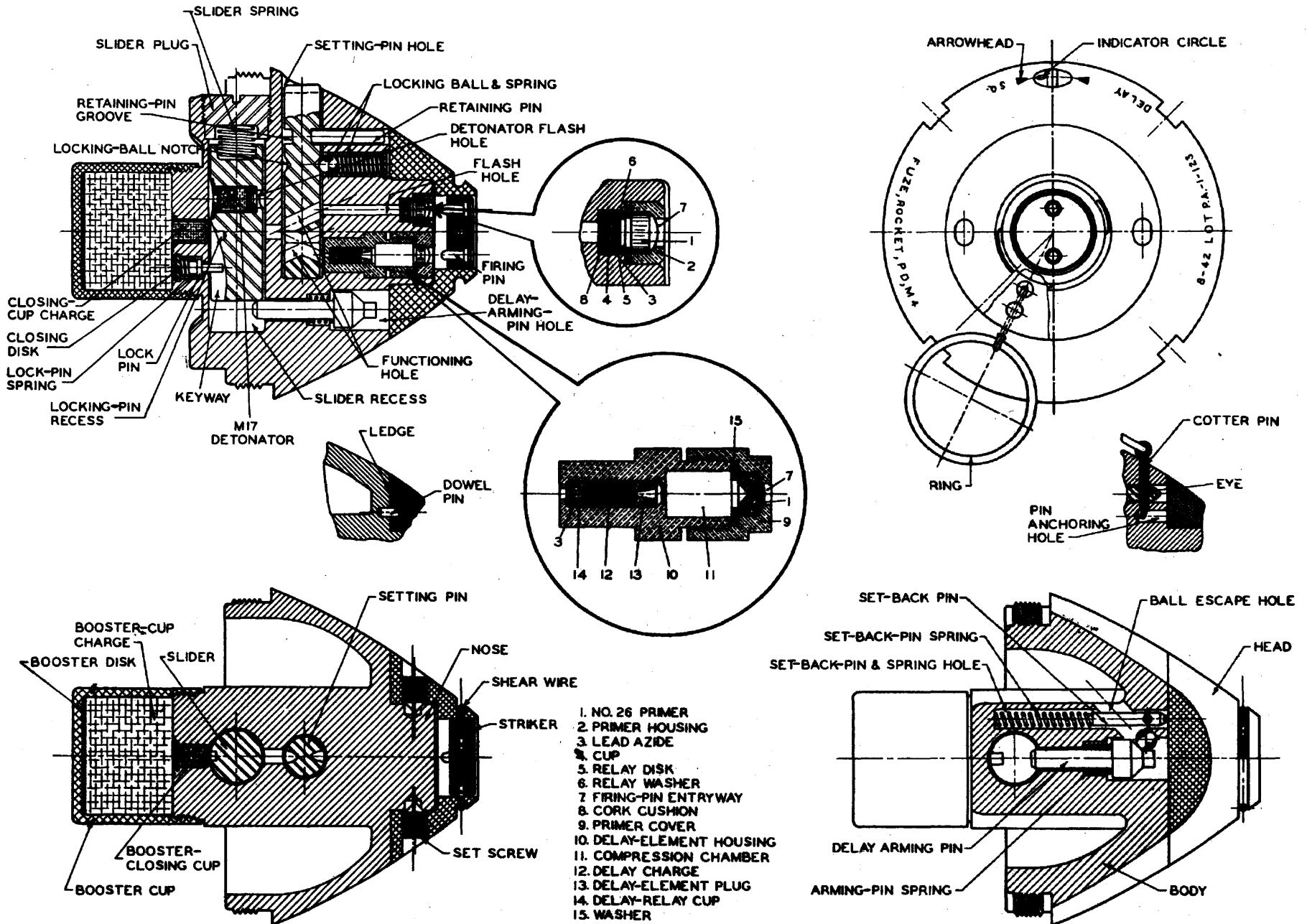
FIGURE 37. - FUZE, POINT DETONATING, M4
