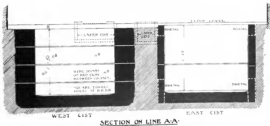
FIG. 335 B. SECTION OF 'TEMPLE REPOSITORIES'.
