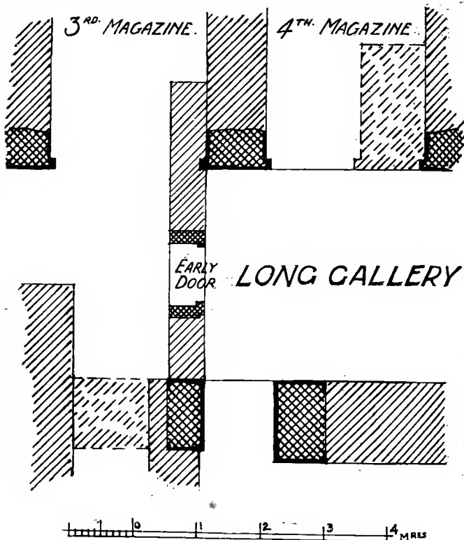
FIG. 323. PLAN OF CROSS WALL AND DOORWAY MADE TO SECURE ENCLAVE OF 'KASELLES'.
