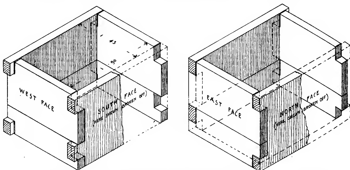
FIG. 334. TWO DIAGRAMMATIC VIEWS OF EAST CIST OF REPOSITORIES (M.M. III) SHOWING INTERLOCKING JOINTS OF SLABS.
