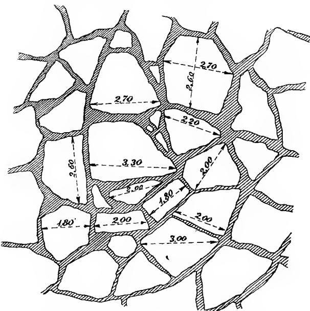
FIG. 222 a . PAVING OF GREAT BREAKWATER.
