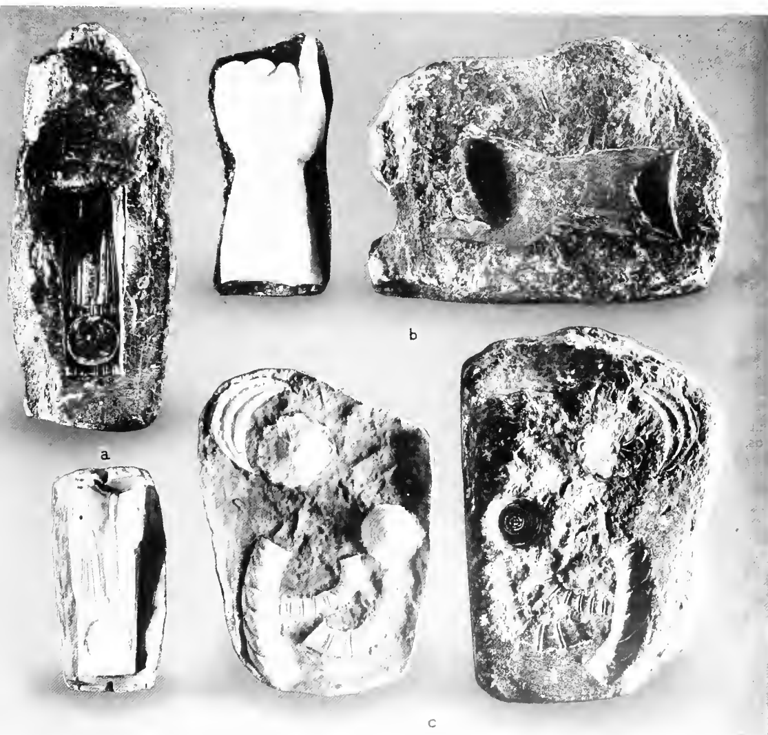
FIG. 349. BLACK STEATITE MATRICES FOR MOULDING FAÏENCE OBJECTS, WITH MOULDINGS BESIDE IT. ( \frac{2}{3} c.)
