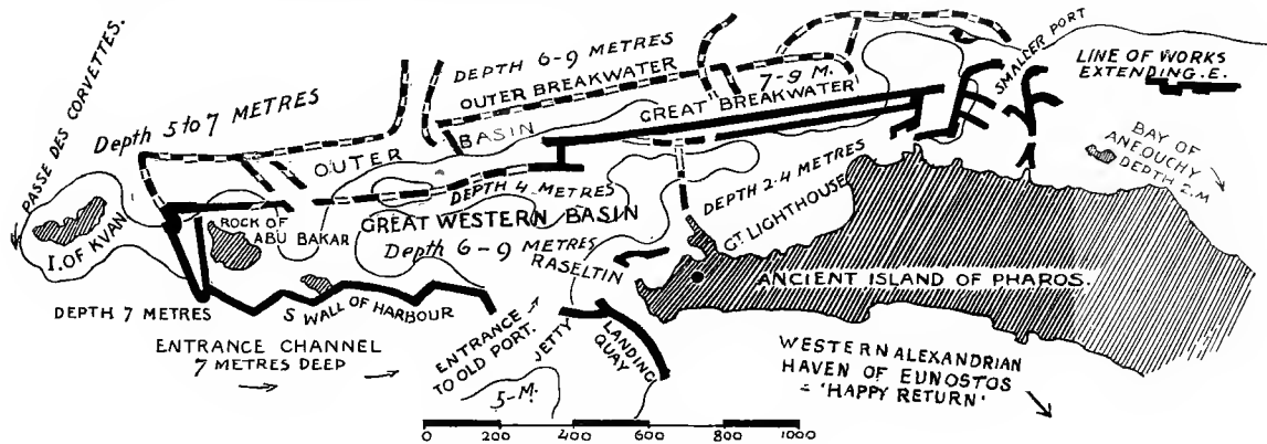
FIG. 221. SKETCH-PLAN OF PRE-HELLENIC PORT OF PHAROS.
