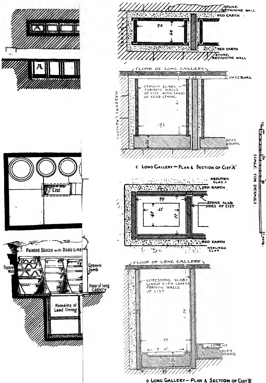
FIG. 325. A, B, C D CISTSELLES' AND THEIR LATER CONVERSION INTO SUPERFICIAL VATS.
