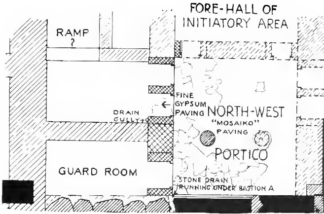
FIG. 162. PLAN OF NORTH-WEST PORTICO.
