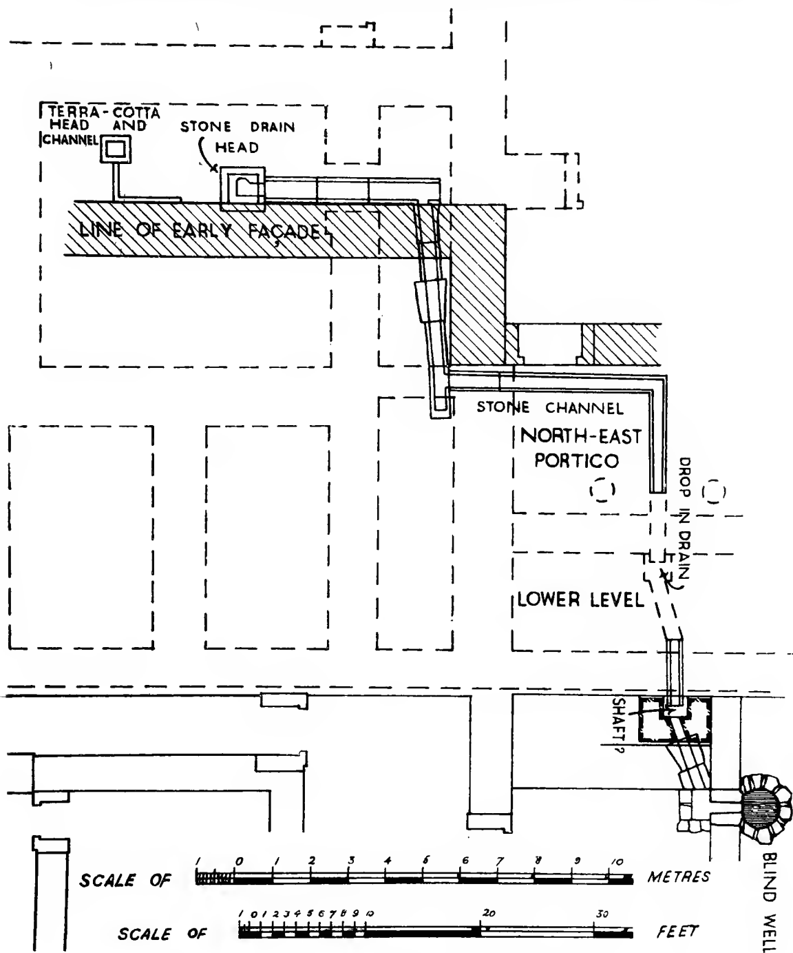
FIG. 276. PLAN OF DRAINAGE SYSTEM OF EARLY EAST HALL (M. M. III).
