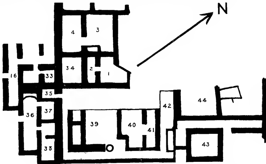
FIG. 39. PLAN OF E. M. II BUILDINGS AT VASILIKÈ (SEAGER): HOUSE ON THE HILL TOP.
