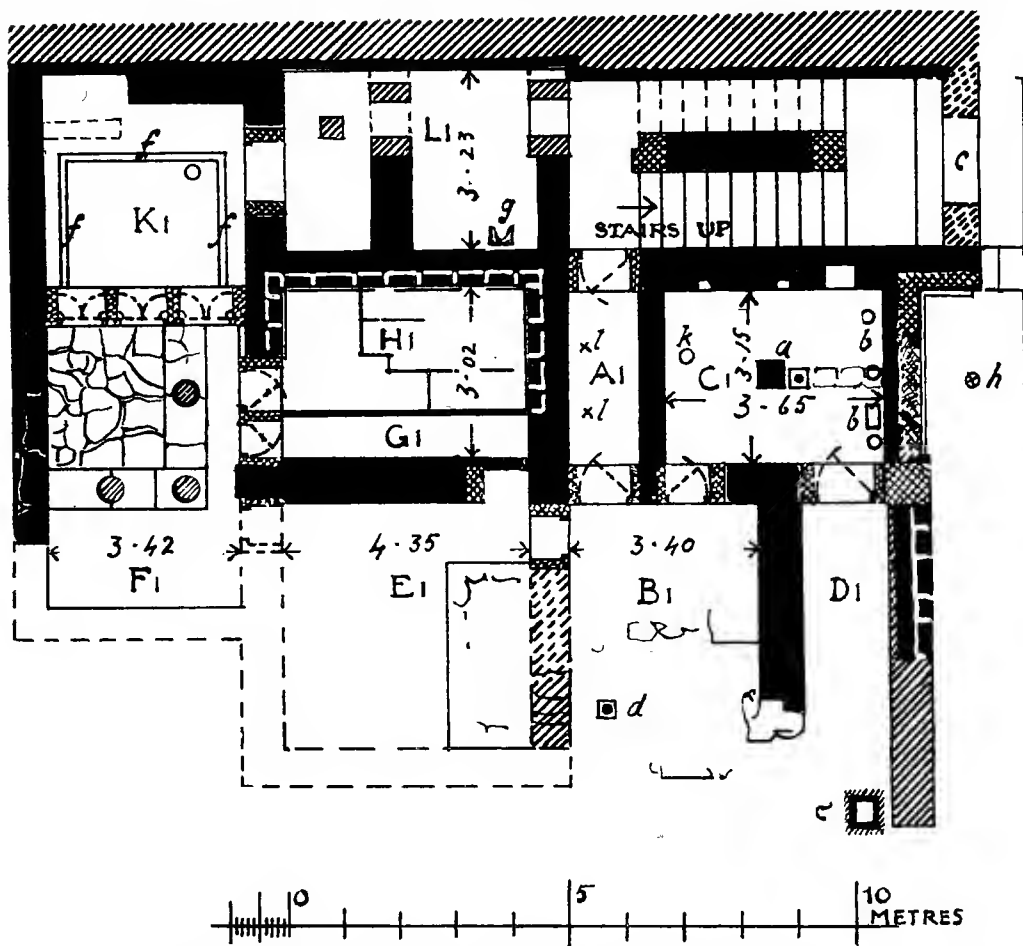
FIG. 306. PLAN OF SOUTH-EAST HOUSE. F 1. EARLY PERISTYLE WITH COLUMN BASES OF POLYCHROME MATERIALS: H 1. APPARENTLY EARLIER LIGHT-WELL WITH FINE ASHLAR MASONRY, LATER ROOFED OVER: K 1. SMALL MEGARON ( f, f, f , RAISED DAIS): L 1. INNER ROOM USED AS SHRINE IN REOCCUPATION PERIOD ( g , 'SACRAL HORNS' L. M. III b ): A 1. PASSAGE ( l, l , LILY AND OLIVE FRESCOS): C 1. PILLAR ROOM ( a , PILLAR: b, b , STANDS FOR RITUAL VESSELS: h , 'SACRAL KNOT' OF IVORY: k , COLUMNAR LAMP): D 1. MAGAZINE OPENING OFF CRYPT ( d , PLASTER STAND).
