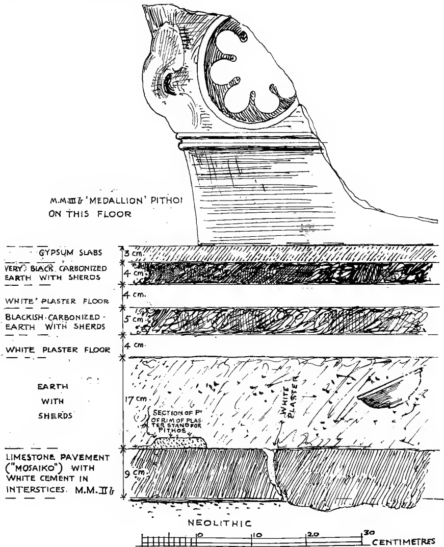
FIG. 233. SECTION BENEATH M. M. III b PAVEMENT OF MAGAZINE OF 'MEDALLION' PITHOI.
