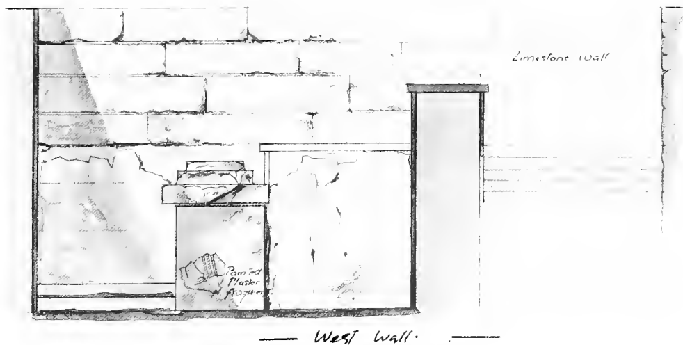
FIG. 294. SECTIONS OF NORTHERN LUSTRAL BASIN, LOOKING EAST (A) AND WEST (B).
