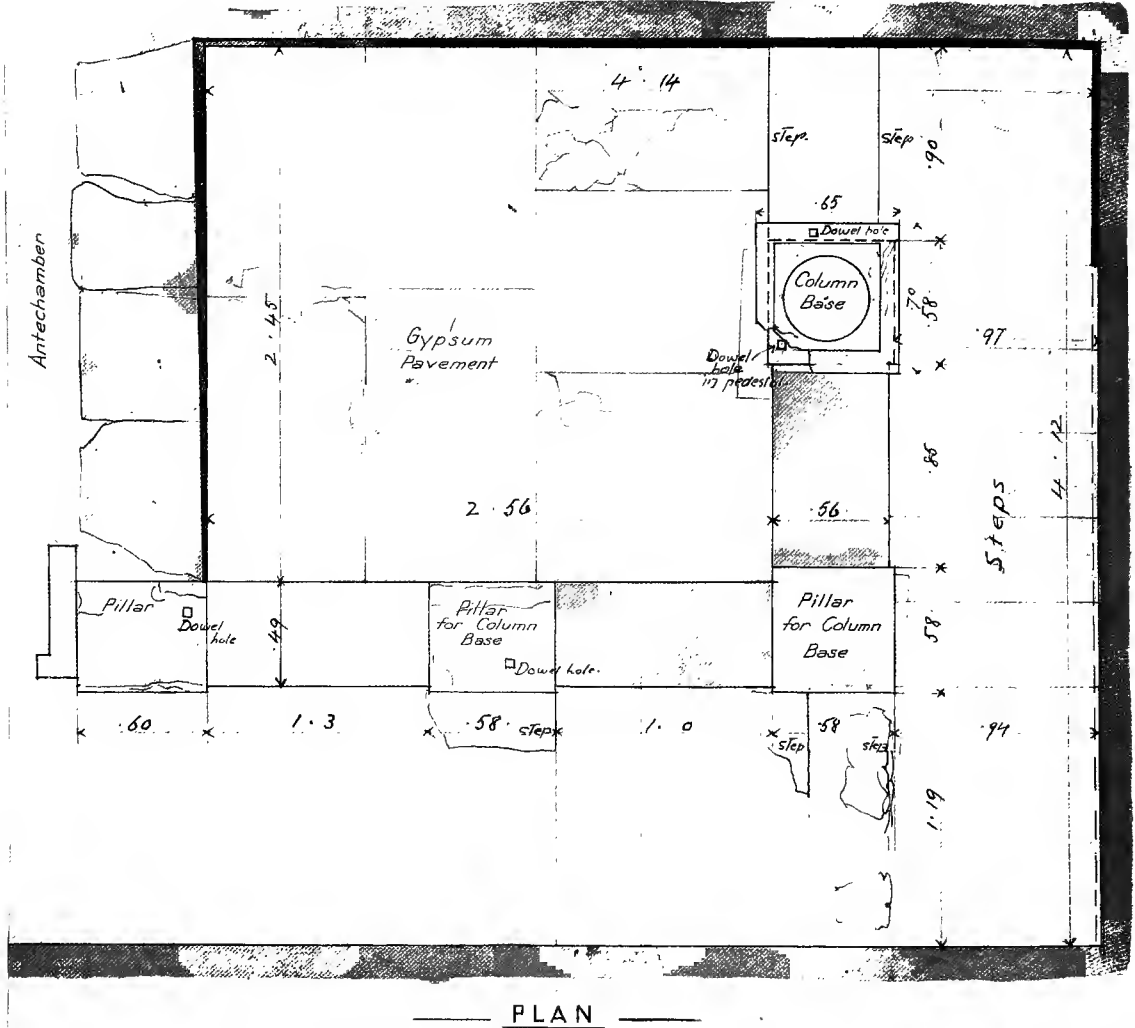
FIG. 293. PLAN OF LUSTRAL BASIN.
