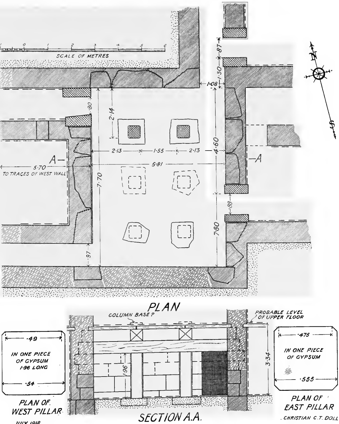
FIG. 290. PLAN AND RESTORED SECTION OF NORTH PILLAR CRYPT.
