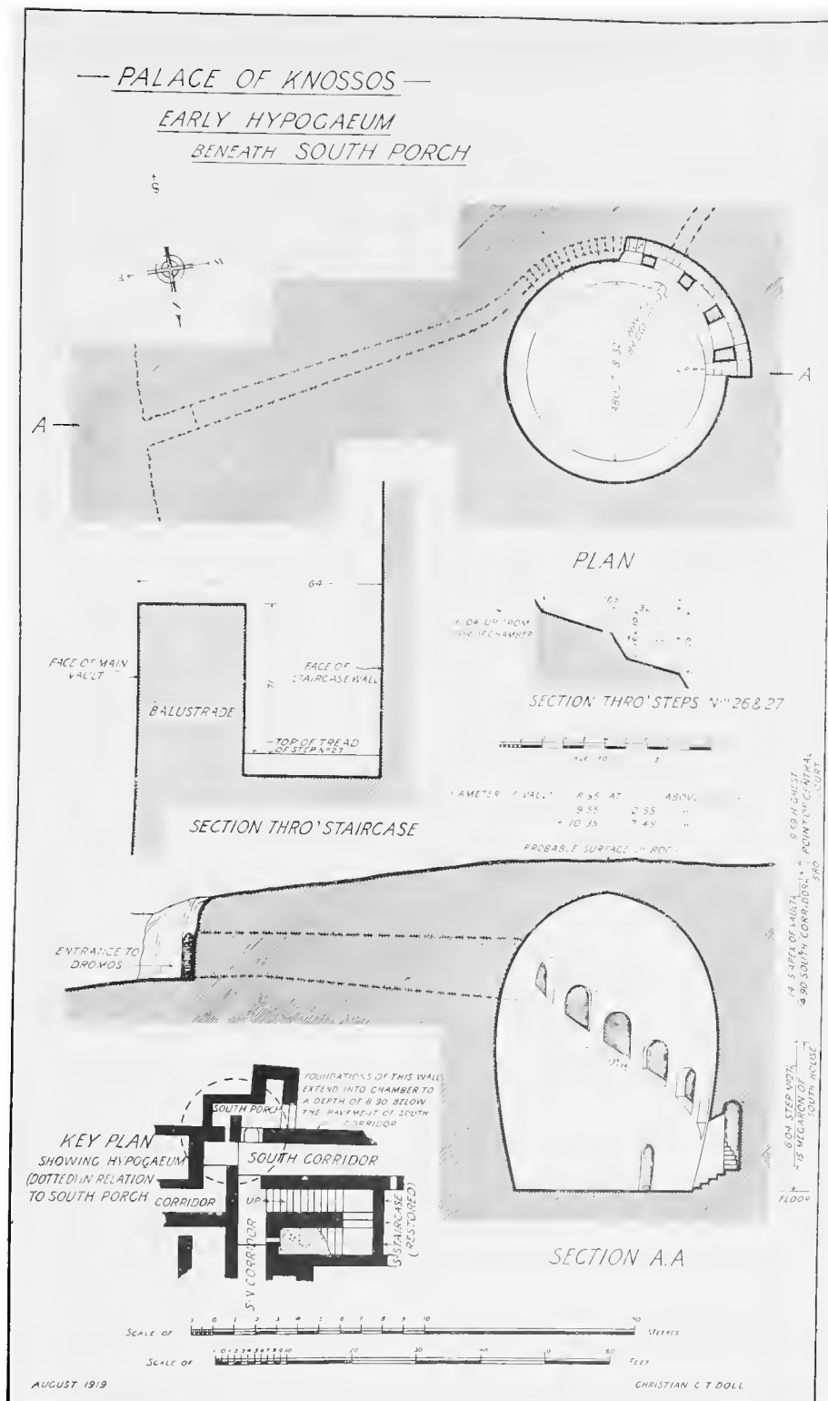
FIG. 74. PLAN AND SECTIONS OF EARLY HYPOGAEUM BENEATH SOUTH PORCH OF PALACE, KNOSSOS; PROBABLY SUBTERRANEAN SOUTHERN ENTRANCE OF EARLIER BUILDING.
