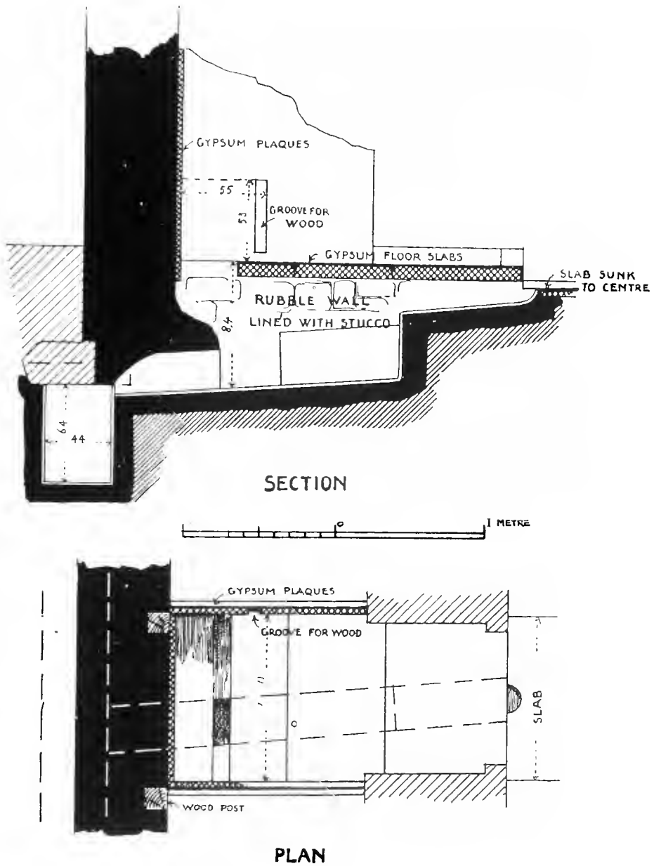
FIG. 172. PLAN AND SECTION OF LATRINE. (THEODORE FYFE.)
