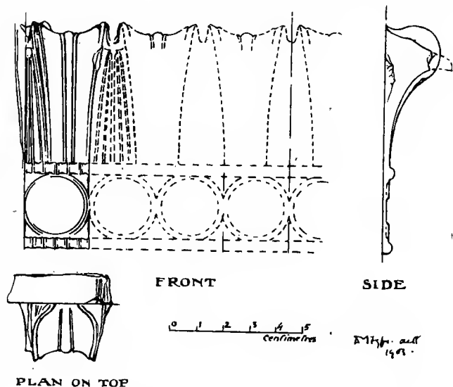
FIG. 350. DEVELOPMENT OF BRACKET BASED ON SECTION GIVEN BY MOULD, FIG. 349, a .
