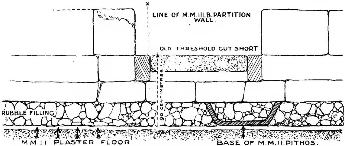
FIG. 262. FRONT VIEW OF N. WALL OF N.E. ROOM SHOWING ALTERED DOOR OPENING AND UNDERLYING M. M. II FLOOR.
