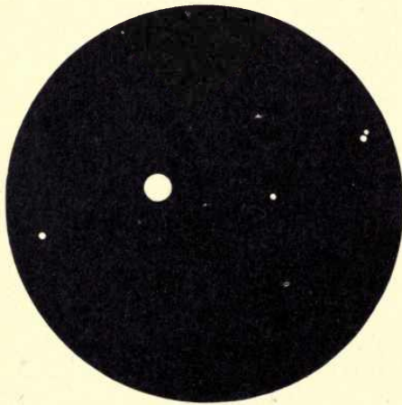
PROCYON AND ITS NEIGHBORS.
