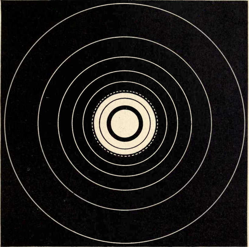
POLAR VIEW OF SATURN'S SYSTEM.
