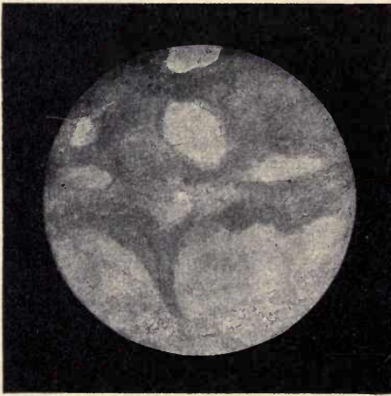
MARS SEEN WITH A FIVE-INCH TELESCOPE.
