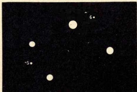
THE TRAPEZIUM WITH THE FIFTH AND SIXTH STARS.
