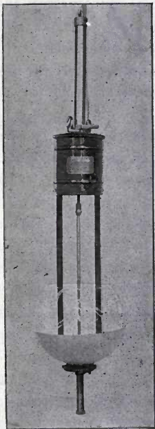
FIG. 25.—SINGLE CARBON ARC LAMP.
