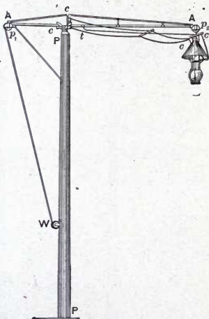
FIG. 63.—MAST-ARM SUPPORT. LAMP RAISED.
