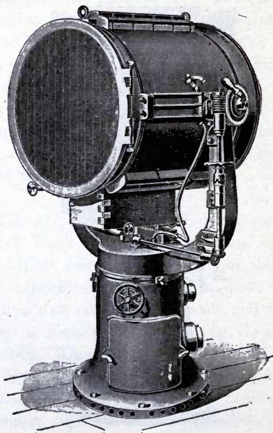
FIG. 112.—THIRTY-INCH PROJECTOR.
