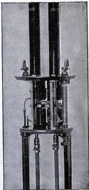
FIG. 34.—MECHANISM OF A SERIES DOUBLE-CARBON ARC LAMP.
