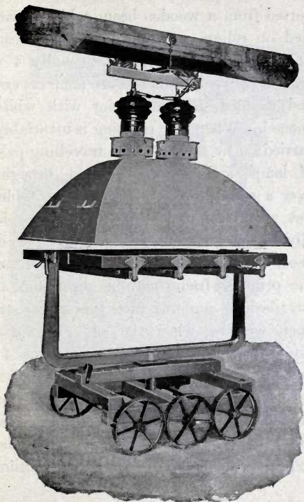
FIG. 169.—EQUIPMENT FOR ELECTRIC BLUE-PRINTING.
