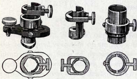
FIG. 137.—CARBON HOLDERS.
