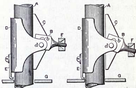
FIG. 19.—CLUTCH IN A SERIES ARC LAMP.
