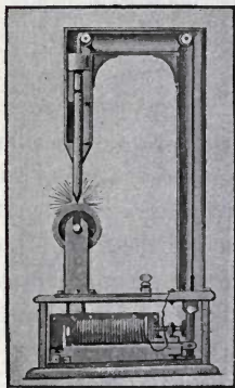
FIG. 28.—HARRISON'S LAMP.
