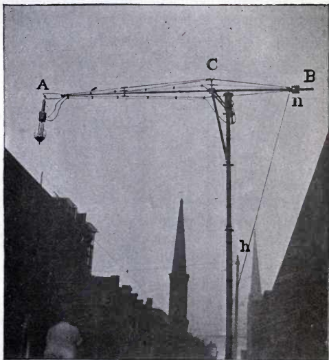
FIG. 65.—ARC LAMP MAST ARM.
