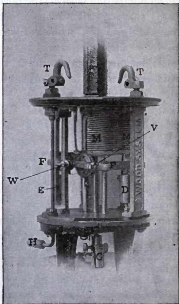
FIG. 86 —ALTERNATING-CURRENT LAMP MECHANISM.
