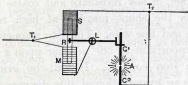
FIG. 13.—DIAGRAM OF EARLY SIEMEN'S REGULATOR.
