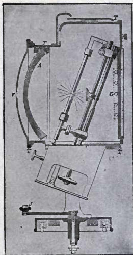
FIG. 121.—MANGIN'S PROJECTOR.
