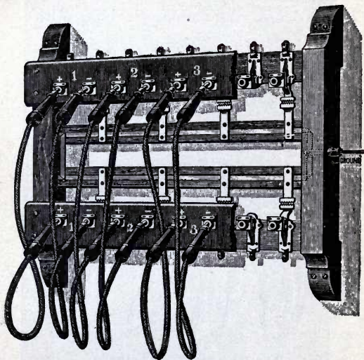
FIG. 155.—SWITCHBOARD WITH FACE REMOVED.
