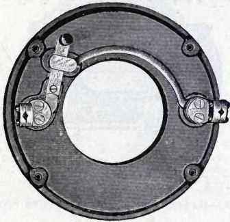
FIG. 68.—CIRCULAR LAMP HANGER.
