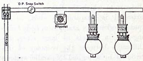
FIG. 38.—INCANDESCENT CIRCUIT, WITH SHORT LAMPS.
