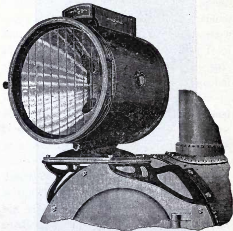
FIG. 123.—LOCOMOTIVE ARC HEADLIGHT.
