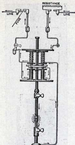
FIG. 40.—CONNECTIONS OF CONSTANT-POTENTIAL ARC LAMP.
