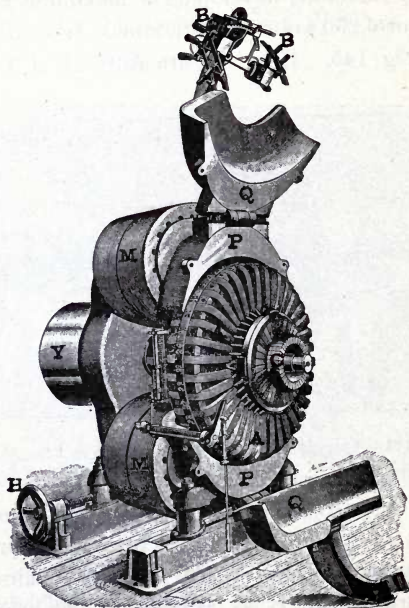
FIG. 147.—ARC-LIGHT GENERATOR.
