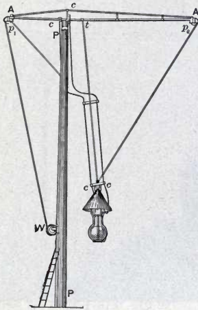
FIG. 64.—MAST-ARM SUPPORT. LAMP LOWERED.
