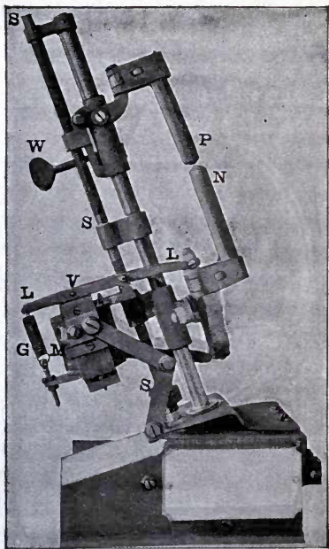
FIG. 108.—AUTOMATIC FOCUSING LAMP.
