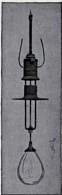
FIG. 97.—ALTERNATING-CURRENT CONSTANT-POTENTIAL LAMP WITH GLOBE INVERTED.
