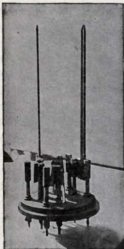
FIG. 2.—JABLOCHKOFF CANDLE HOLDER.
