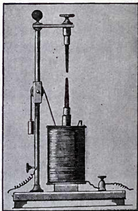
FIG. 10.—ARCHEREAU'S REGULATOR.
