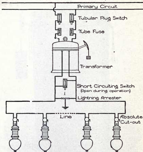
FIG. 167.—CONNECTIONS OF CONSTANT-CURRENT ARC-LIGHTING TRANSFORMER.
