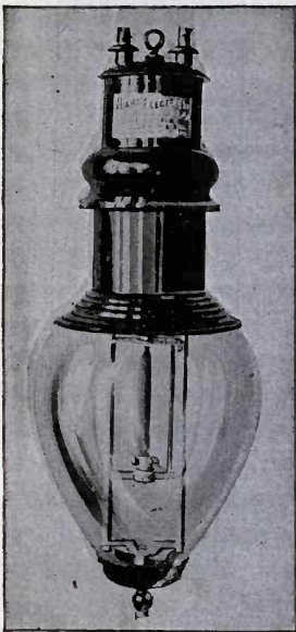
FIG. 98.—ALTERNATING-CURRENT ARC LAMP.
