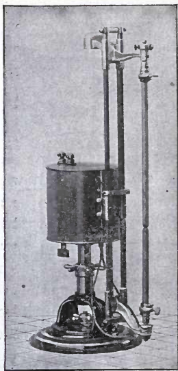
FIG. 109.—VERTICAL AUTOMATIC FOCUSING LAMP.
