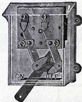
FIG. 71.—CUT-OUT SWITCH.
