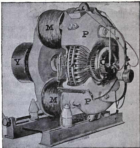
FIG. 148.—ARC-LIGHT GENERATOR.
