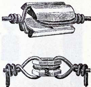
FIG. 58.—CIRCUIT-LOOP INSULATORS.
