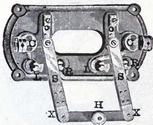
FIG. 69.—HANGER BOARD AND INSULATING SWITCH.
