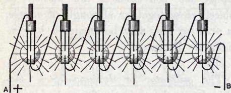
FIG. 8.—SERIES CONNECTION OF ARC LAMPS.
