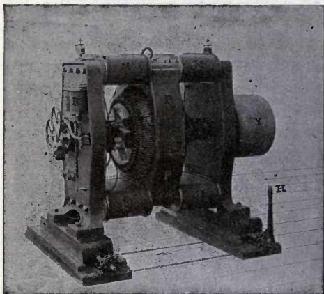
FIG. 140.—BIPOLAR GRAMME-RING ARC-LIGHT GENERATOR.
