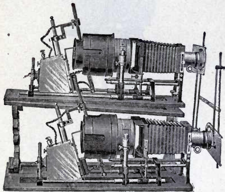
FIG. 125.—ELECTRIC STEREOPTICON.
