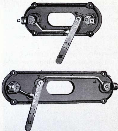
FIG. 67.—LAMP HANGERS.
