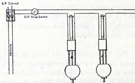
FIG. 39.—INCANDESCENT CIRCUIT WITH TWO ARC LAMPS.
