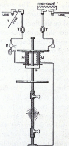
FIG. 87.—CONNECTIONS OF LAMP MECHANISM SHOWN IN FIG. 86.
