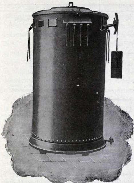
FIG. 166.—CONSTANT-CURRENT ARC-LIGHTING TRANSFORMER COMPLETE.
