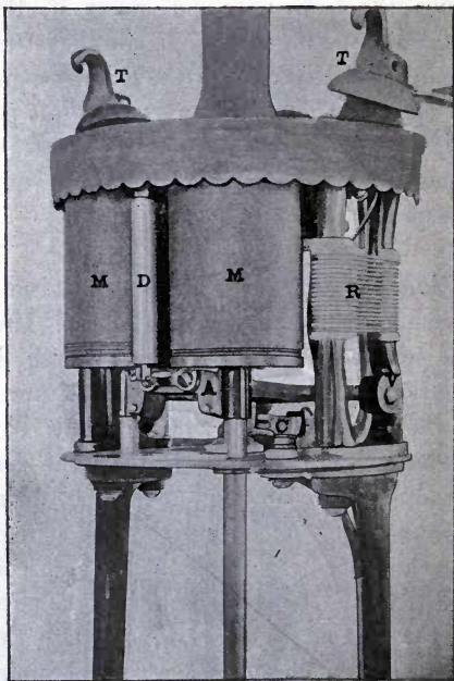
FIG. 18.—FORM OF ARC LAMP MECHANISM.
