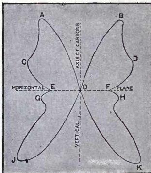
FIG. 103.—DISTRIBUTION OF LIGHT FROM AN ALTERNATING-CURRENT ARC.
