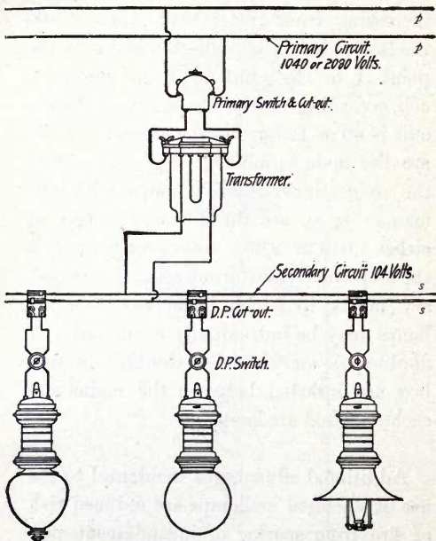
FIG. 162.—DIAGRAM OF CONNECTIONS.
