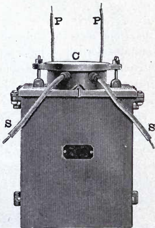
FIG. 95.—OIL INSULATED TRANSFORMER.
