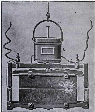
FIG. 26.—THE WALLACE ALL-NIGHT LAMP.
