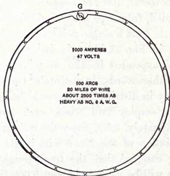
FIG. 37.—PARALLEL ARC LIGHT DISTRIBUTION.
