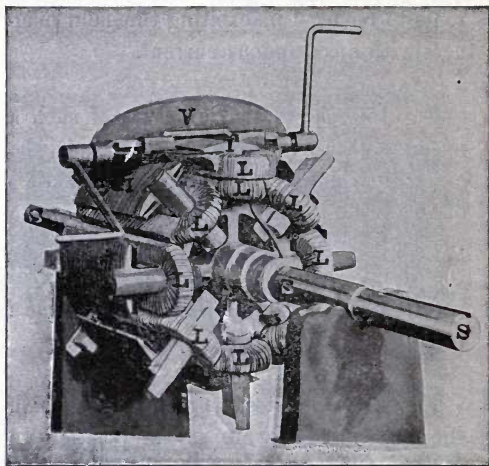
FIG. 151.—ARRANGEMENT OF ARMATURE COILS.
