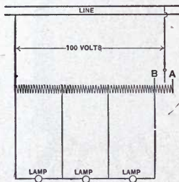
FIG. 92.—CONNECTIONS OF ECONOMY COIL.
