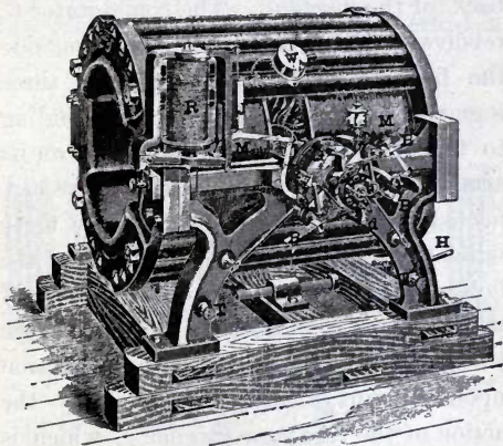
FIG. 142.—BIPOLAR CONTINUOUS-CURRENT ARC-LIGHT GENERATOR.
