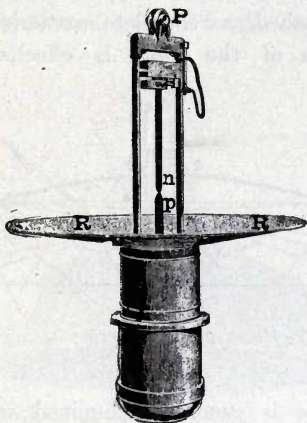
FIG. 104.—ARC LAMP FOR DIFFUSED LIGHTING.
