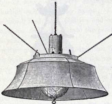
FIG. 106.—VIEW OF ARC DIFFUSER OF FIG. 105.
