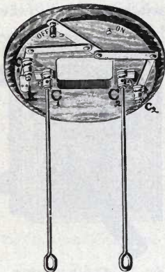
FIG. 70.—CIRCULAR INSULATING HANGER BOARD AND SWITCH.
