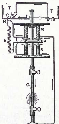
FIG. 16.—DIAGRAMMATIC CONNECTION OF LAMP SHOWN IN FIG. 15.
