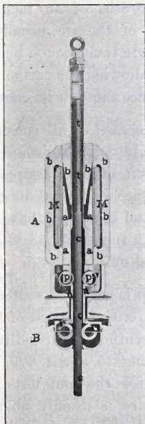
FIG. 47.—SECTION OF MECHANISM SHOWN IN FIGS. 44, 45 AND 46.
