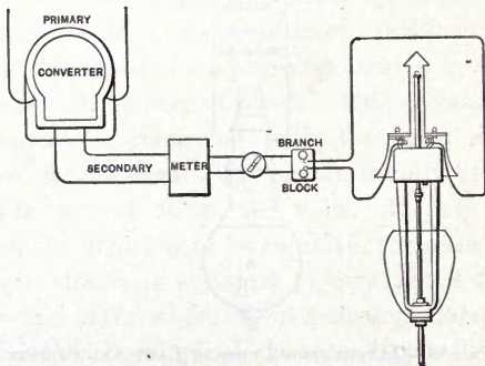
FIG. 89.—ALTERNATING-CURRENT ARC LAMP AND CIRCUIT CONNECTIONS.
