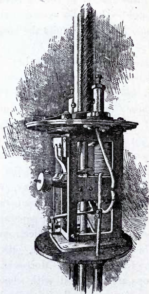
FIG. 24.—MECHANISM OF ARC LAMP.
