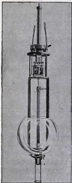
FIG. 29.—ALL-NIGHT ELLIPTICAL CARBON LAMP.
