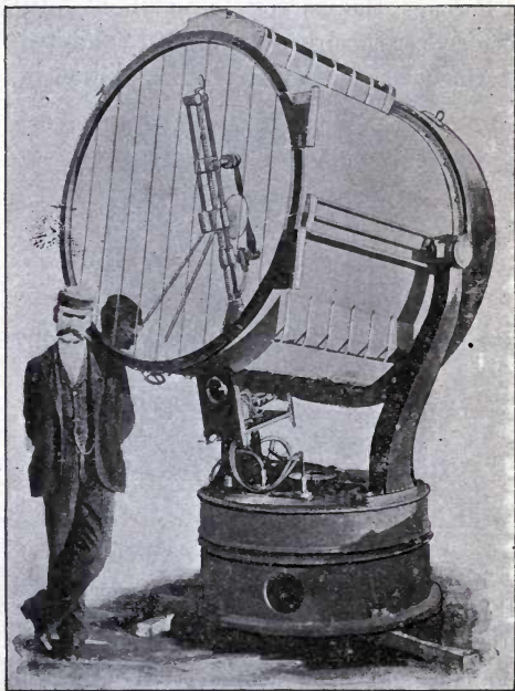
FIG. 120.—SIXTY-INCH PROJECTOR.
