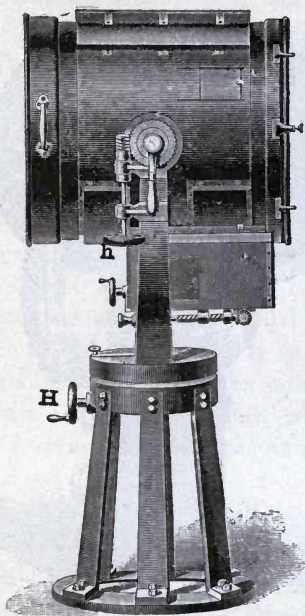
FIG. 111.—SEARCH LAMP WITH SLOW MOTION SCREW.
