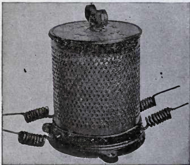
FIG. 93.—ECONOMY COIL AND SWITCH.
