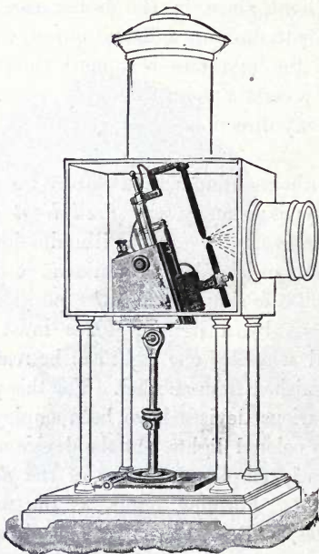
FIG. 124.—LANTERN PROJECTION ARC LAMP.
