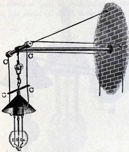
FIG. 49.—OUTRIGGER SUSPENSION.
