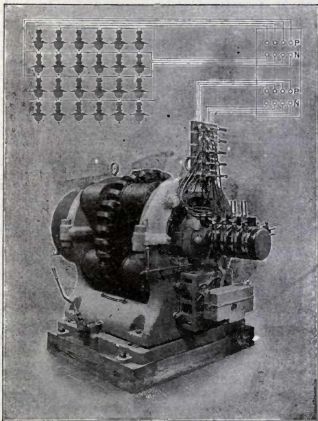
FIG. 168.—MULTI-CIRCUIT, 4 CIRCUITS, SHOWING THE GENERATOR, SWITCHBOARD, AND THE DIFFERENT LAMP CIRCUITS.
