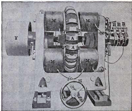
FIG. 145.—ARC-LIGHT GENERATOR.
