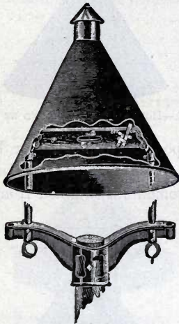
FIG. 76.—HANGER BOARD IN POSITION UNDER HOOD.
