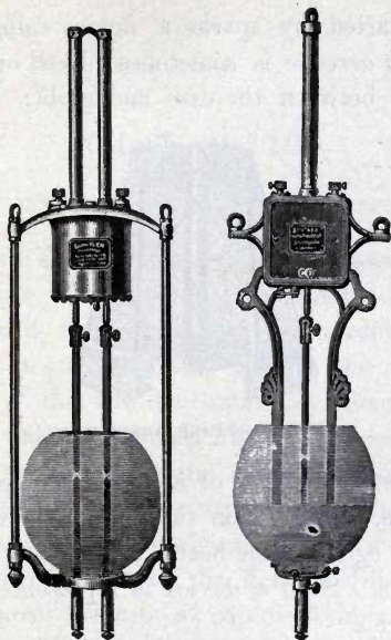
FIG. 84.—GLOBE INSIDE AND OUTSIDE OF LAMP FRAME.
