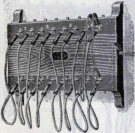
FIG. 154.—ARC SWITCHBOARD.
