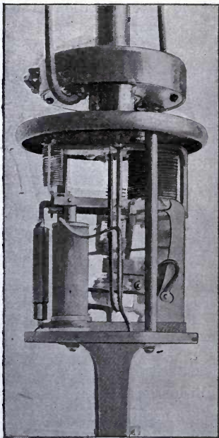
FIG. 23.—INTERIOR MECHANISM OF ARC LAMP.
