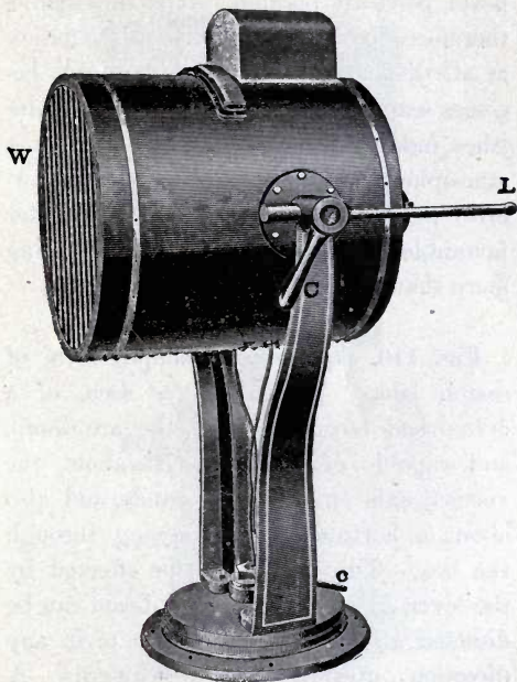
FIG. 110.—SIMPLE FORM OF SEARCH LAMP.
