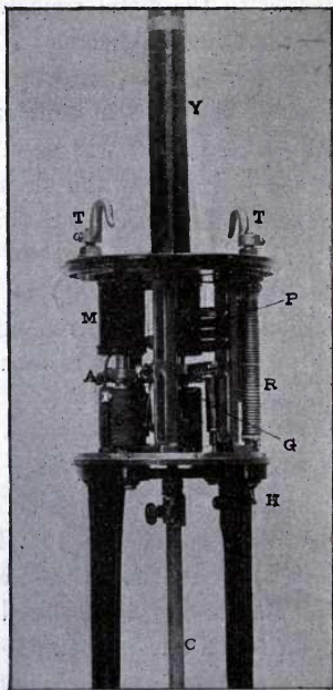
FIG. 17.—FORM OF ARC LAMP MECHANISM.
