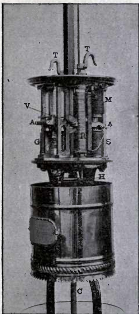
FIG. 15.—FORM OF ARC LAMP MECHANISM.
