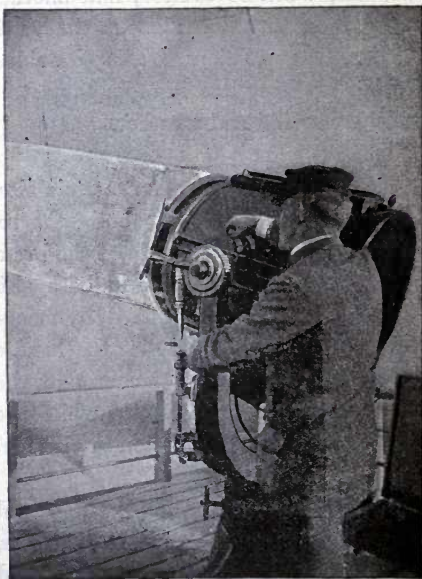
FIG. 113.—THIRTY-INCH PROJECTOR ON MOUNT WASHINGTON.
