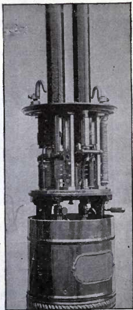
FIG. 33.—MECHANISM OF A SERIES DOUBLE-CARBON ARC LAMP.
