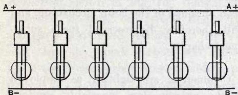
FIG. 9.—PARALLEL OR MULTIPLE CONNECTION OF ARC LAMPS.
