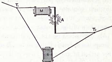
FIG. 12.—DIAGRAM OF SHUNTS AND SERIES MAGNETS.
