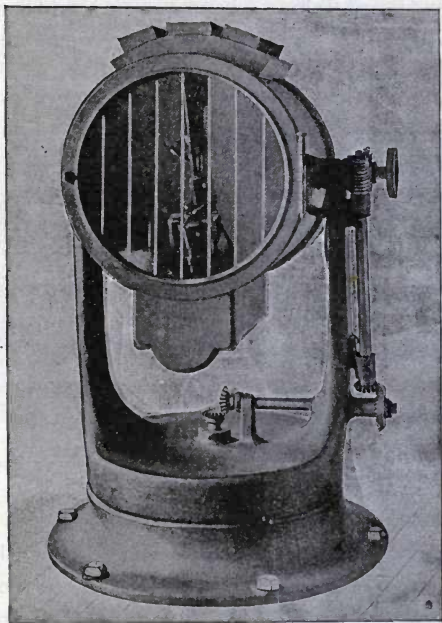
FIG. 115.—MARINE SEARCH-LIGHT PROJECTOR, WITH GEAR CONTROL.
