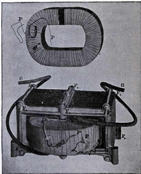
FIG. 94.—TRANSFORMER, DETAILS OF CONSTRUCTION.
