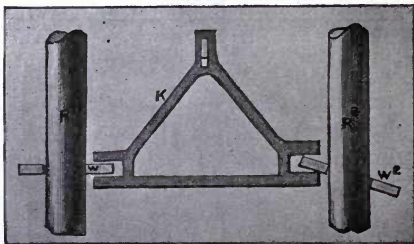
FIG. 31.—BRUSH WASHER OR RING CLAMP.
