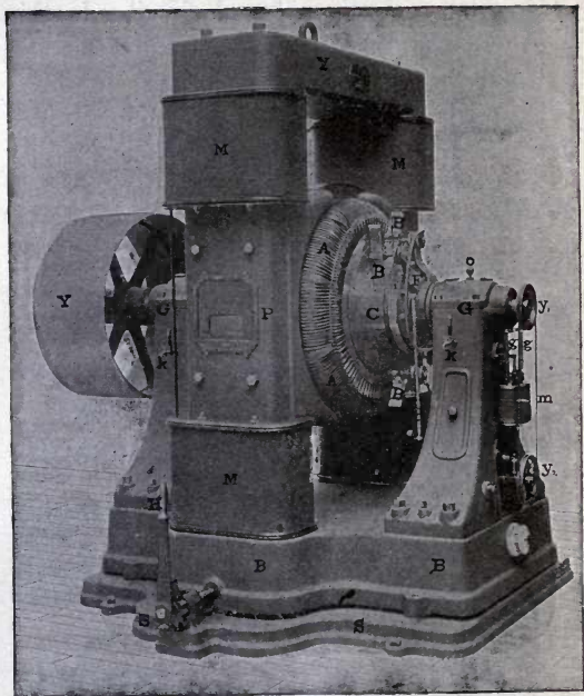
FIG. 138.—BIPOLAR CONTINUOUS-CURRENT GENERATOR.
