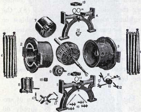
FIG. 143.—PARTS OF GENERATOR SHOWN IN FIG. 142.
