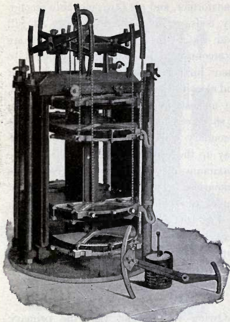
FIG. 165.—MECHANISM OF CONSTANT-CURRENT ARC-LIGHTING TRANSFORMER.
