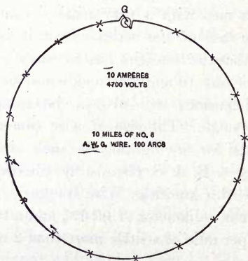
FIG. 36.—SERIES ARC LIGHT DISTRIBUTION.
