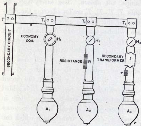
FIG. 90.—VARIOUS METHODS OF CONNECTING ALTERNATING-CURRENT ARC LAMPS.
