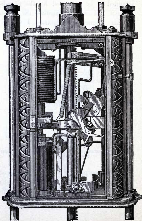
FIG. 23.—INTERIOR MECHANISM OF A SERIES ARC LAMP.
