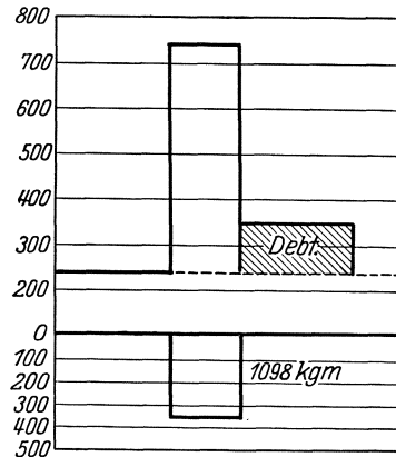
Abb. 23. Normal hell (Dr. E.). Requirement: 2028 ccm O 2 . Debt: 565 ccm = 27,8%.
