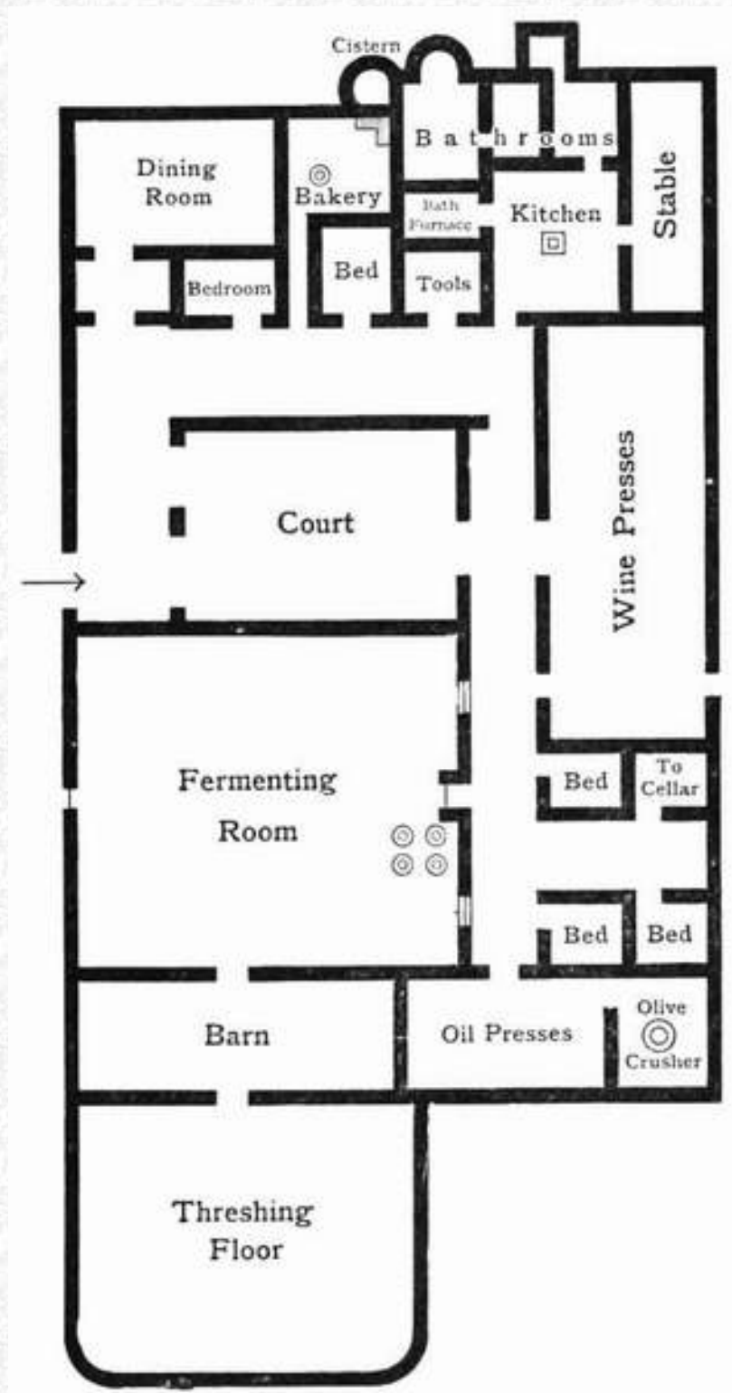
Plan Of A Campanian Farmhouse - This was in the most prosperous and comfortable district of Italy.
