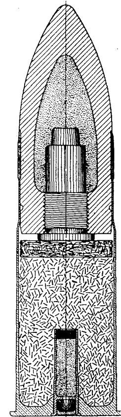
FIG. 76.—37-mm. ammunition with 20-grain primer.
