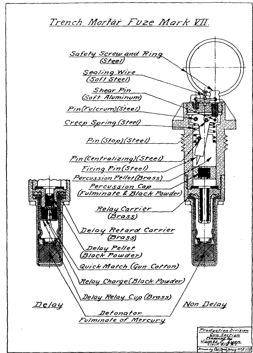
FIG. 105.—Detail of trench mortar fuze, Mark VII.
