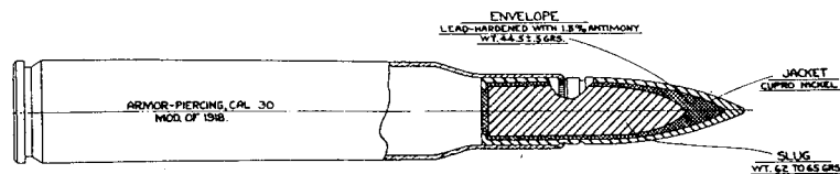
FIG. 157.—Armor-piercing cartridge, caliber .30, model 1918.
