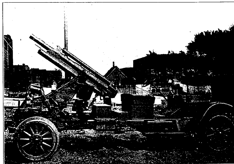
FIG. 40.—75-mm. field gun, model 1916, on A. A. truck mount, model 1917, 2\frac{1}{2} -ton White truck.
