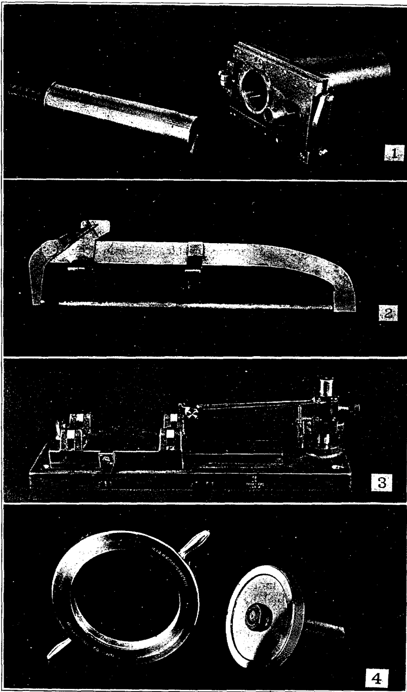
FIG. 210.—Miscellaneous types of gauges. 1. Chamber gauge and check plug for 75-mm. gun. 2. O. O. gauge for base thickness of shell. 3. Frankford Arsenal concentricity gauge. 4. Screw thread gauges, ring and plug type.
