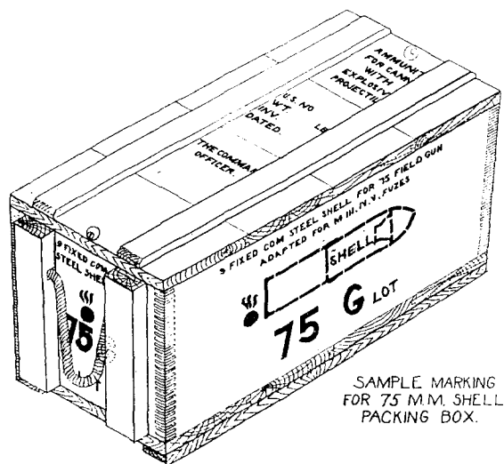
FIG. 82.—Packing case for 75-mm. shell.
