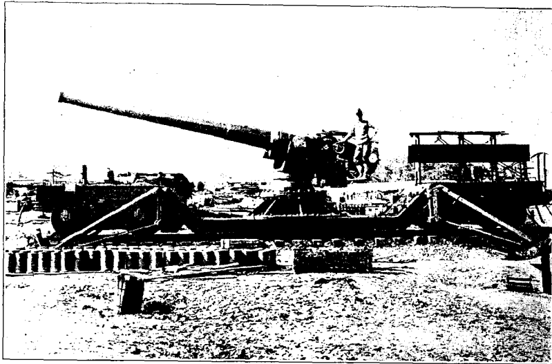
FIG. 30.—7-inch Navy railway mount, model of 1918.
