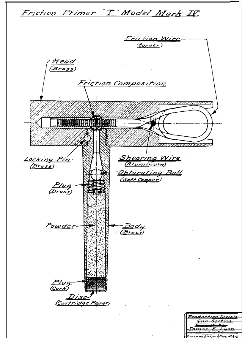
FIG. 78.—"T" model friction primer, Mark IV.
