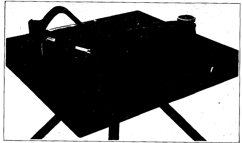
FIG. 143.—Plane table with clinometer and angle of site instrument.
