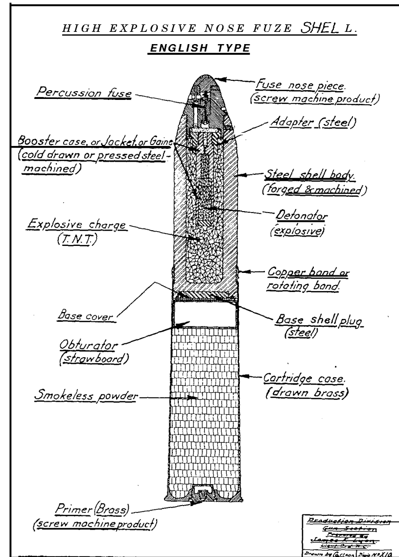
FIG. 51.—High-explosive nose fuze shell, English type.
