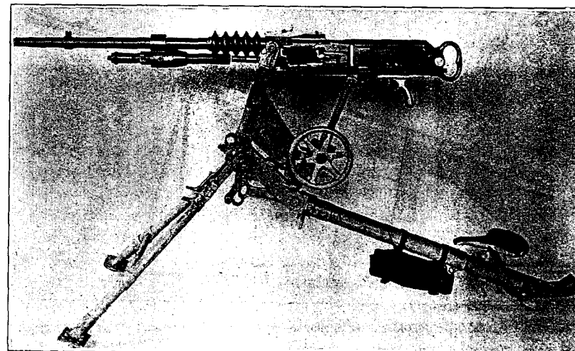
FIG. 138.—Hotchkiss machine gun and tripod.
