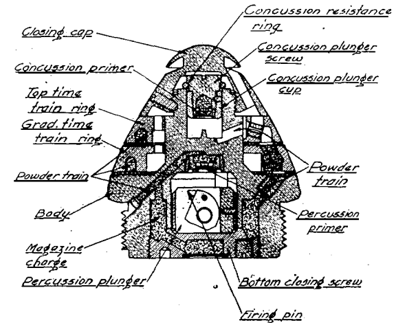
FIG. 67.—Combination time and percussion fuze—before arming.
