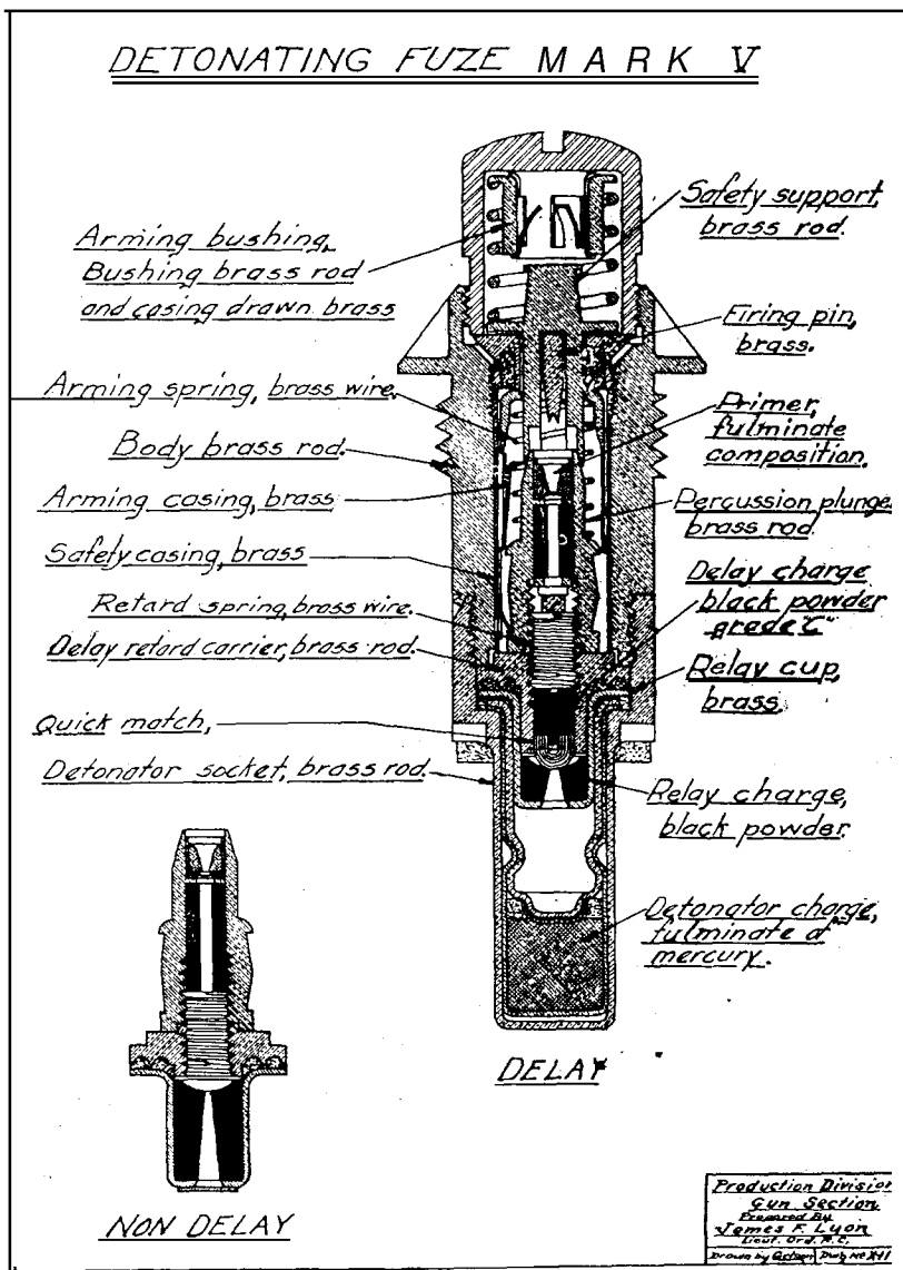
FIG. 61.—Point detonating fuze, Mark V.
