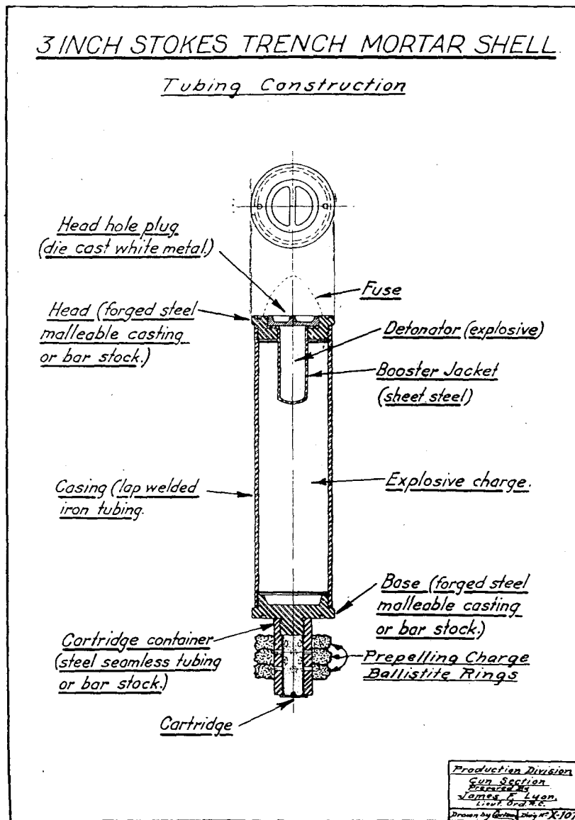
Fig. 97.—Detail of 3-inch Stokes trench mortar shell.
