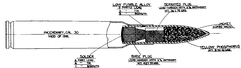
FIG. 158.—Incendiary cartridge, caliber .30, model 1918.
