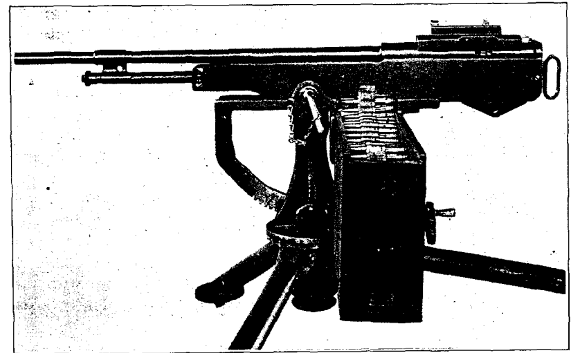
FIG. 134.—Marlin aircraft machine gun mounted on Colt tripod.
