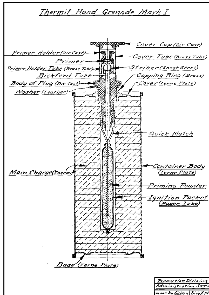
FIG. 90.—Sectional view of thermit hand grenade, Mark I.
