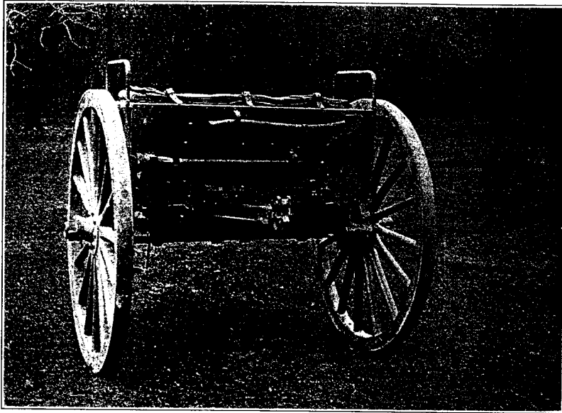
FIG. 10.—3-inch gun caisson, model of 1916, rear view.
