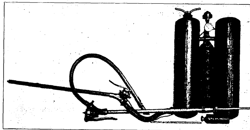
FIG. 129.—Experimental knapsack flame projector.
