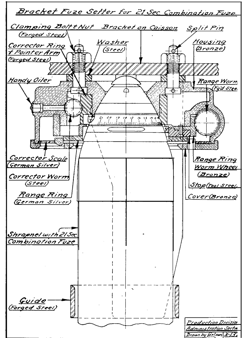
FIG. 80.—Bracket fuze setter, Model 1916.
