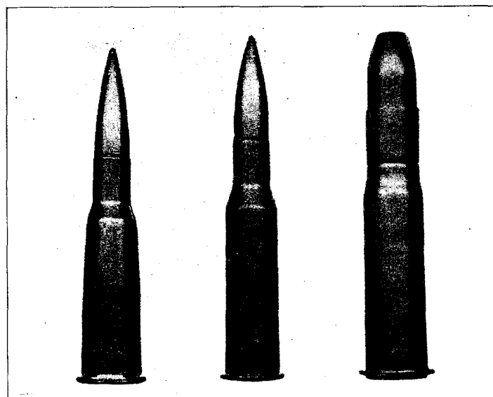
8-mm. Lebel cartridge 7.62-mm Russian ammunition 11-mm. incendiary cartridge
