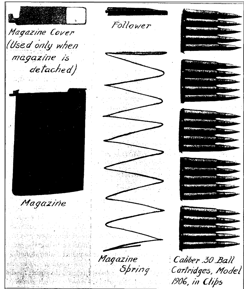
FIG. 150.—U. S. rifle, model 1903, extension magazine with parts and clips.
