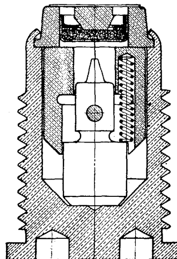
FIG. 63.—Base percussion fuze minor caliber, Mark I, Baldwin type.
