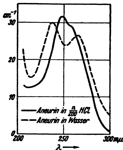
Fig. 12. Absorption Spectrum of Vitamin B 1 (from GREWE 424)).
