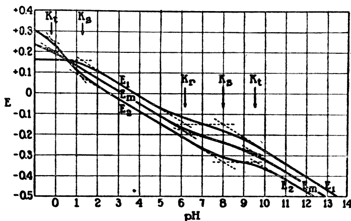
Fig. 11. Plot of the normal potentials of riboflavin against ph. E_1 , normal potential of mixture of the fully reduced and of the semiquinoid form; E_s , normal potential of mixture of the semiquinoid and the fully oxidized form; E_m , normal potential of mixture of fully reduced and of fully oxidized form; K_t , dissociation constants of oxidized form, K_s , dissociation constants of reduced form (MICHAELIS, SCHUBERT and SMYTHE 822)).
