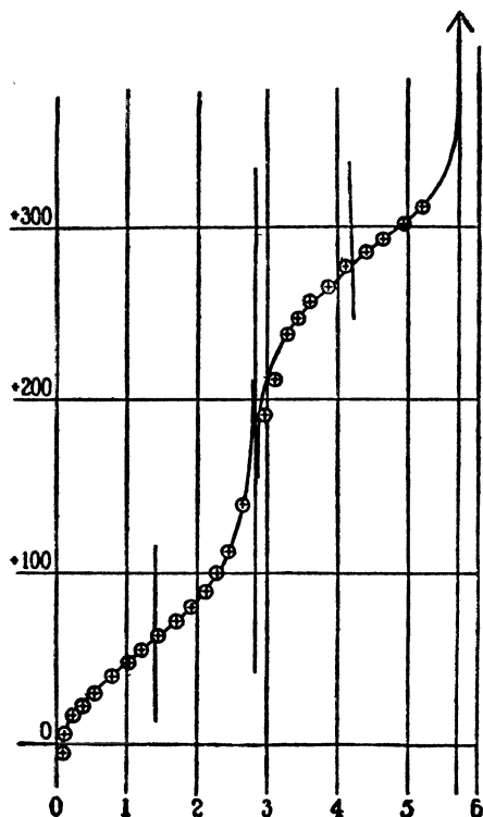
Fig. 1. Potentiometric oxidative titration curve of \alpha -hydroxyphenazine (MICHAELIS 805). The leuco-dye was titrated with benzoquinone as oxidizing agent at pH 1.00. Abscissa: benzoquinone added; Ordinate: potential as referred to the hydrogen electrode.
