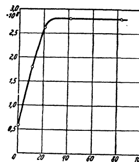
Fig. 6. Curve representing the changes in light absorption occurring upon adding varying amounts of globin to 1 mg. blood hemin dissolved in 200 cc. 0.1 M. neutral phosphate buffer. Abscissa: mg. globin in 200 cc. solution; Ordinate: Light absorption coefficient, \beta , at 405 m \mu . (From WARBURG and NEGELEIN 1275)).
