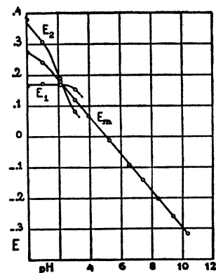
Fig. 15. E_o /ph-curve of Chlororaphine (ELEMA 234)).
