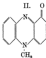
Pyocyanine (N-Methyl- \alpha -oxyphenazine)
