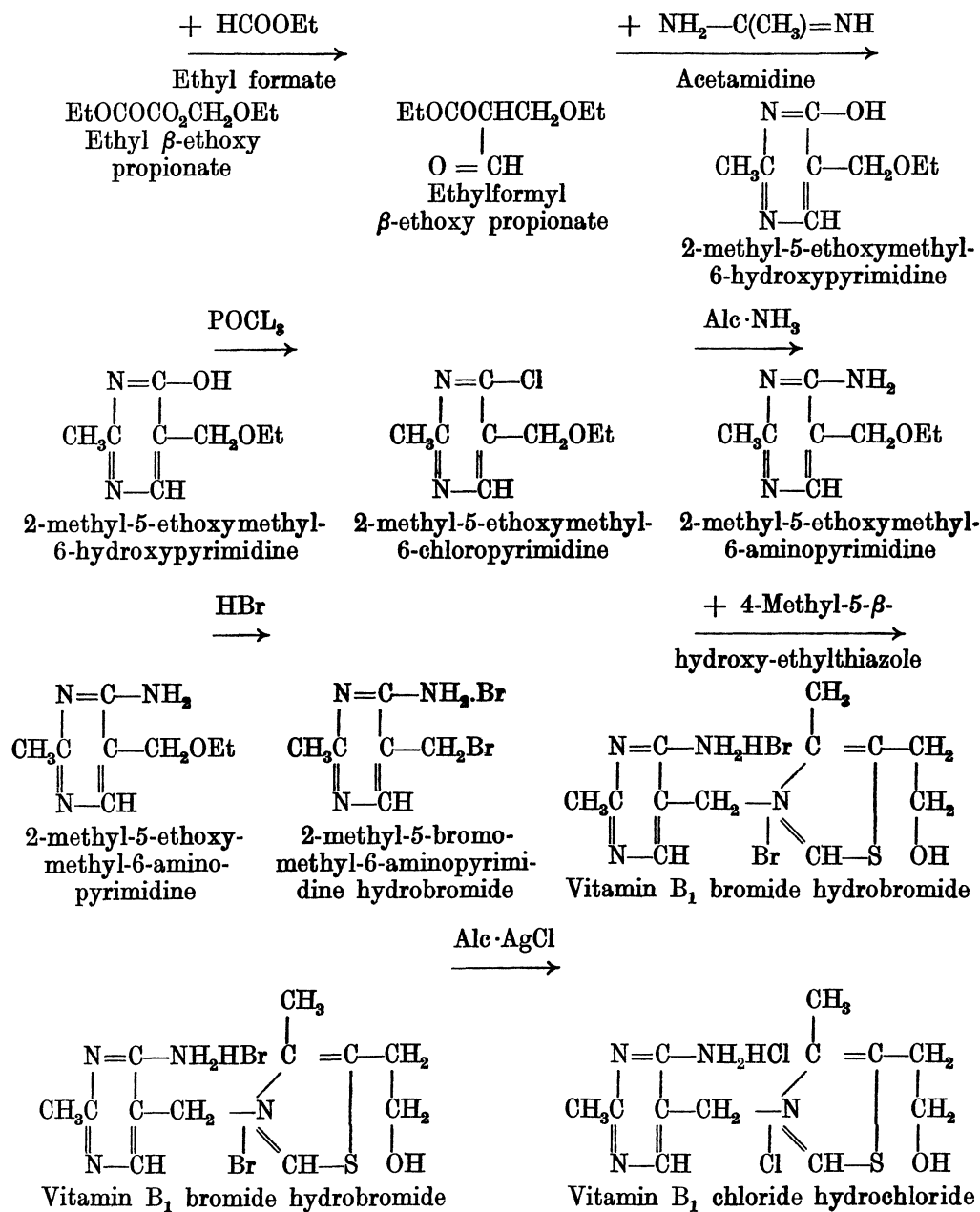
Synthesis of Vitamin B 1 by WILLIAMS.
