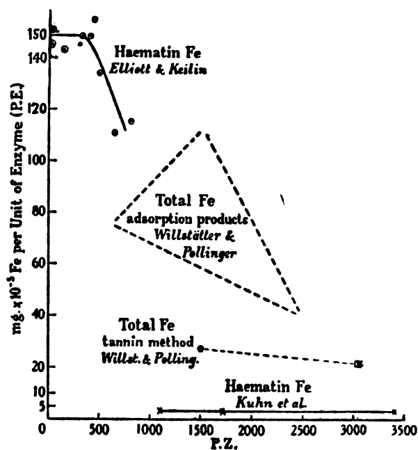
Fig. 7. Diagram showing the amounts of hematin-iron or of total iron per unit of peroxidase activity, in preparations of varying concentration. The total iron figures of WILLSTÄTTER and POLLINGER are scattered within the triangular area indicated in the diagram. (From ELLIOTT and KEILIN 247)).
