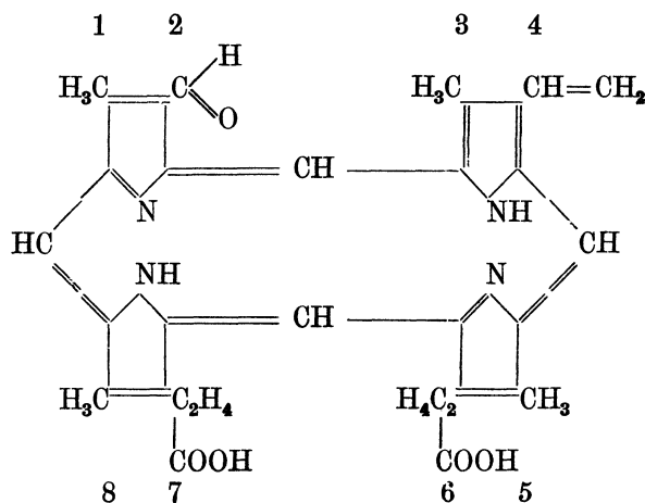
Spirographis Porphyrin (acc. to FISCHER and SEEMANN 343)).
