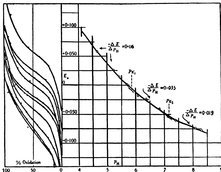
Fig. 16. Potentials of Toxoflavin (Acc. to STERN 1083).
