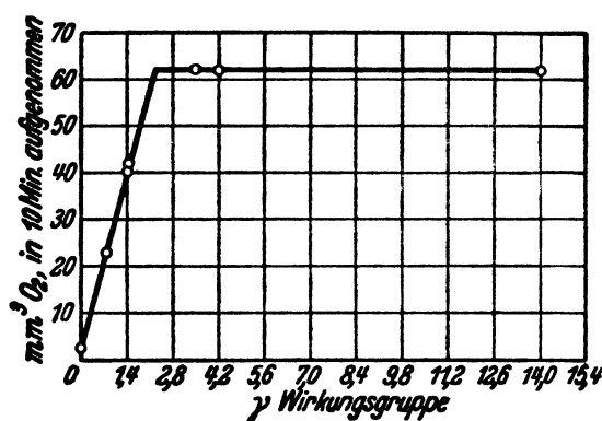
Fig. 9. Resynthesis of the yellow enzyme. Ordinate, catalytic activity in terms of O 2 -uptake of the test system; Abscissa, amount of flavin phosphate added to constant amount of carrier protein (THEORELL 1954)
