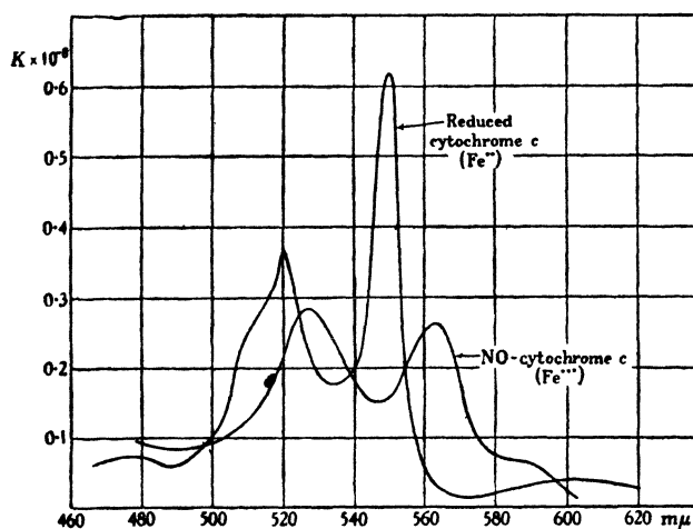
Fig. 5. Absorption Spectrum of NO-cytochrome complex as compared with that of reduced cytochrome. Ordinate, absorption coefficient per gram atom of cytochrome iron; abscissa, wave-length in millimicrons. (KEILIN and HARTREE 548a)).
