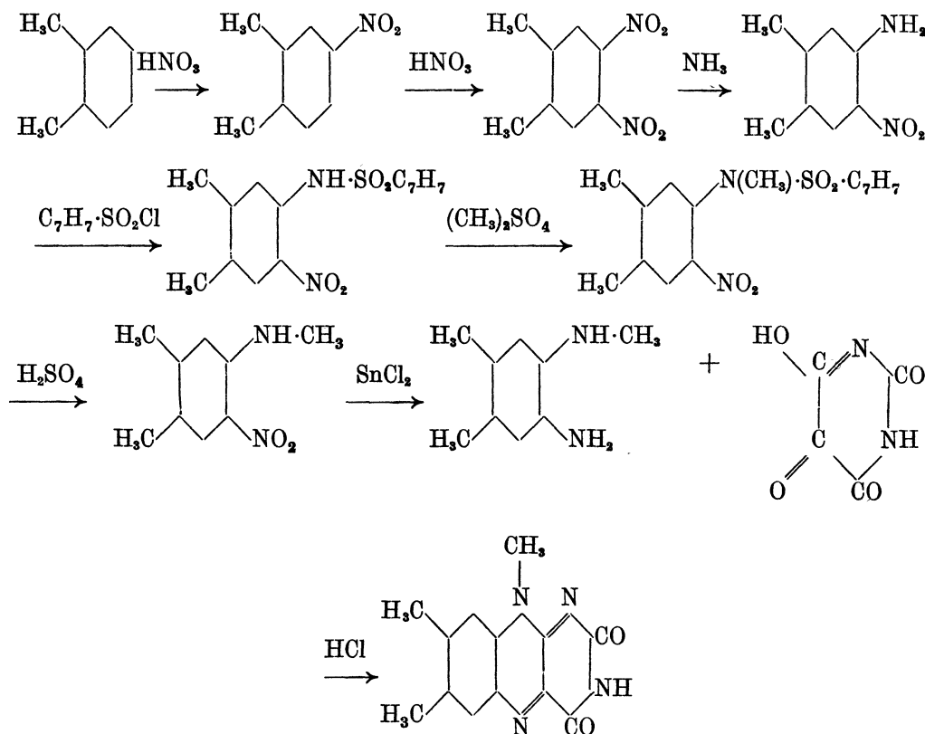
Synthesis of Lumilactoflavin according to KUHN.
