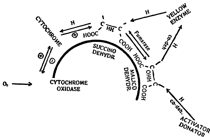
Fig. 17. Schema of Cell Respiration according to SZENT-GYÖRGYI 1125). The semicircle represents a granule of the muscle cell. The picture is somewhat simplified by not writing the three cytochromes in series.
