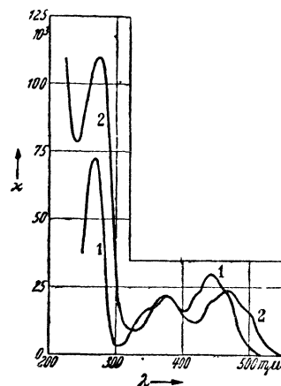
Fig. 10. Absorption Spectra of the Yellow Enzyme (2) and of Riboflavin (1) acc. to RUDY 1010).
