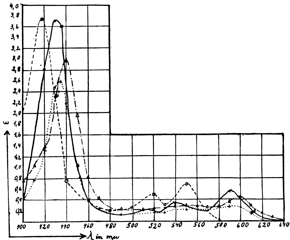
Fig. 3. Absorption Spectra of the Respiratory Enzyme Spirographishemin proteins and Cytochrome c in the Visible (400 to 640 \text{ m}\mu ). Abscissa: Wave-length; Ordinate: Absorption coefficient. Curves:
