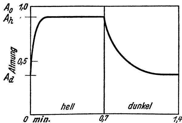
Fig. 2. Course of CO-inhibited respiration with intermittent illumination (WARBURG and NEGELEIN 1268).
