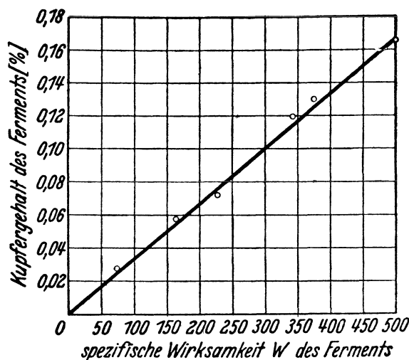
Fig. 8. Specific activity and copper content of potato polyphenol oxidase. (From KUBOWITZ 613). Abscissa, Specific activity; Ordinate, Copper content in %.
