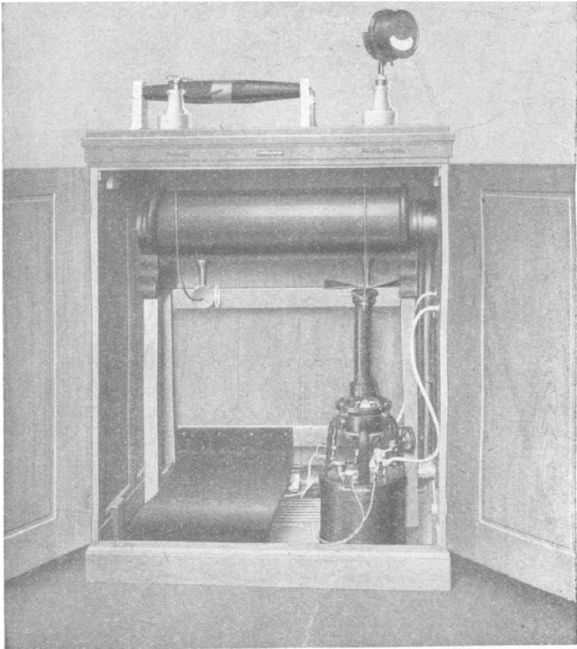
Coolidge-Instrumentarium.
