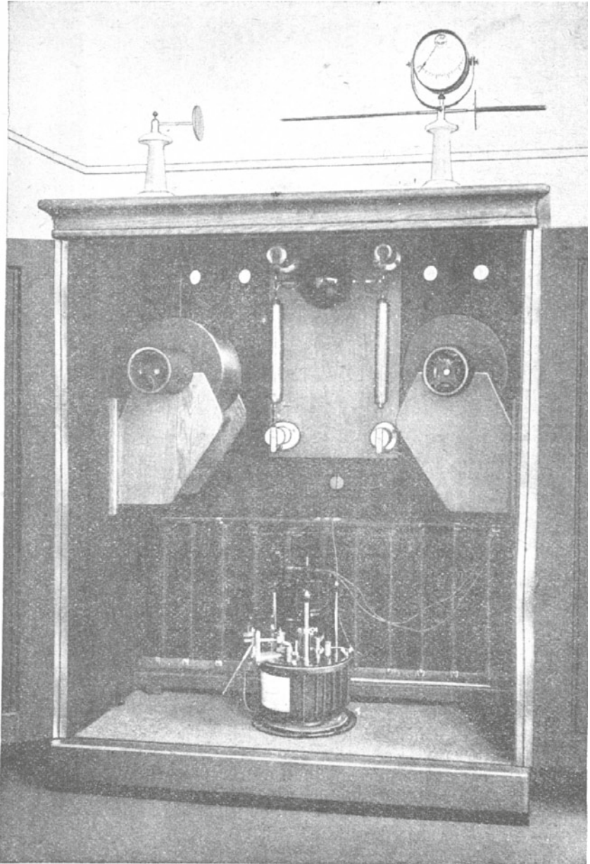
Symmetrie-Instrumentarium.
