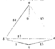
diuersilaterum; ... pyramidi abgd. ... 100. recto, lib. 7, 8-15; pag. 171. lib. 38 — pag. 172, lib. 41.
