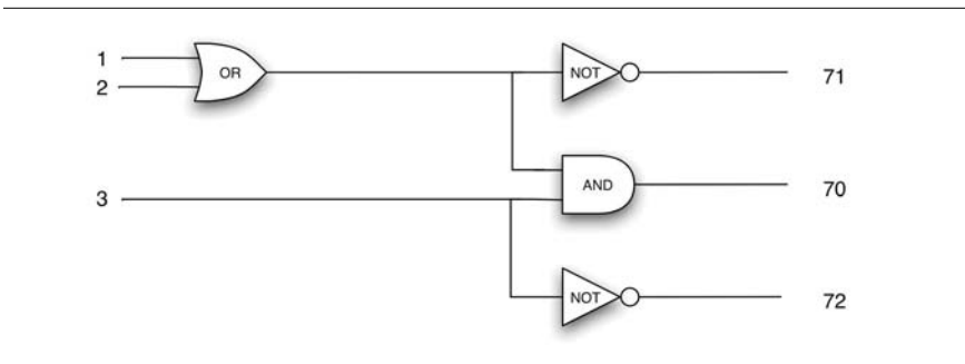
Figure 4.7 Logic diagram equivalent to Figure 4.6.
