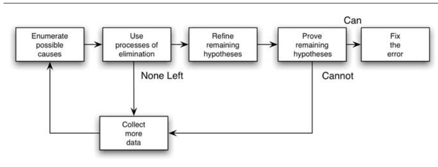
Figure 7.4 The deductive debugging process.
