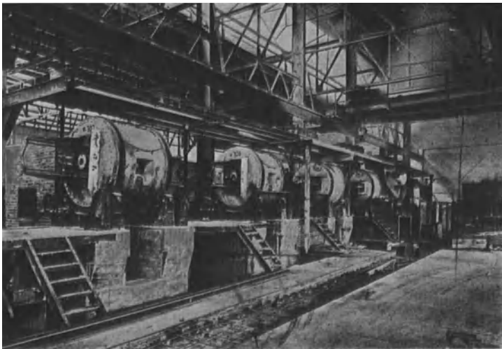
Abb. 5. Detroit-Öfen der Detroit-Brass-Company.
