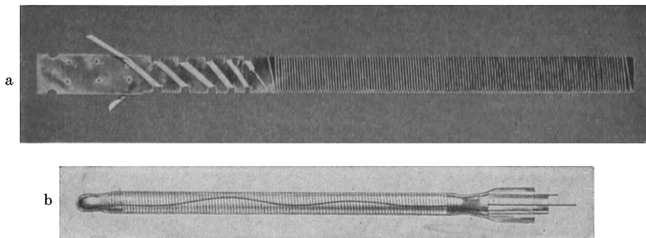
Abb. 29. Platin-Widerstands-Thermometer.
