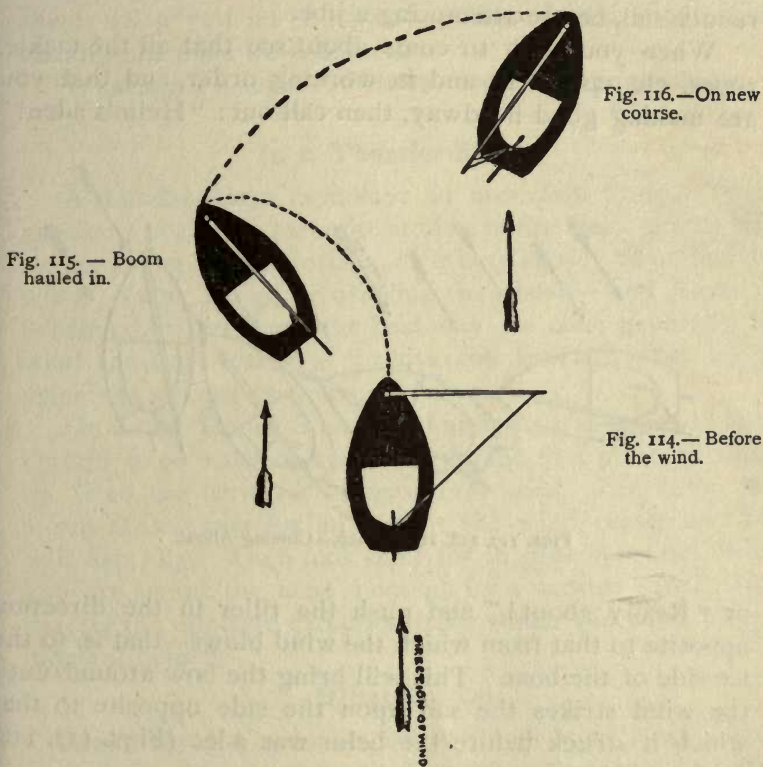
FIGS. 114, 115 and 116.—Jibing.
