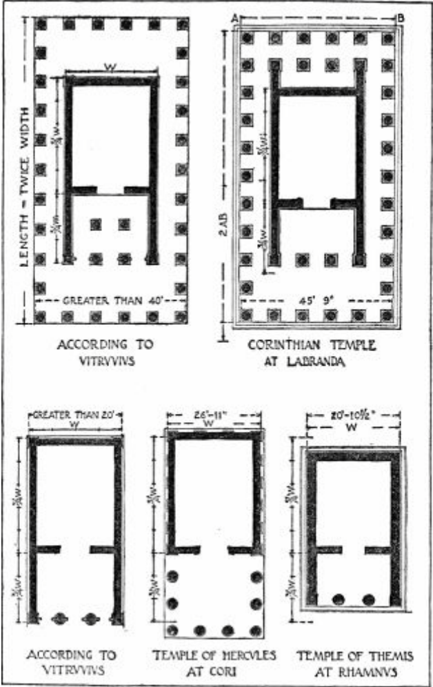
VITRUVIUS' TEMPLE PLAN COMPARED WITH ACTUAL EXAMPLES
