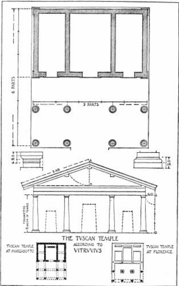
THE TUSCAN TEMPLE ACCORDING TO VITRUVIUS.
