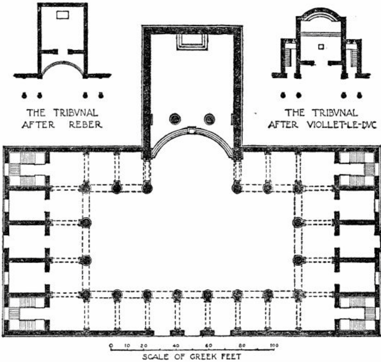
VITRUVIUS' BASILICA AT FANO
