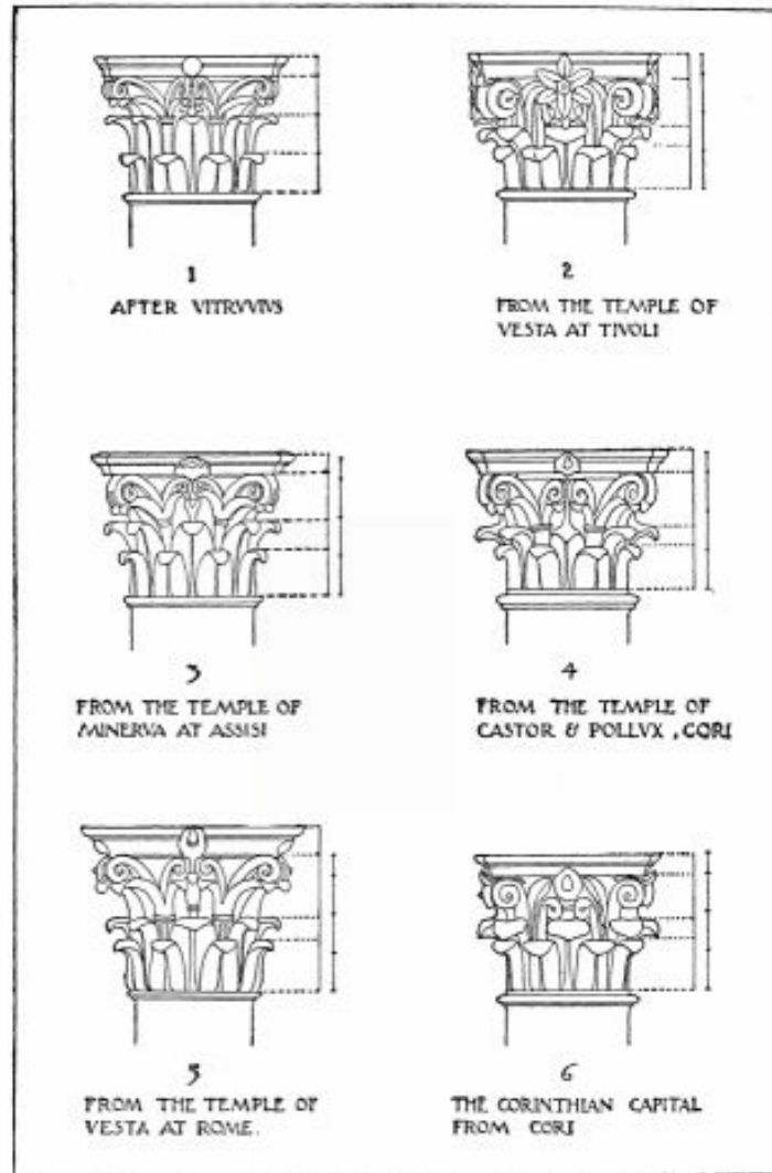
THE CORINTHIAN CAPITAL OF VITRUVIUS COMPARED WITH THE MONUMENTS
