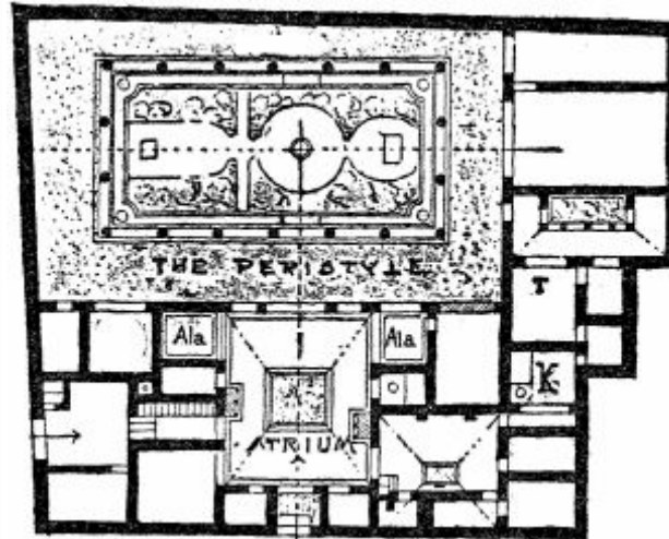
PLAN OF THE HOUSE OF THE VETTII, POMPEII
