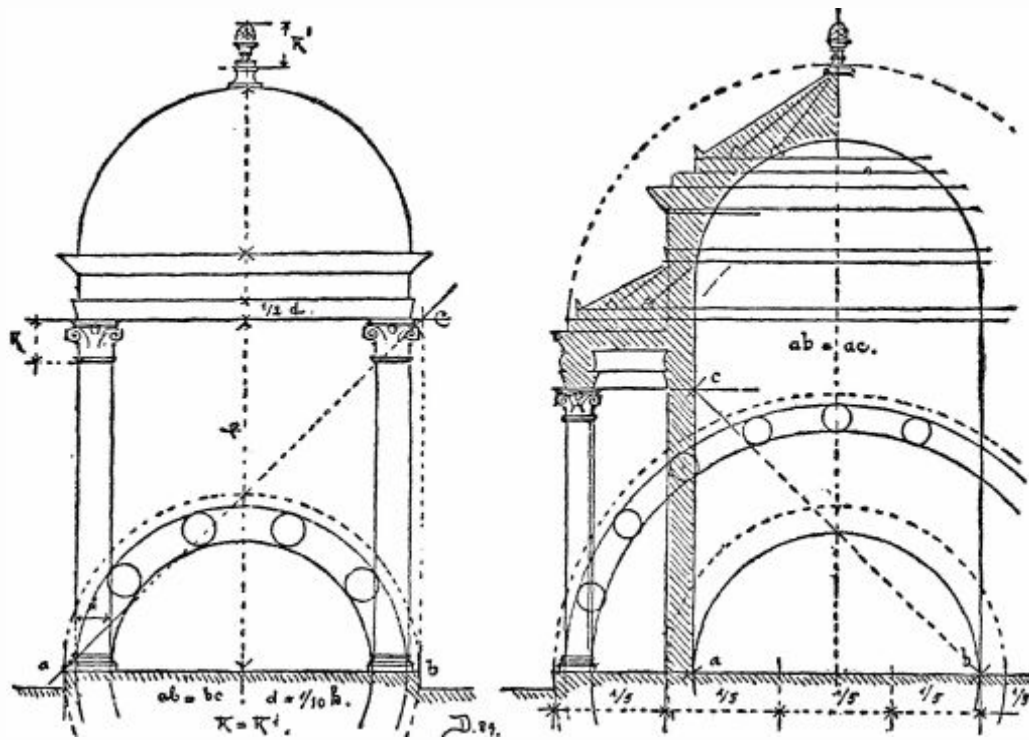
THE CIRCULAR TEMPLE ACCORDING TO VITRUVIUS
