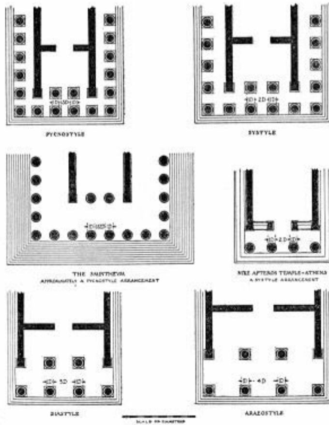
THE CLASSIFICATION OF TEMPLES ACCORDING TO INTERCOLUMNIATION
