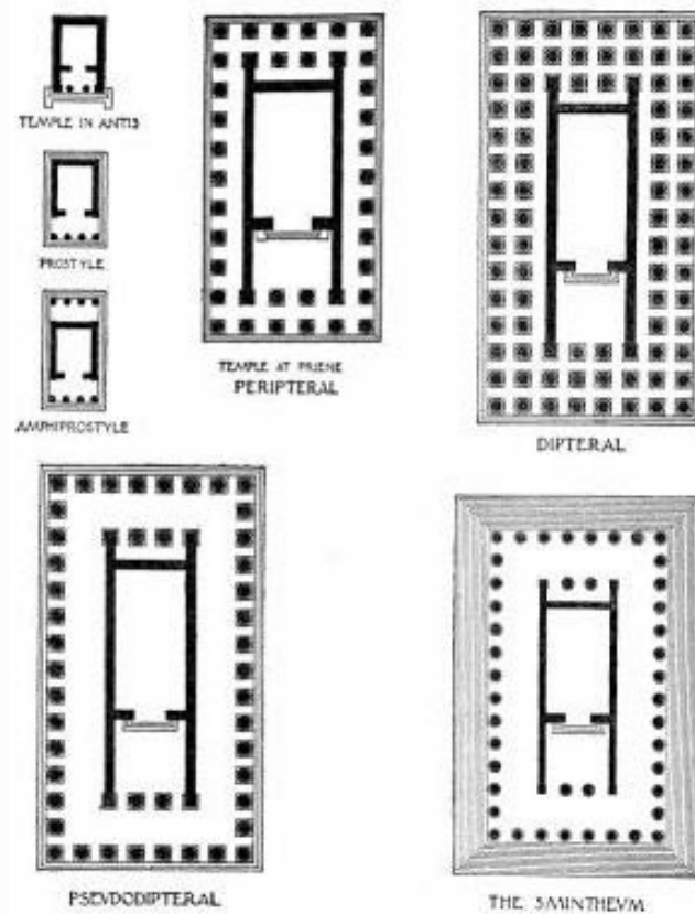
THE CLASSIFICATION OF TEMPLES ACCORDING TO THE ARRANGEMENTS OF THE COLONNADES
