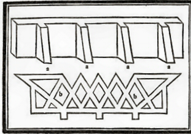
RETAINING WALLS
