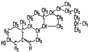
a Cholesterin
