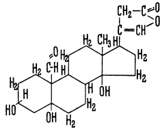
b Strophanthidin
