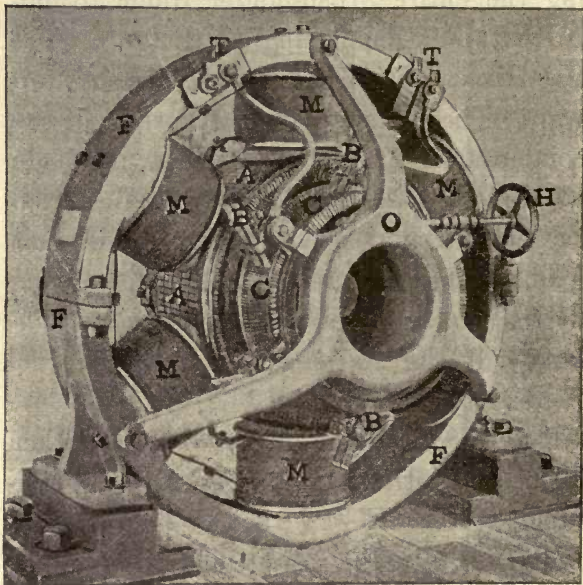
FIG. 108.—SIX-POLE GENERATOR.
