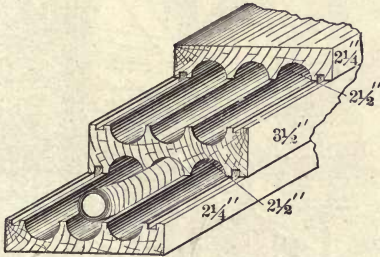
FIG. 94.--CONDUIT OF CREOSOTED WOOD CUT AWAY TO SHOW STRUCTURE.
