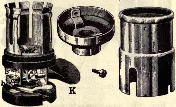
FIG. 27.—DETAILS OF SOCKET.
