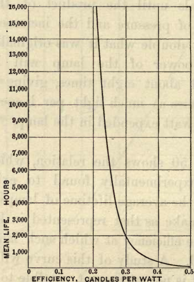
FIG. 50.—CURVE SHOWING THE MEAN DURATION OF LIFE IN A PARTICULAR CLASS OF INCANDESCING LAMPS AT VARIOUS EFFICIENCIES.
