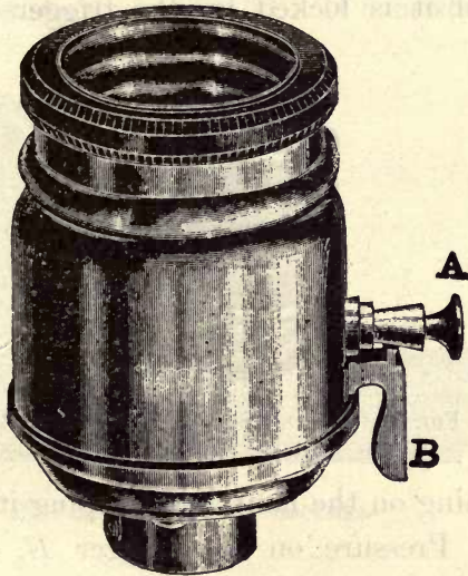
FIG. 30.—PUSH BUTTON KEY SOCKET.
