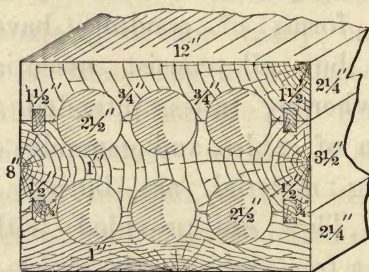
FIG. 93.—CONDUIT OF CREOSOTED WOOD.
