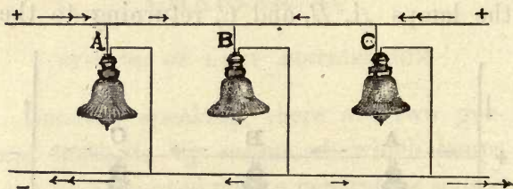
FIG. 54.—MULTIPLE-CONNECTED LAMPS.
