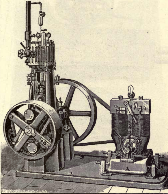
FIG. 110.—BELT-DRIVEN GENERATOR FOR ISOLATED PLANTS.
