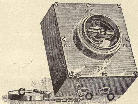
FIG. 145.—WATER-TIGHT MARINE SWITCH.
