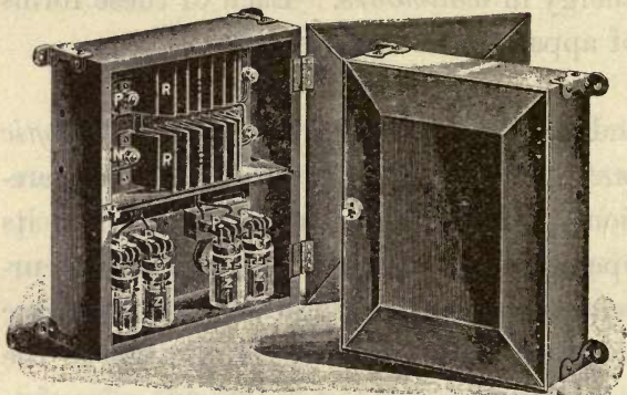
FIG. 114.—ELECTROLYTIC METER.
