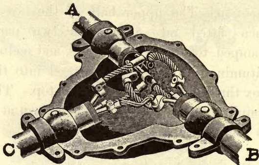
FIG. 101.—BRANCH COUPLING BOX.
