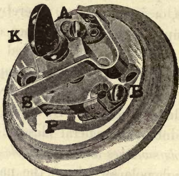
FIG. 84.—SIMPLE FORM OF SINGLE-POLE SWITCH.
