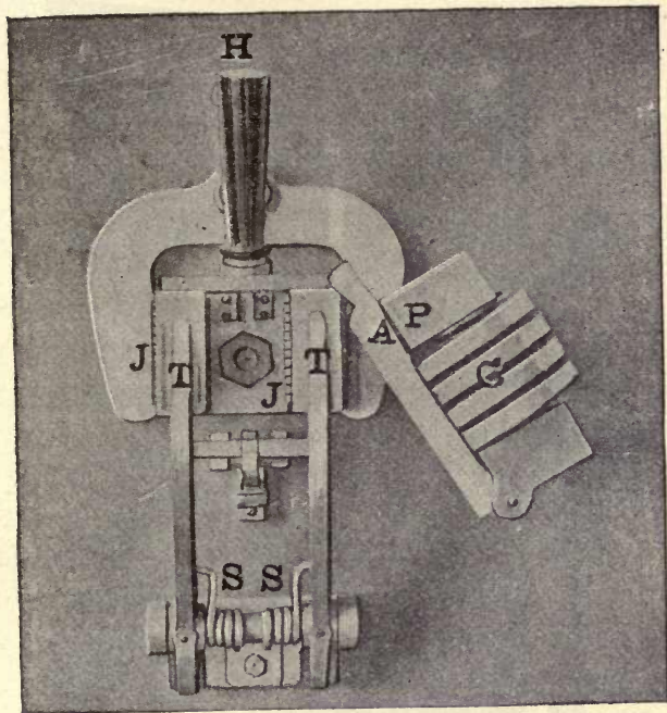
FIG. 125.—OVERLOAD SWITCH, CLOSED.
