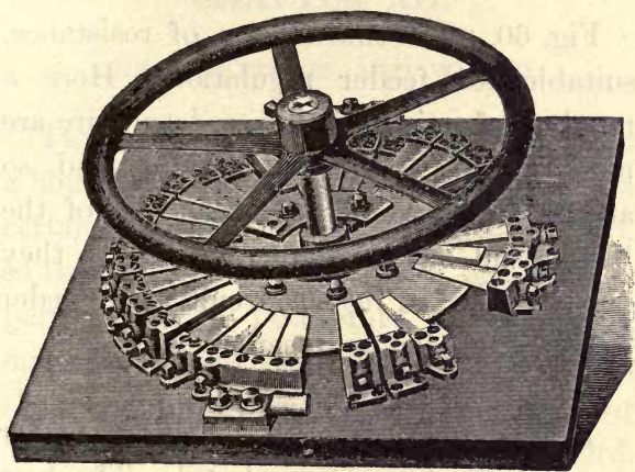
FIG. 61.—EQUALIZER SWITCH.
