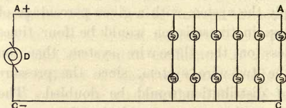
FIG. 56.—MULTIPLE-SERIES CONNECTION.
