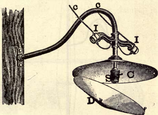
FIG. 131.—STREET FIXTURE, WITH LAMP REMOVED AND SOCKET EXPOSED.
