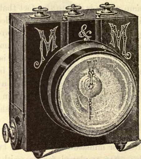
FIG. 142.—SAFETY LAMP FOR MINES.
