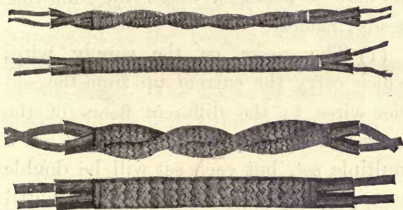
FIG. 73.—FORMS OF DOUBLE FLEXIBLE CONDUCTORS.
