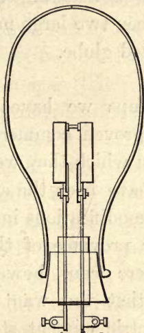
FIG. 6.—FARMER'S LAMP.
