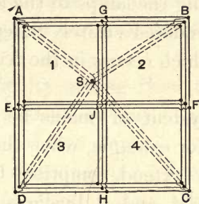
FIG. 59.—DIAGRAM OF THREE-WIRE FEEDER DISTRIBUTION.
