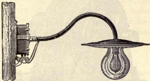
FIG. 137.—SERIES-CONNECTED STREET LAMP FOR ALTERNATING-CURRENT CIRCUITS.
