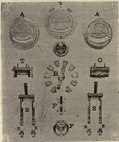
FIG. 123.—STORAGE BATTERY SWITCHBOARD.
