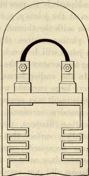
FIG. 13.—HORSESHOE LAMP.
