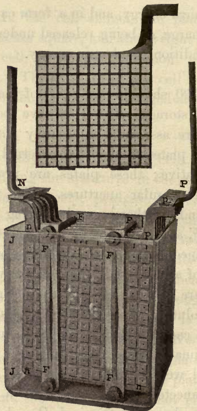
FIG. 120.—STORAGE CELL.
