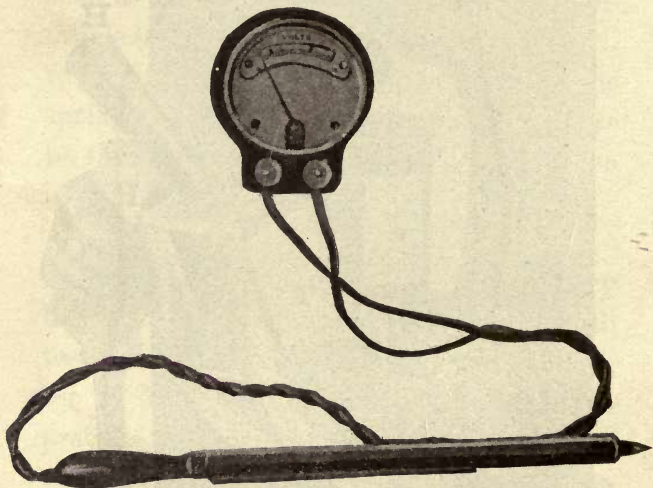
FIG. 127.—STORAGE CELL VOLTMETER AND ELECTRODES.
