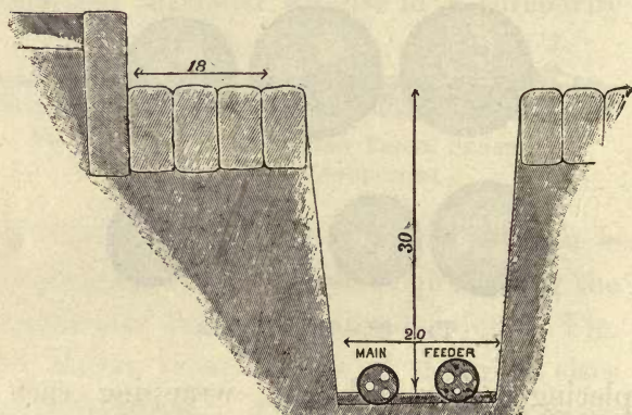
FIG. 99.—SECTION OF STREET TRENCH CONTAINING A FEEDER AND MAIN TUBE.
