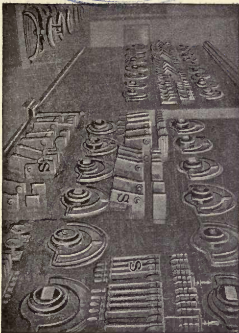
FIG. 105.—PARTIAL VIEW OF SWITCHBOARD.
