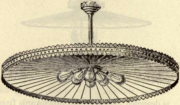
FIG. 40.—PANEL REFLECTOR AND SHADE FOR CLUSTER.
