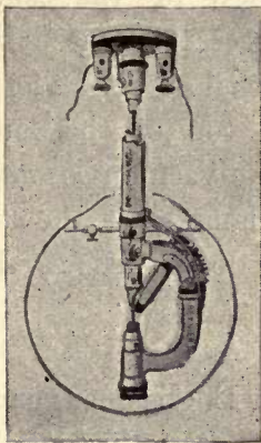
FIG. 8.—REYNIER'S LAMP.
