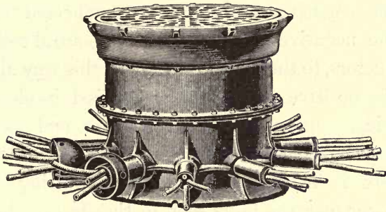
FIG. 104.—JUNCTION BOX.
