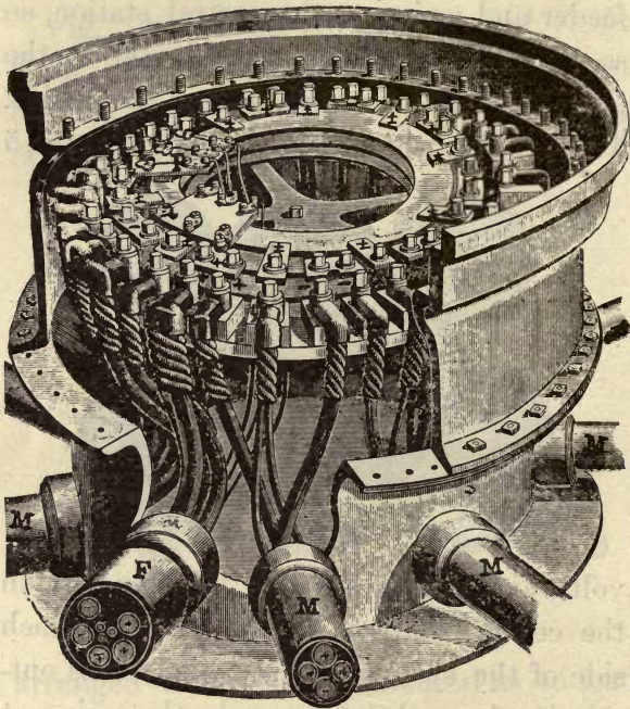
FIG. 103.—JUNCTION BOX.
