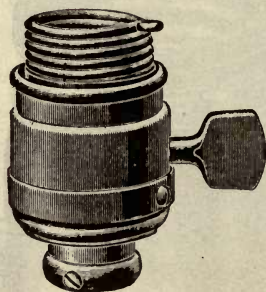
FIG. 31.—SPRING SOCKET FOR SCREW BASE.
