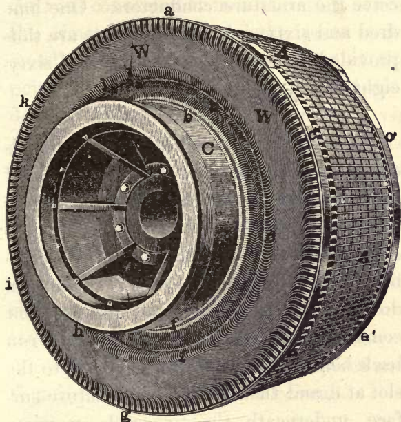
FIG. 109.—ARMATURE OF GENERATOR.
