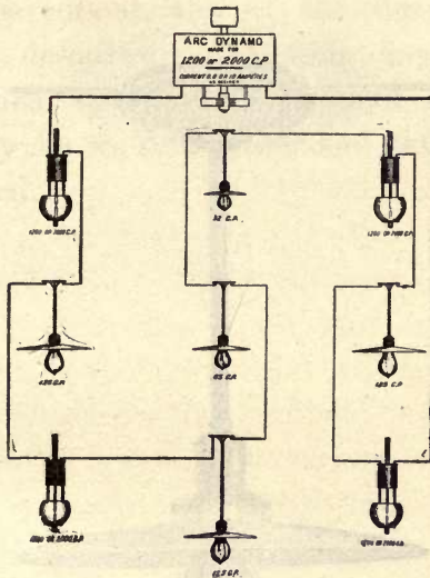
FIG. 134.—SERIES ARC AND INCANDESCENT CIRCUIT.
