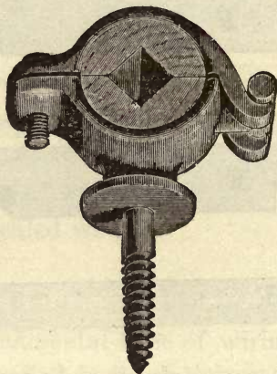
FIG. 75.—FORM OF SCREW CLEAT.
