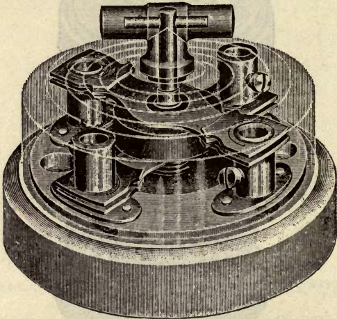
FIG. 86.—LARGER FORM OF DOUBLE-POLE SWITCH.
