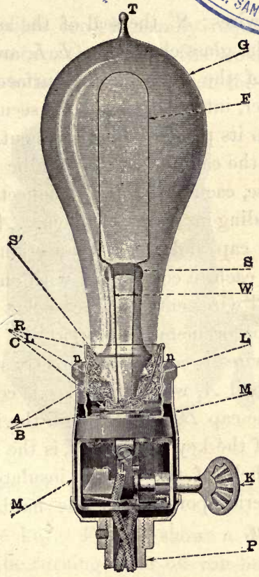
FIG. 29.—LAMP AND SOCKET SHOWING CONNECTIONS.
