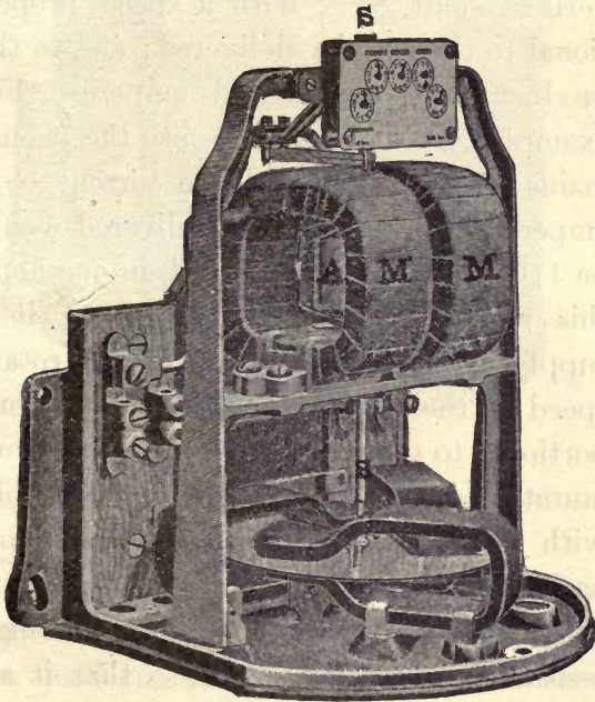
FIG. 116.—INTERIOR OF RECORDING WATTMETER.
