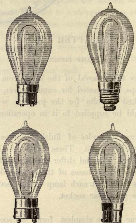
FIG. 23.—COMPLETED INCANDESCENT LAMPS.
