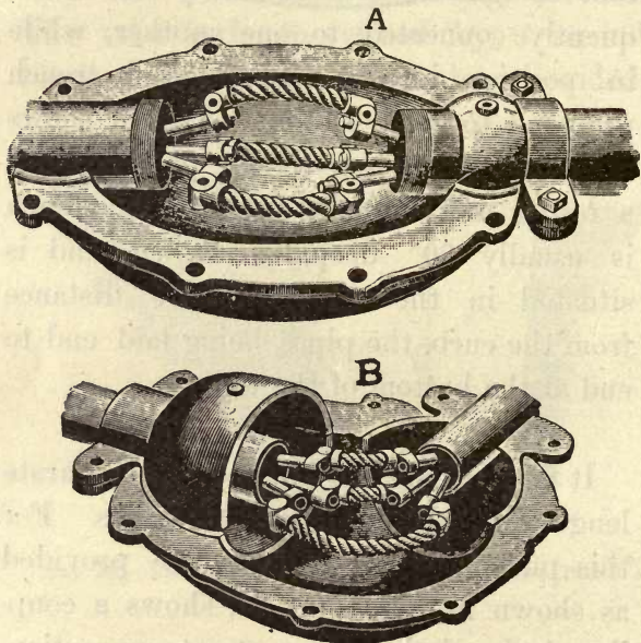
FIG. 100.—COUPLING BOXES.
