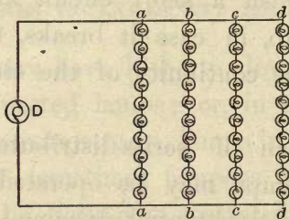
129.—MULTIPLE-SERIES SYSTEM.
