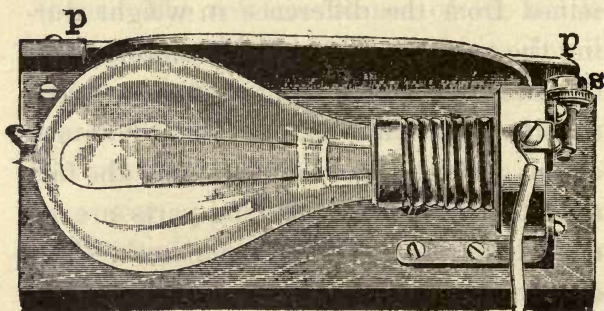
FIG. 115.—THERMOSTAT FOR ELECTROLYTIC METERS.
