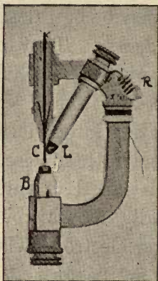
FIG. 7.—REYNIER'S LAMP.
