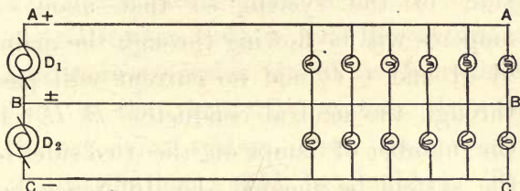
FIG. 55.—THREE-WIRE SYSTEM, SERIES-MULTIPLE CONNECTION.
