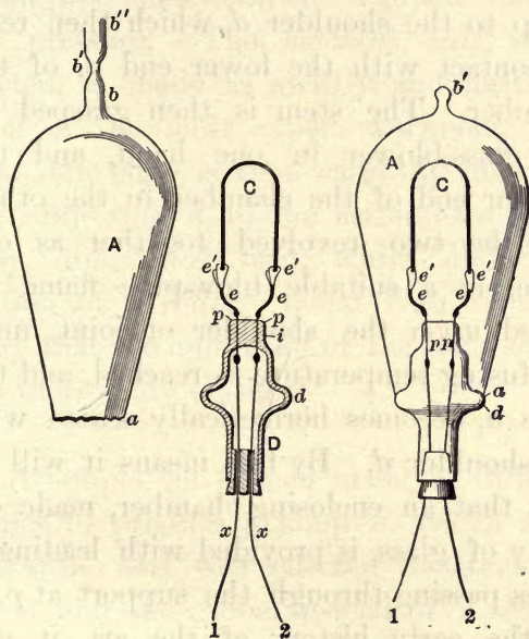
FIG. 17.—STEPS OF SEALING-IN PROCESS.
