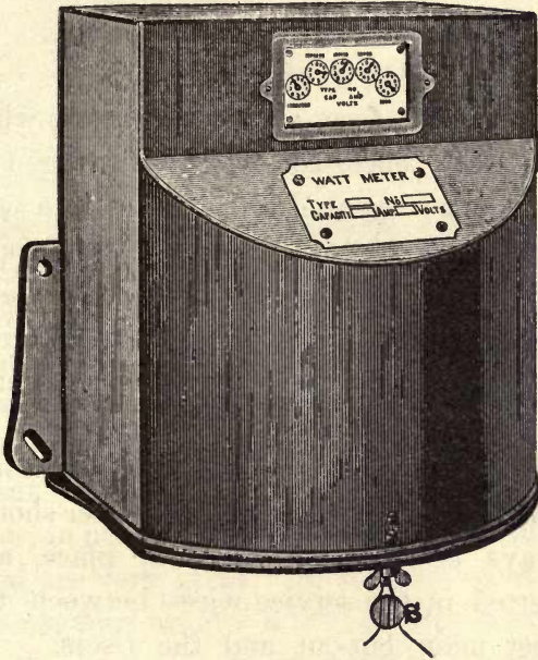
FIG. 117.—RECORDING WATTMETER.
