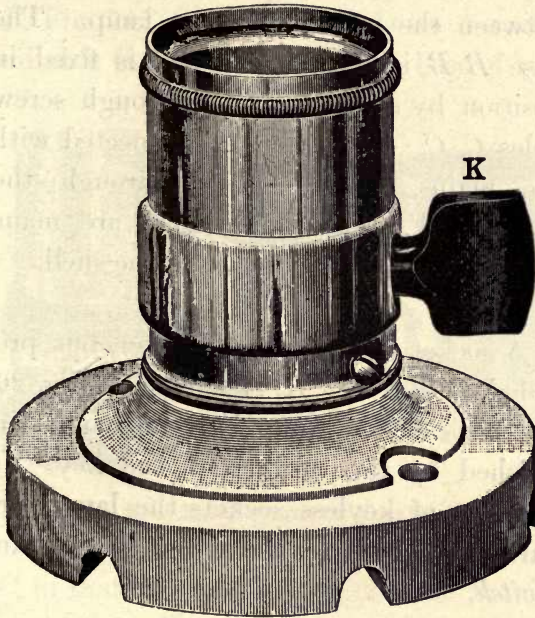
FIG. 26.—KEY WALL-SOCKET.
