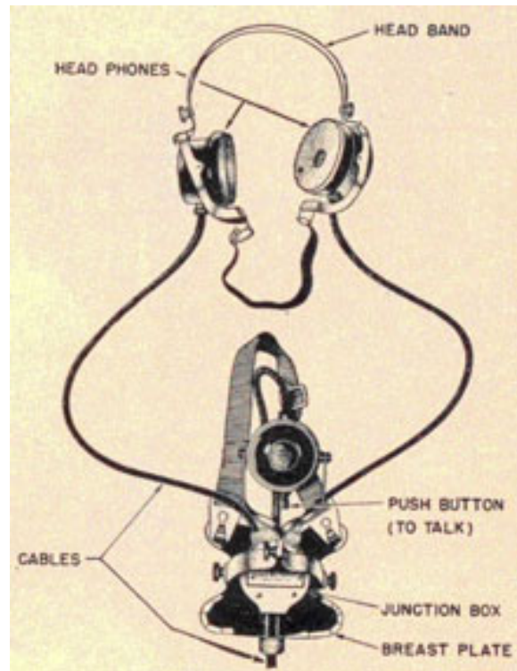
Figure 6-2. The headset.
