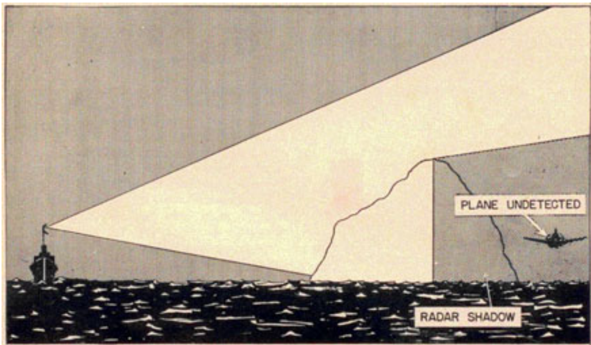
Figure 3-27. Radar shadow.
