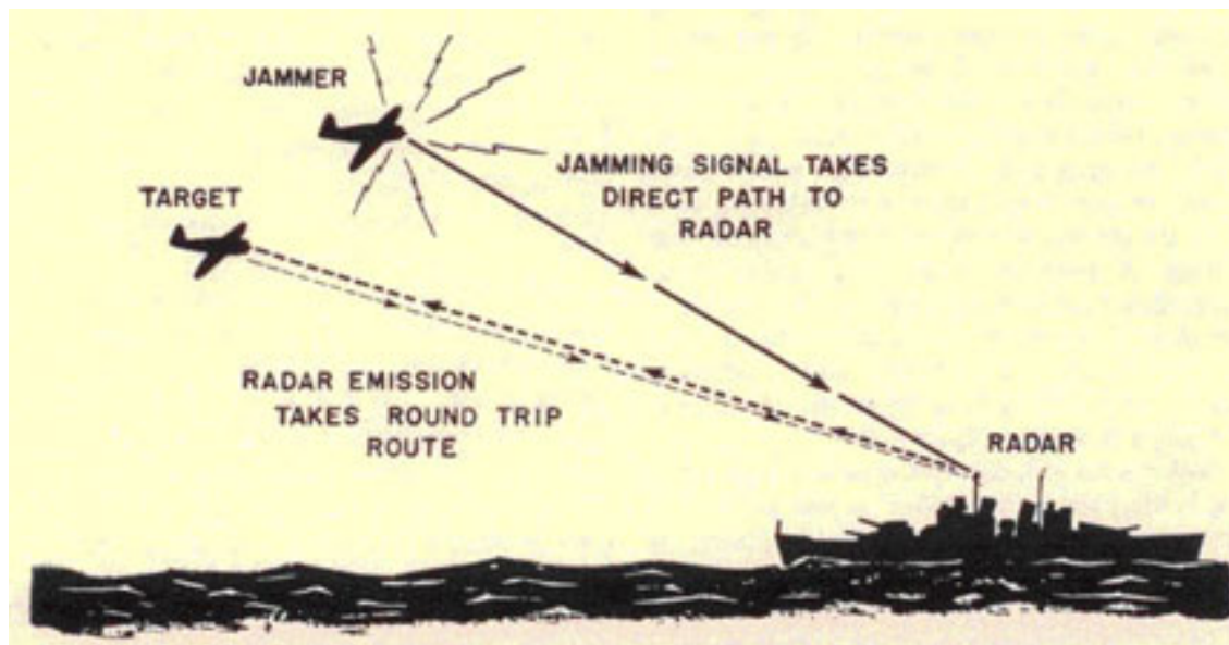
Figure 3-30. Illustration of why electronic jamming is often many times stronger than a radar echo.
