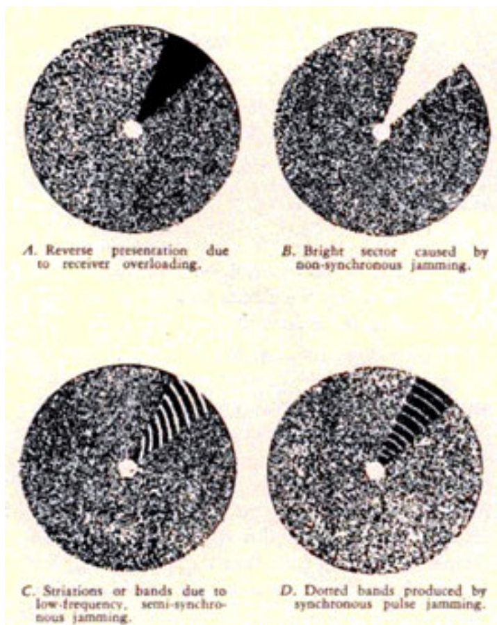
Figure 3-41. The PPI in the presence of jamming.
