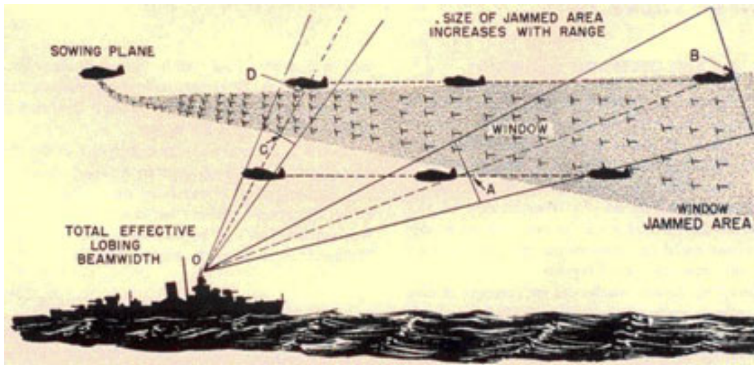
Figure 3-56. Relation between Window dispersal, jammed area and attacking aircraft.
