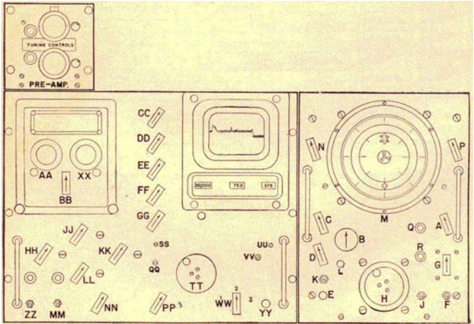
Drawing of receiver, indicator and control unit front panel.
