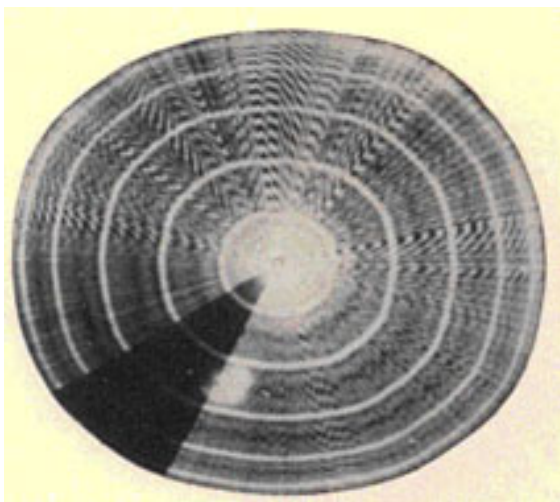
A. Airborne radar, 5-mile sweep. Strong jamming entering side lobes. Echo not visible. Note striations characteristic of semi-synchronous
