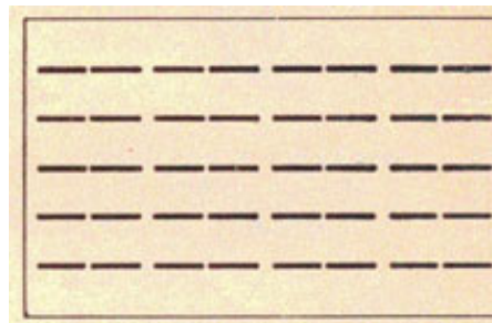
Figure 1-13. Wave lengths.
