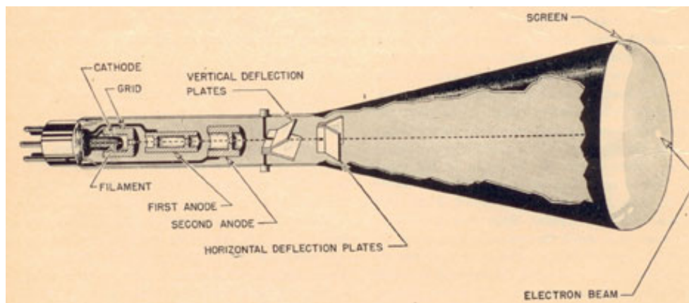
Figure 1-31. Electrostatic cathode-ray tube.
