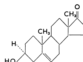
n-Dehydroandrosteron
