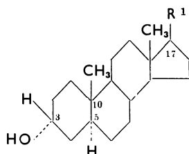
epi-Cholestanol
