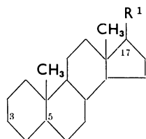
Cholestan
