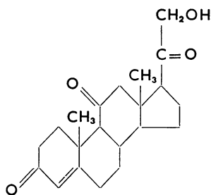
Dehydrocorticosteron
