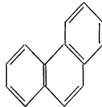
Phenanthren
