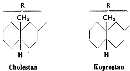
Cholestan
