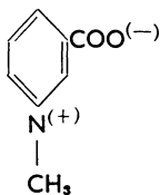
Trigonellin
