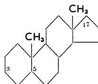
Androstan
