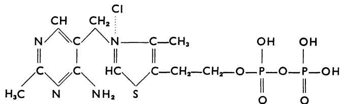
Co-Carboxylase
