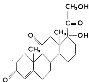
17-Oxydehydrocorticosteron
