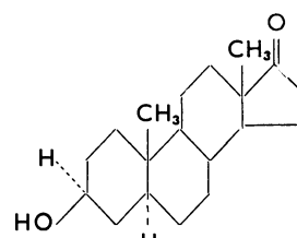
n-Androsteron
