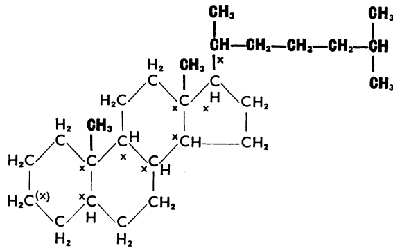
Cholestan
