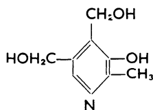
Adermin
