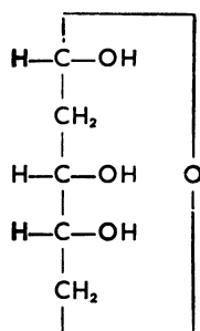
d-(−)-2-Ribodesose (Thyminose)
