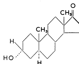
(epi)-Androsteron
