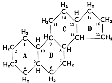
Steran
