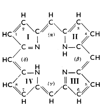
Porphin
