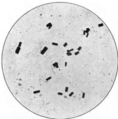
Abb. 8. Caesium-Zink-Goldchlorid.
