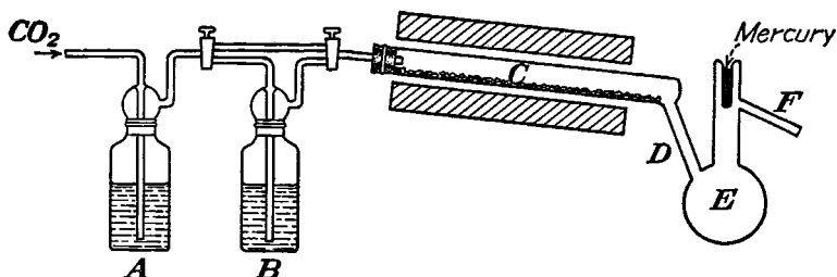
FIG. 8.—Apparatus for the preparation of titanium(IV) bromide.
