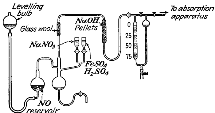
FIG. 10.—Apparatus for the preparation of nitric oxide.
