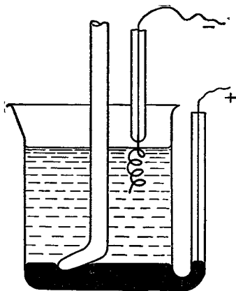
FIG. 2.—Electrolytic cell for producing europium amalgam.
