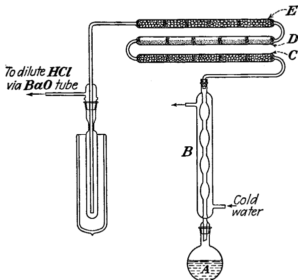
FIG. 18.—Apparatus for preparing anhydrous trimethylamine.
