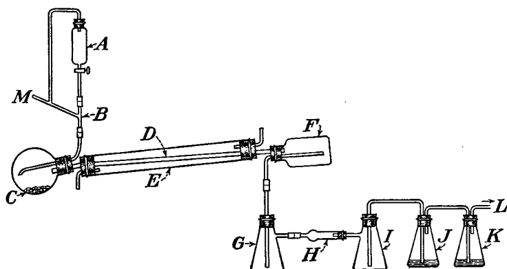
FIG. 15.—Apparatus for the preparation of phosphonium iodide.
