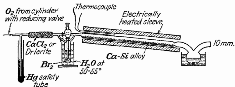
Fig. 6.—Apparatus for the preparation of disilicon hexabromide.
