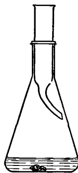
FIG. 1.—Apparatus for dissolving gallium in perchloric acid.
