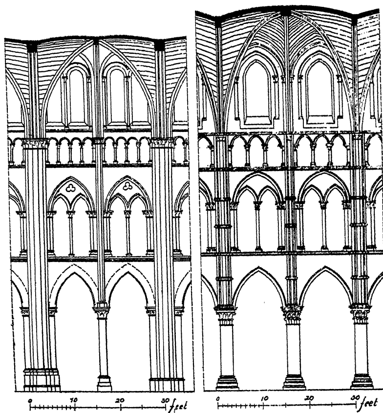
25. ELEVATION OF THE NAVE OF NOYON CATHEDRAL, DESIGNED c. 1150.
