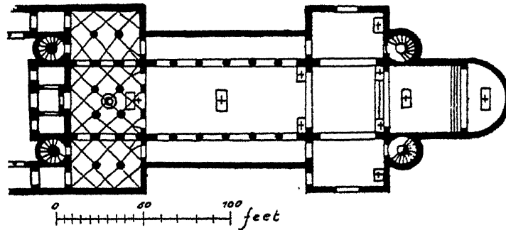
8. CENTULA: ABBEY CHURCH, 790-99 (RECONSTRUCTION).
