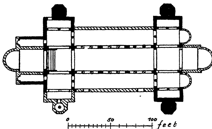
13. HILDESHEIM: ST. MICHAEL'S, BEGUN SHORTLY AFTER 1000.
