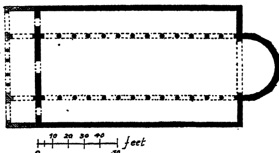
I. RAVENNA: S. APOLLINARE NUOVO, EARLY 6TH CENTURY.
