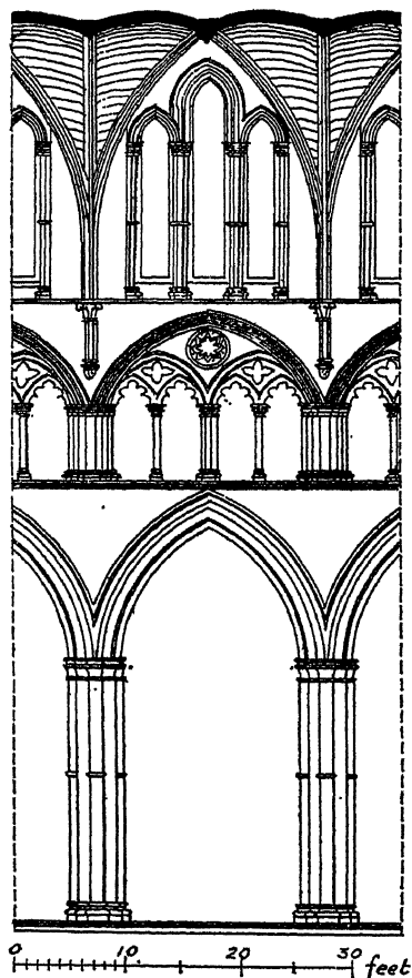
33. ELEVATION OF THE NAVE OF SALISBURY CATHEDRAL, DESIGNED c. 1220.
