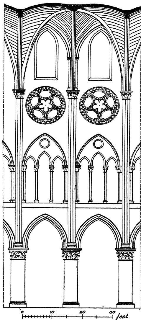
27. PROBABLE ORIGINAL ELEVATION OF THE NAVE OF NOTRE DAME, DESIGNED c. 1170.
