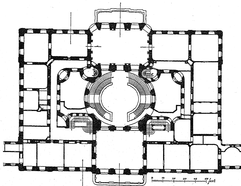
76. BRUCHSAL: EPISCOPAL PALACE. THE CENTRAL STAIRCASE BY BALTHASAR NEUMANN, 1732. TOP; GROUND FLOOR; BOTTOM: FIRST FLOOR.
