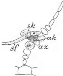
Fig. g. Dudresnaya coccinea . sf=Oblastemfaden (sporogener Faden). sk=dessen Kern (sporogener Kern). az=Auxiliarzelle. ak=deren Kern.
