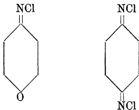
Chinonchlorimid.
