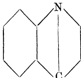
H Chinolin.
