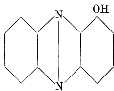
Phenazin.
