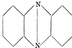
Phenazin.
