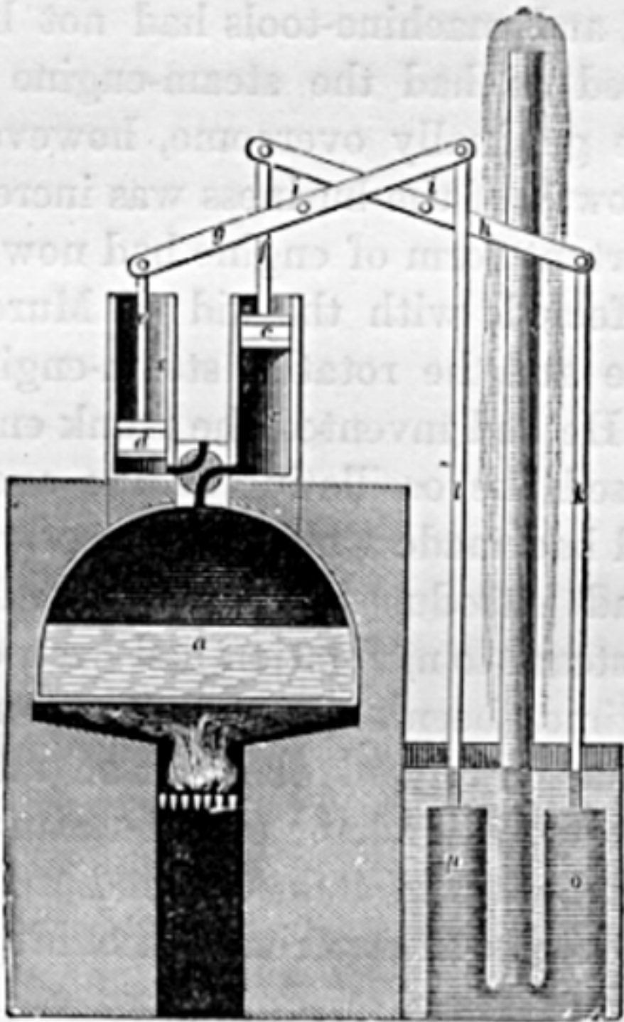
FIG. 41.—Leupold's Engine, 1720.
