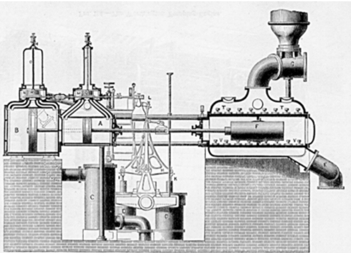
FIG. 103.—The Worthington Pumping-Engine, 1876. Section.
