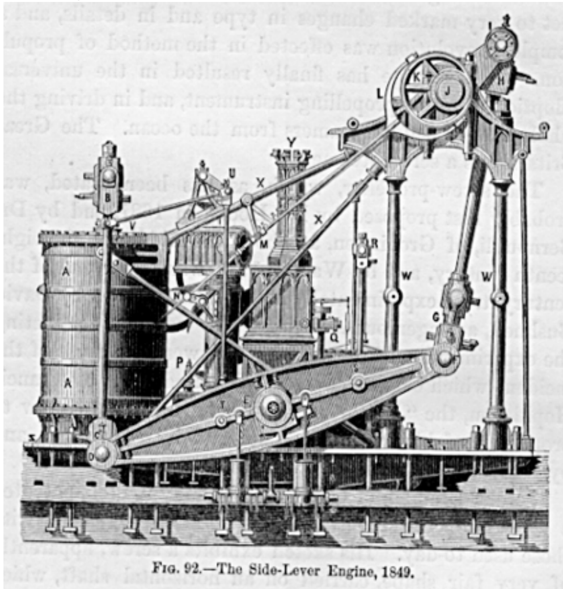
Fig. 92. - The Side-Lever Engine, 1849.
