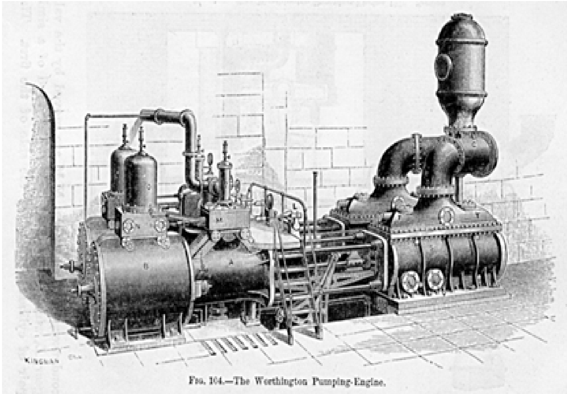
Fig. 104.-The Worthington Pumping-Engine.
