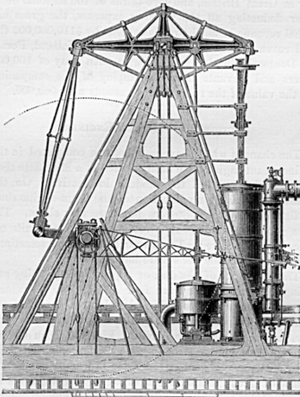
FIG. 130.—Beam-Engine.
