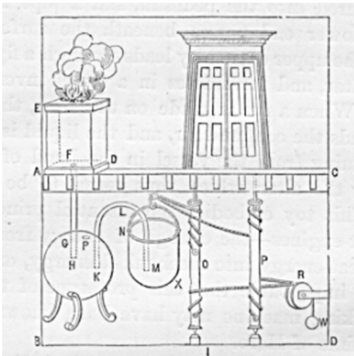
Fig. 1.-Opening Temple-Doors by Steam, B.C. 200.
