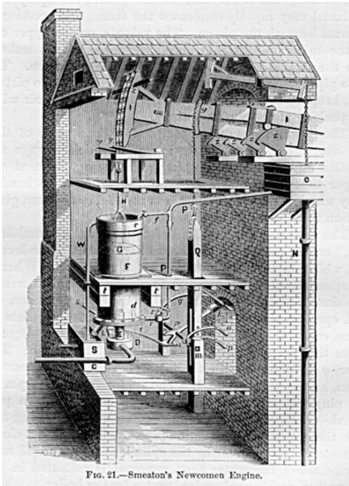
Fig. 21.-Smeaton's Newcomen Engine.
