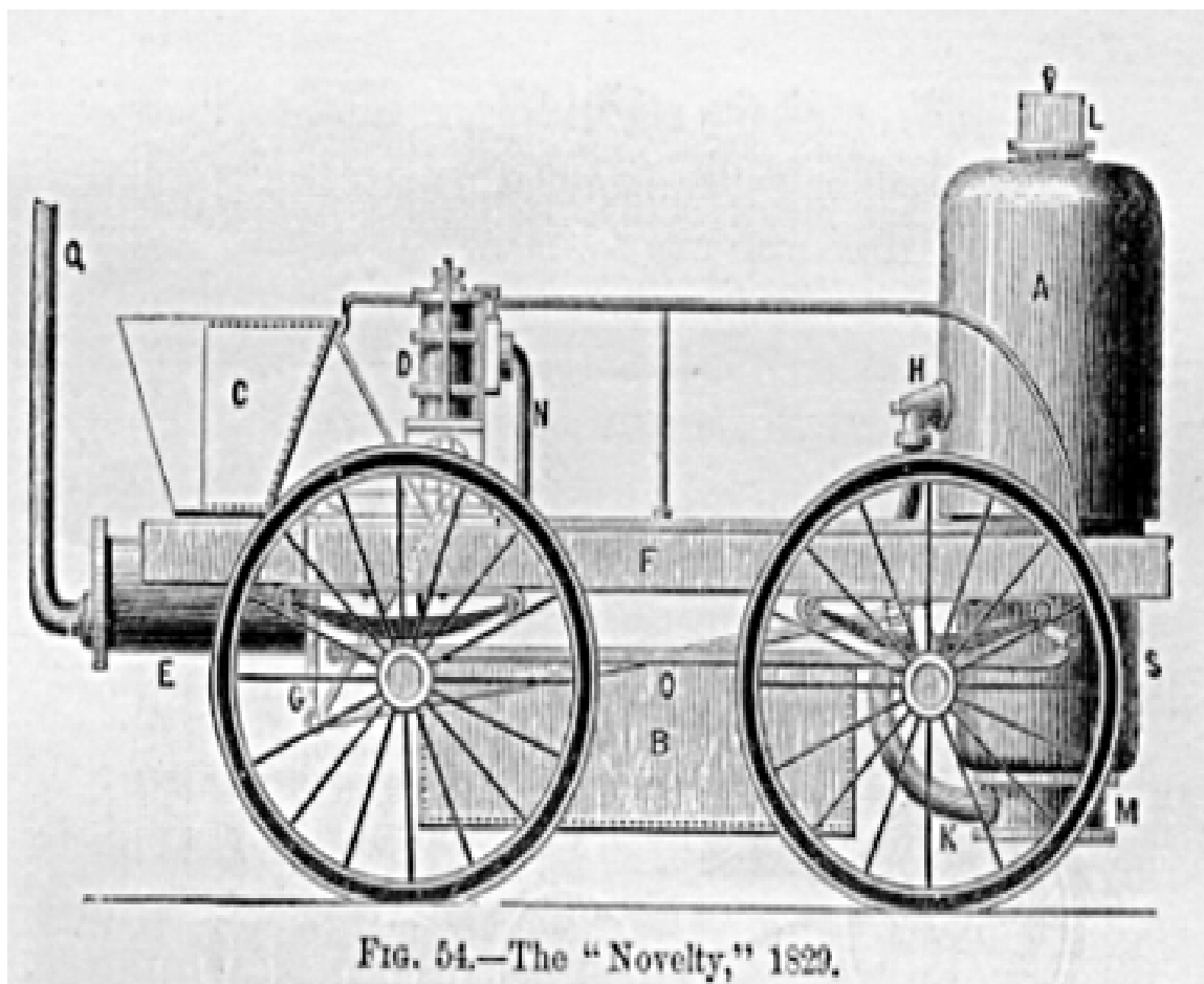
Fig. 54.-The "Novelty," 1829.
