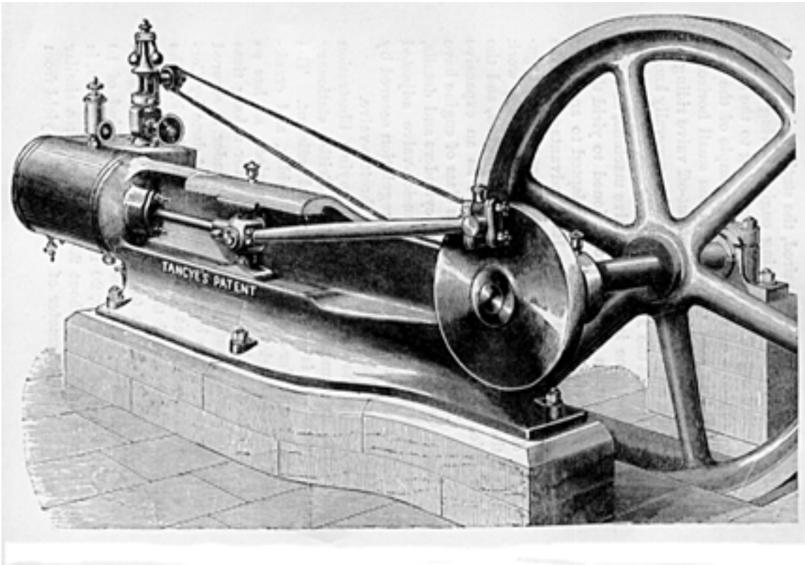
Fig. 95. - Horizontal Stationary Steam-Engine.
