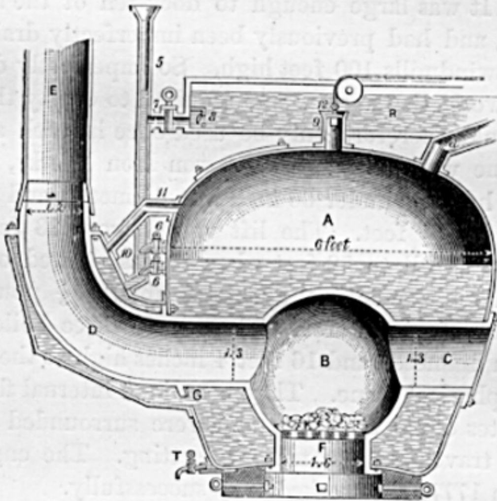
FIG. 23.—Smeaton's Portable-Engine Boiler, 1765.
