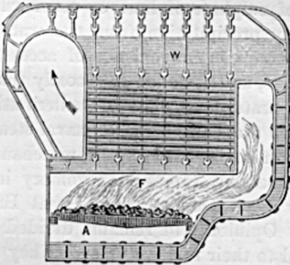
FIG. 142.—Marine Fire-tubular Boiler. Section.
