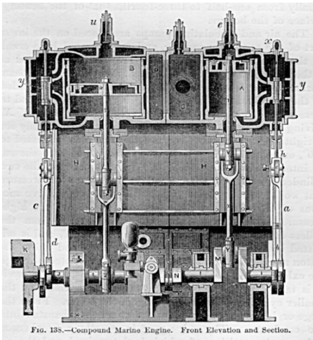
Fig. 138-Compound Marine Engine. Front Elevation and Section.
