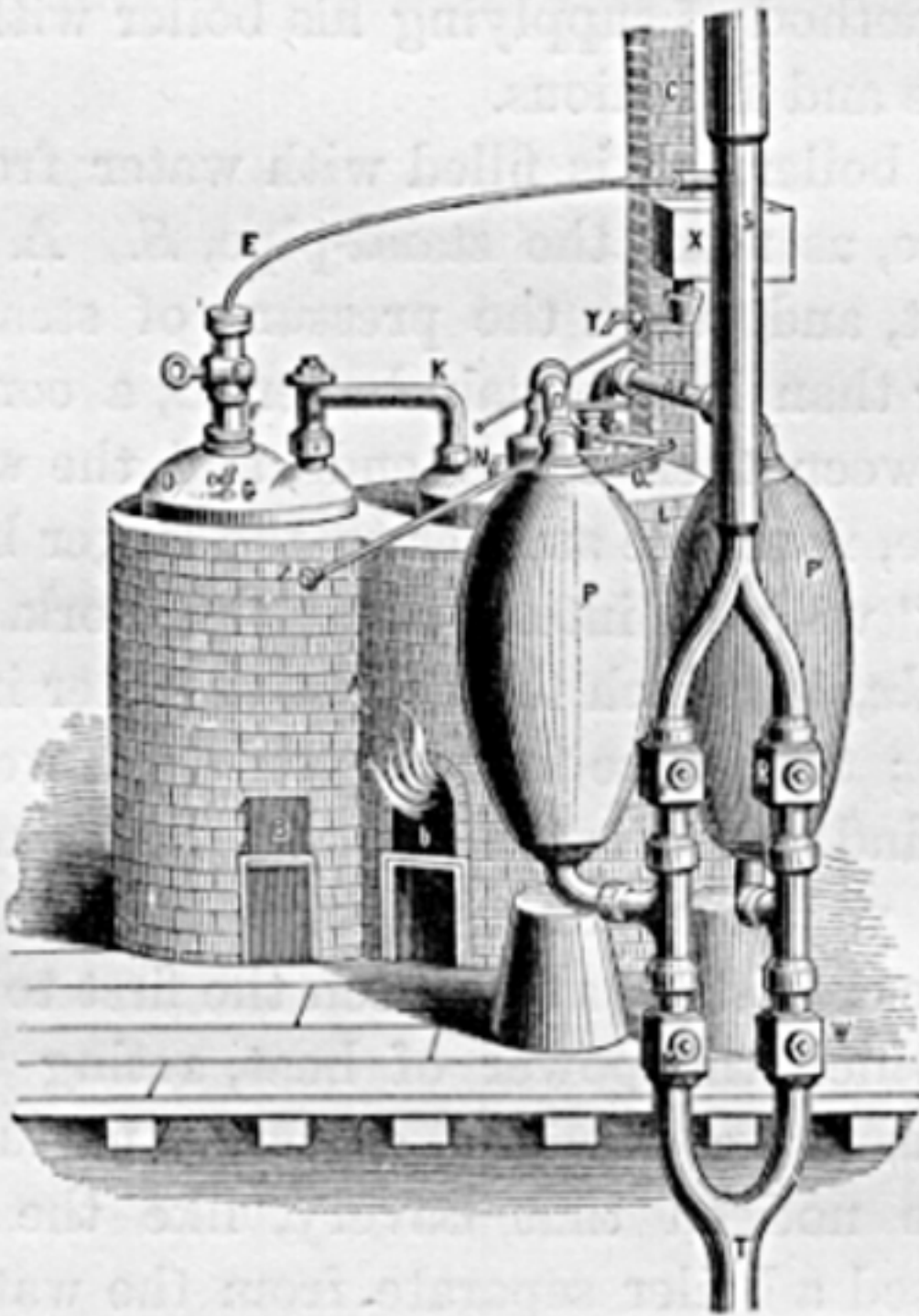
FIG. 13.—Savery's Engine, A. D. 1702.
