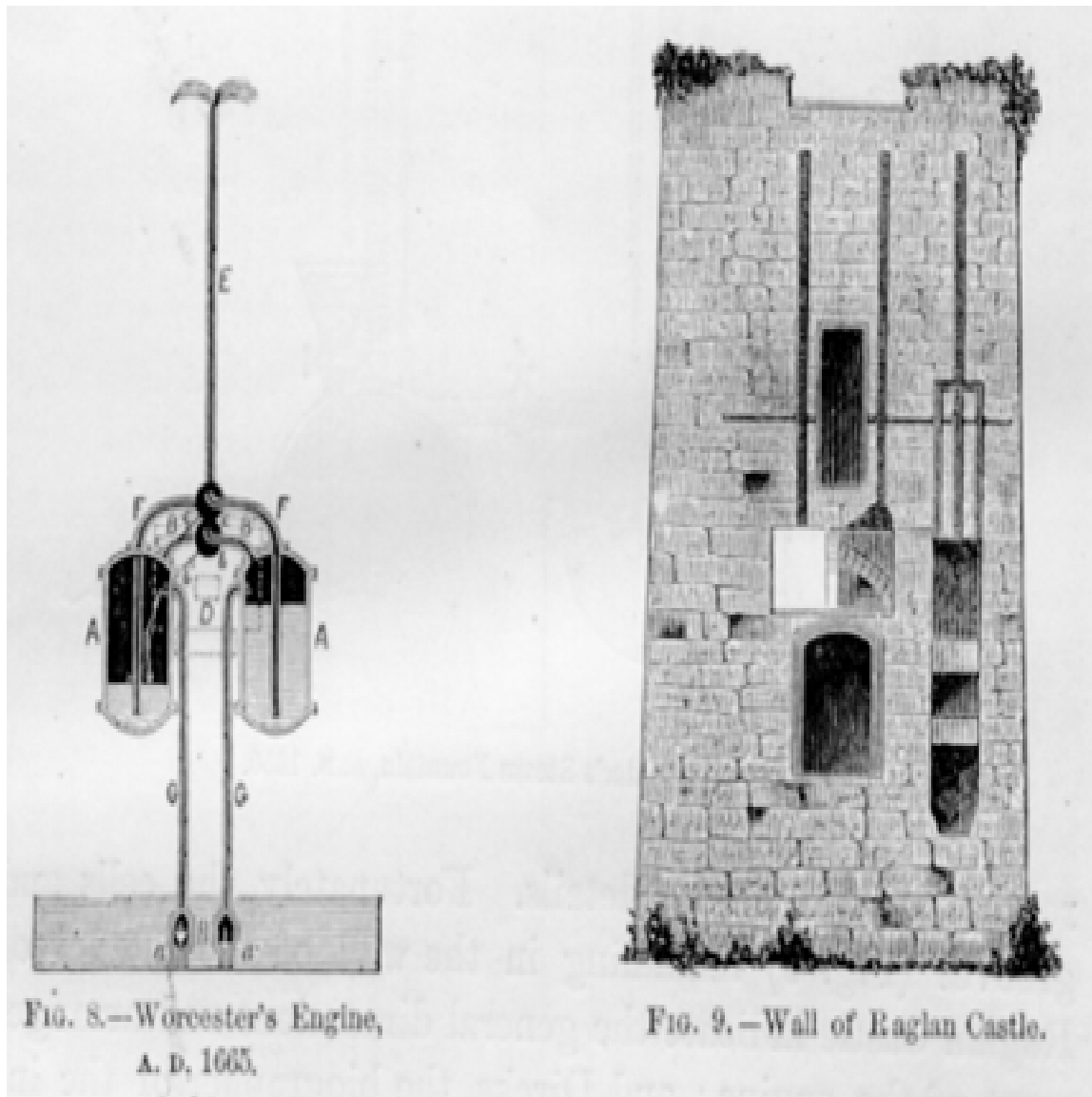
Fig. 8.-Worcester's Engine, A.D. 1665. Fig. 9.-Wall of Raglan Castle.
