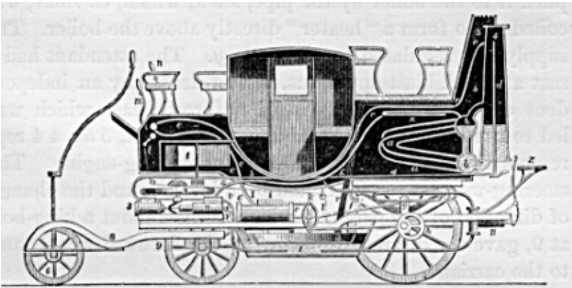
FIG. 48.—Gurney's Steam-Carriage.
