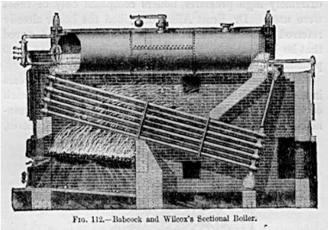
Fig. 112. Babcock and Wilcox's Sectional Boiler.
