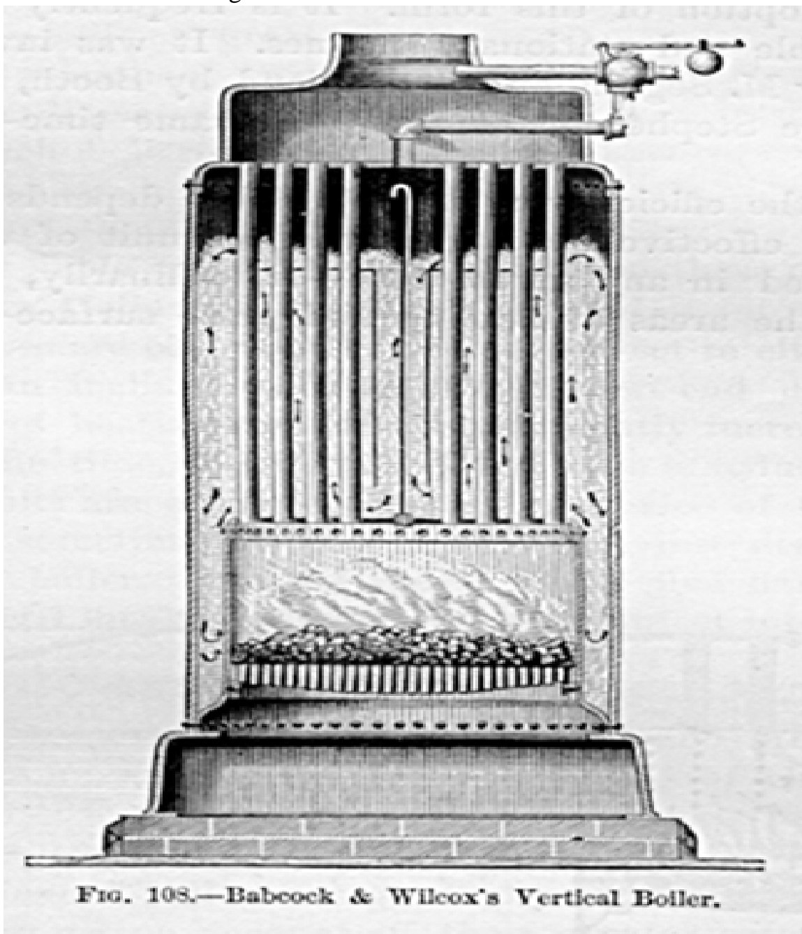
Fig. 108. Babcock & Wilcox's Vertical Boiler.
