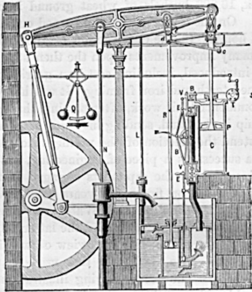
FIG. 31.—Boulton & Watt's Double-Acting Engine, 1784.
