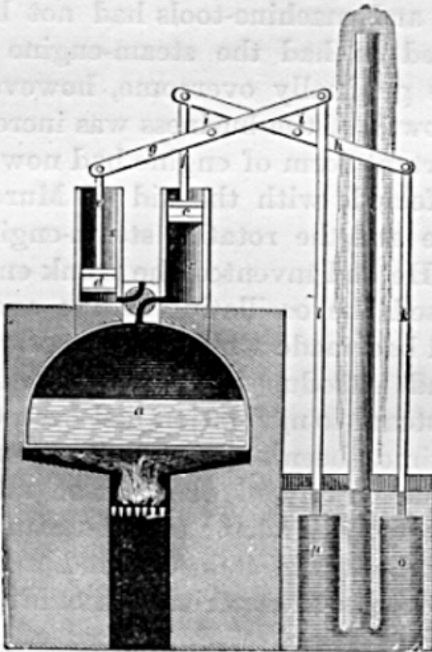
FIG. 41.—Leopold's Engine, 1720.
