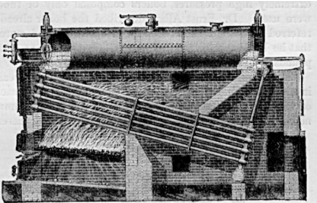
FIG. 112.—Babcock and Wilcox's Sectional Boiler.
