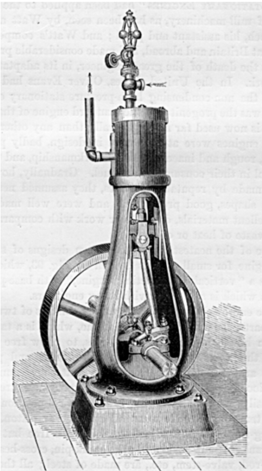
FIG. 93.—Vertical Stationary Steam-Engine.
