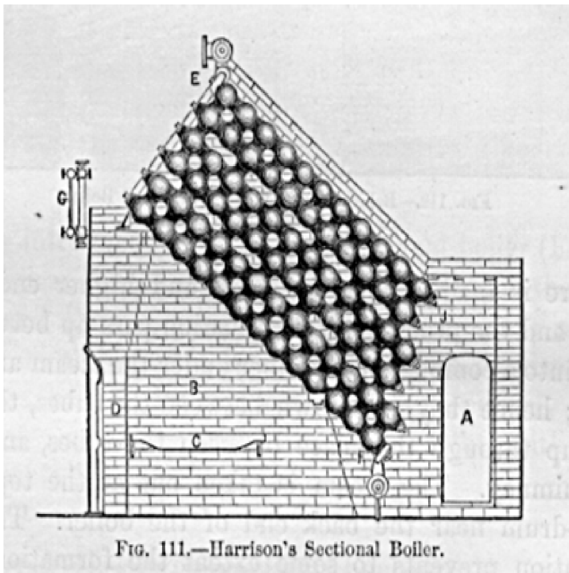
Fig. 111.-Harrison's Sectional Boiler.
