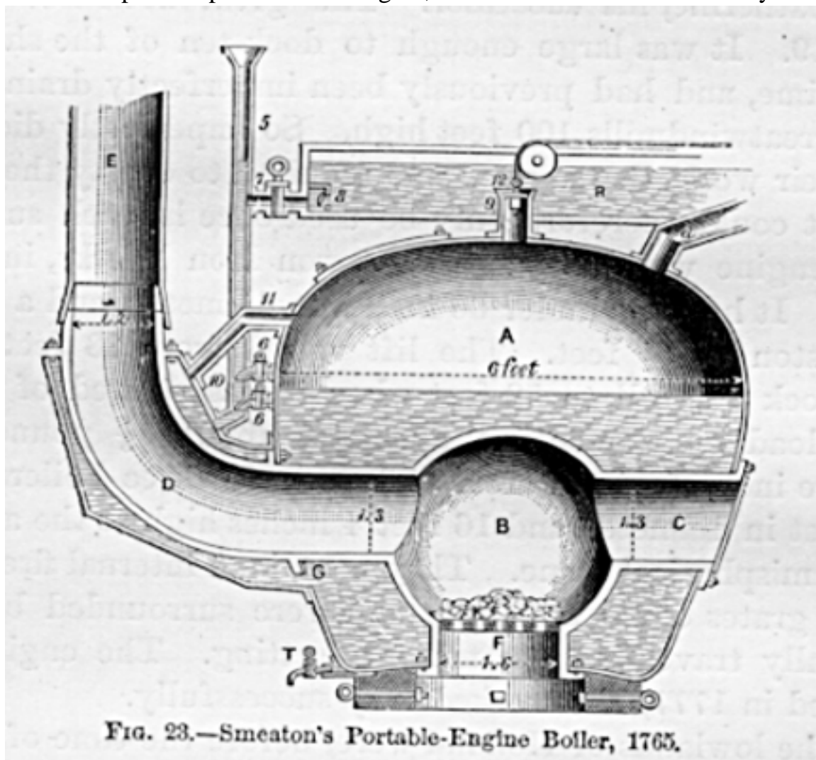
Fig. 23.-Smeaton's Portable Engine Boiler, 1765.
