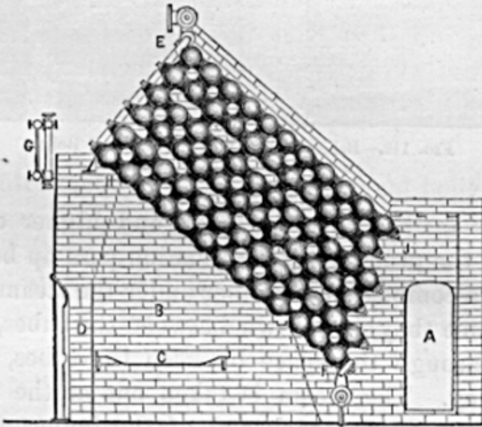
FIG. 111.—Harrison's Sectional Boiler.
