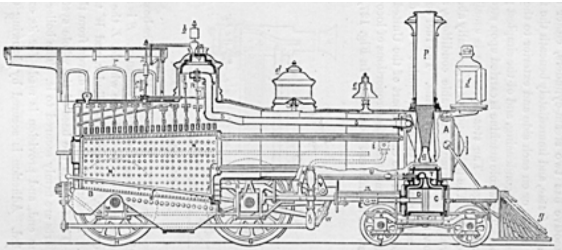
FIG. 125.—The Baldwin Locomotive, Section.
