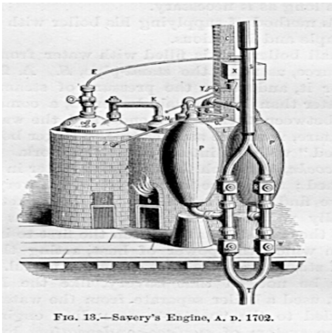
Fig. 13.-Savery's Engine, A.D. 1702.
