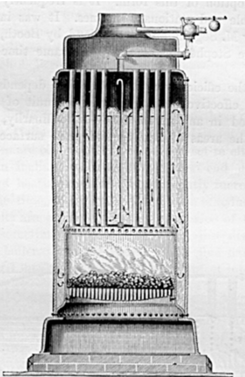
FIG. 108.—Babcock & Wilcox's Vertical Boiler.
