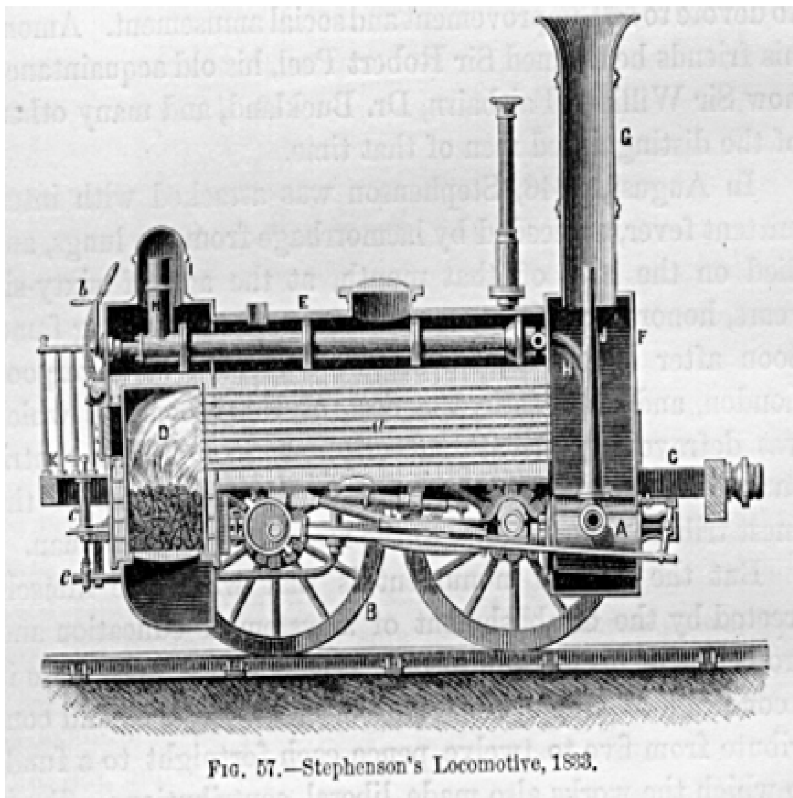
Fig. 57 - Stephenson's Locomotive, 1833.
