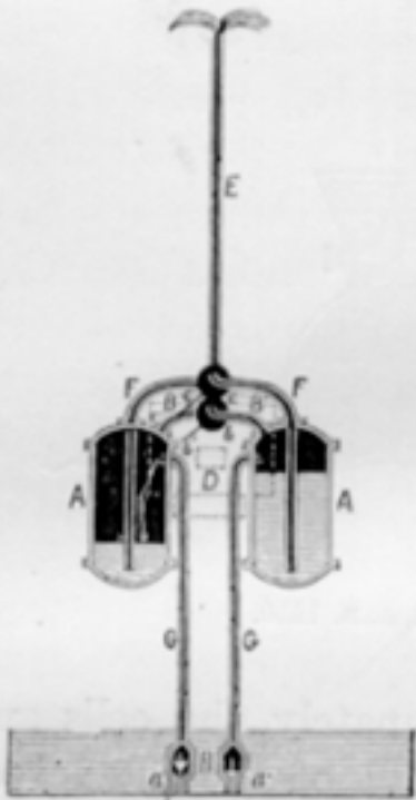
FIG. 8.—Worcester's Engine, A. D. 1665.
