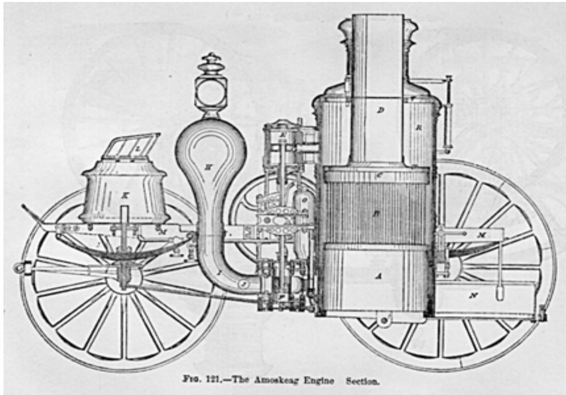
Fig. 121. - The Amoskeag Engine. Section.
