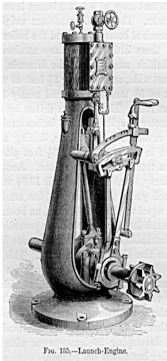
Fig. 135 Launch-Engine.
