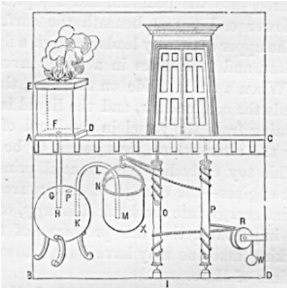
Fig. 2.-Steam Fountain, B.C. 200.
