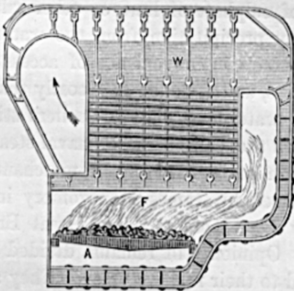
FIG. 142.—Marine Fire-tubular Boiler. Section.
