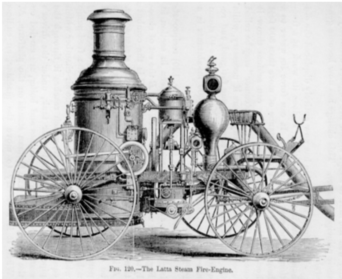
Fig. 120. - The Latta Steam Fire-Engine.
