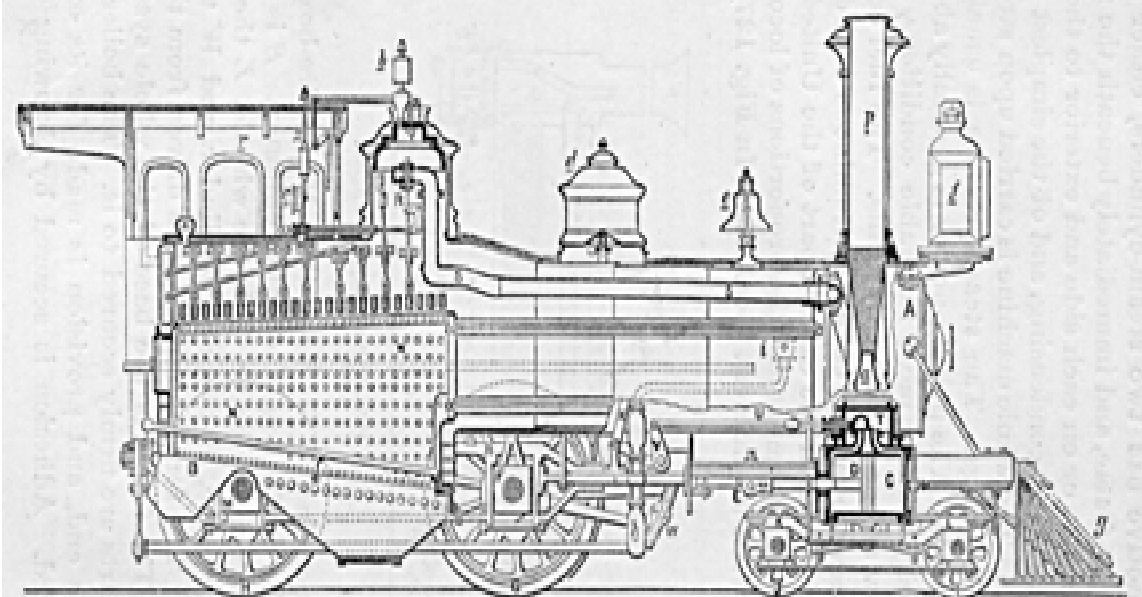
Fig. 128.—The Baldwin Locomotive, Section.
