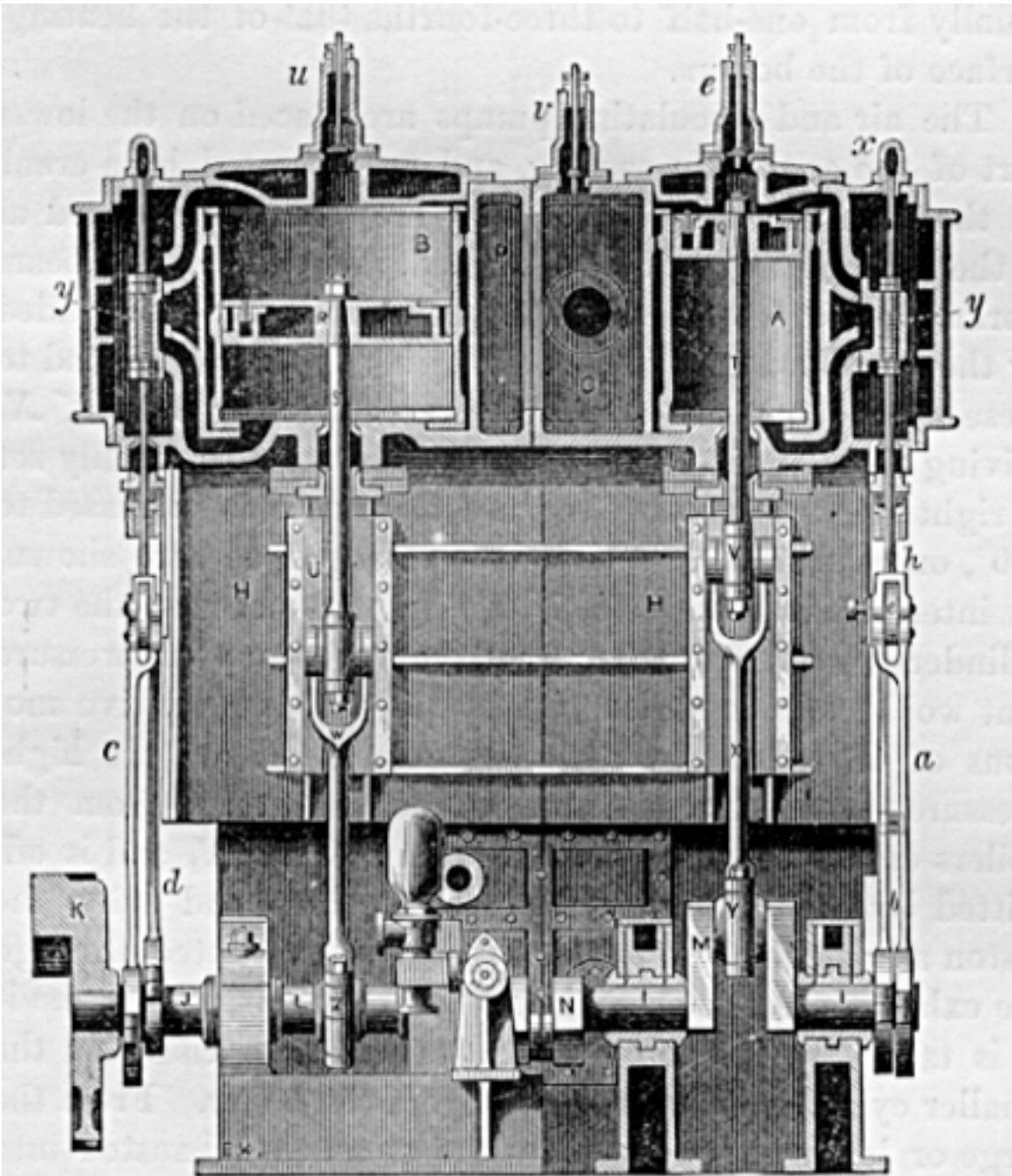
FIG. 138.—Compound Marine Engine. Front Elevation and Section.
