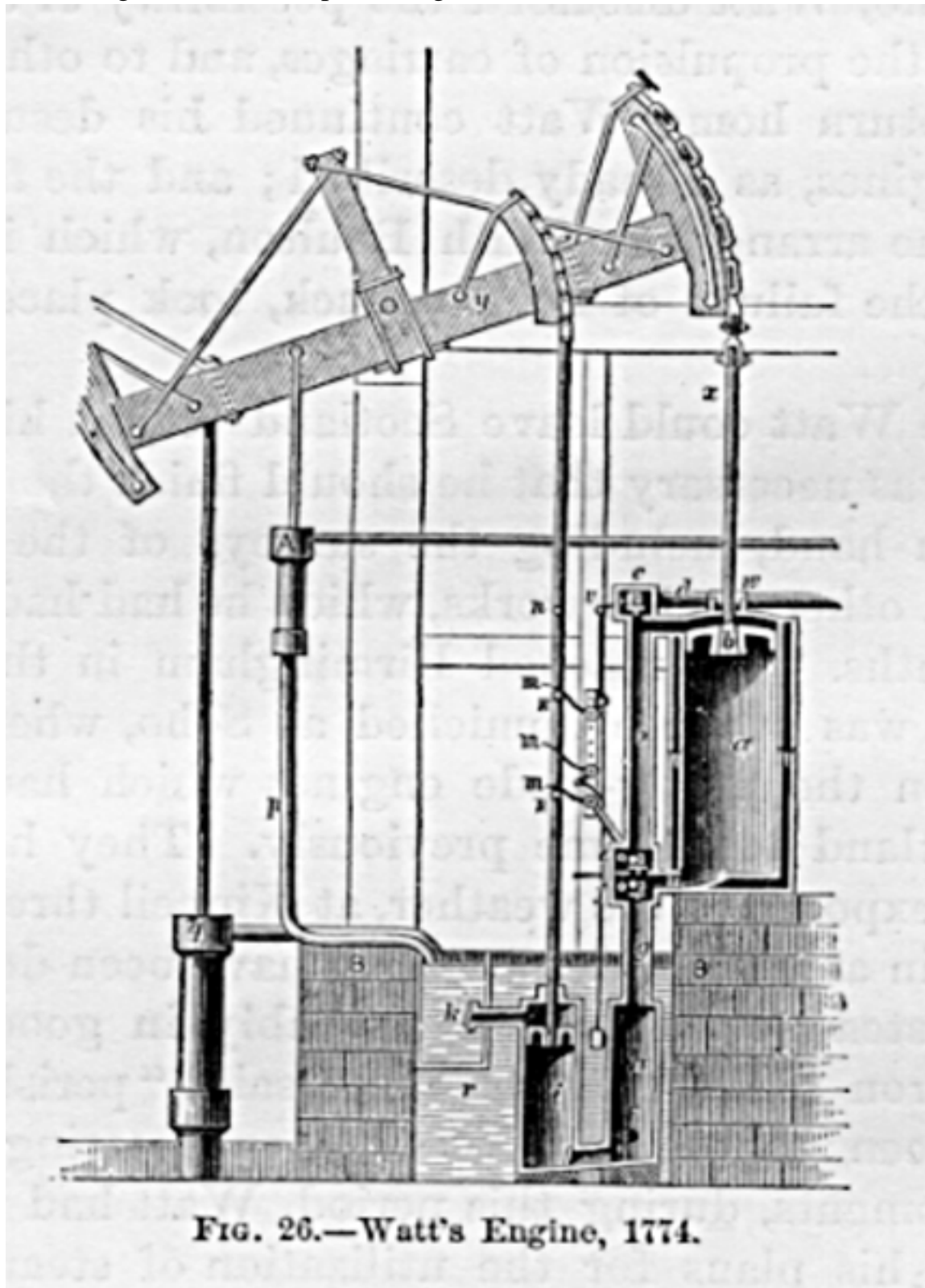
Fig. 26.-Watt's Engine, 1774.
