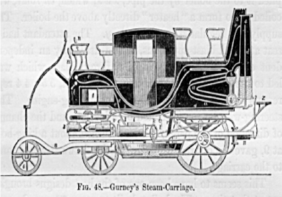
Fig. 48.-Gurney's Steam-Carringe.
