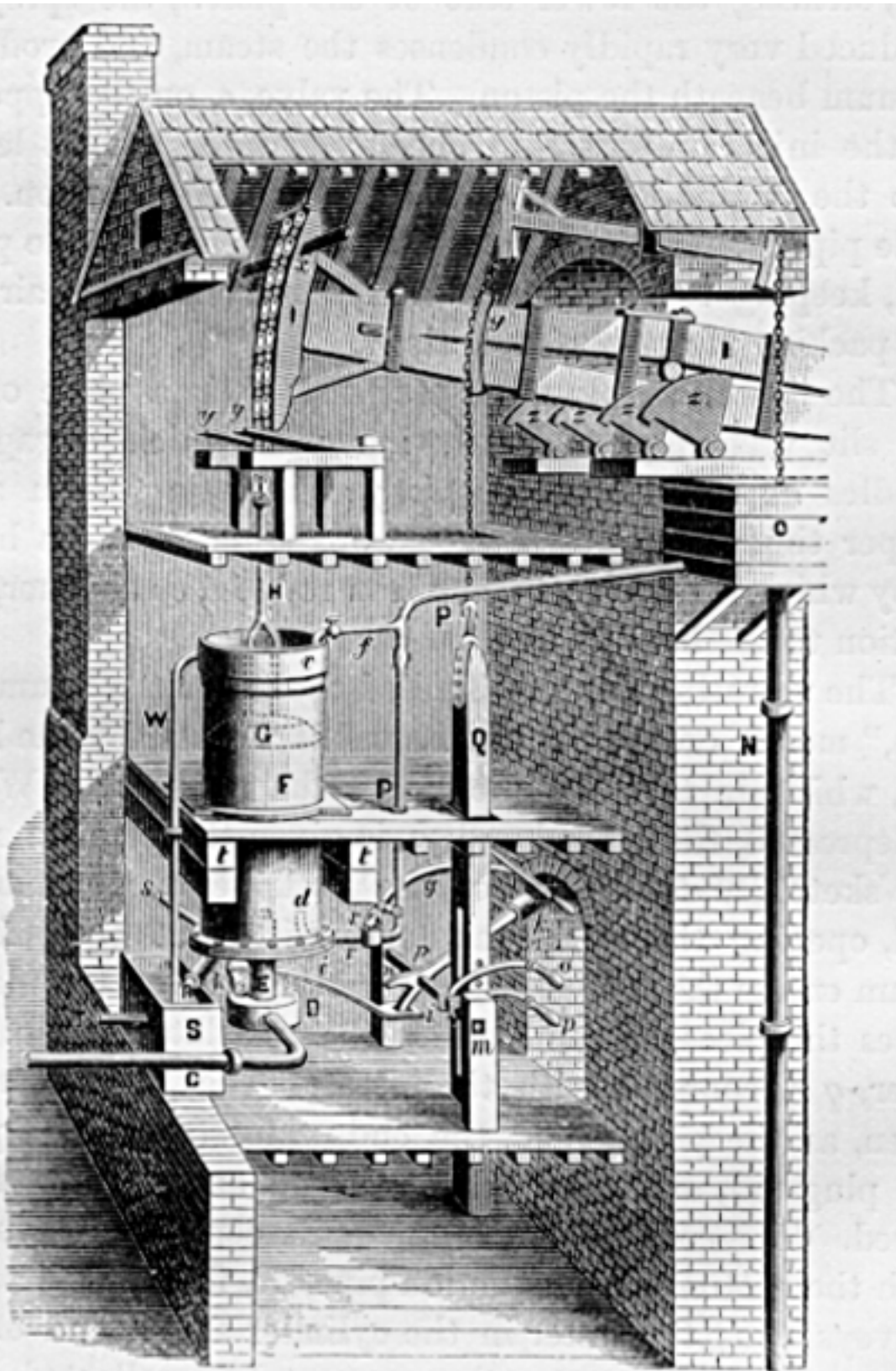
FIG. 21.—Smeaton's Newcomen Engine.
