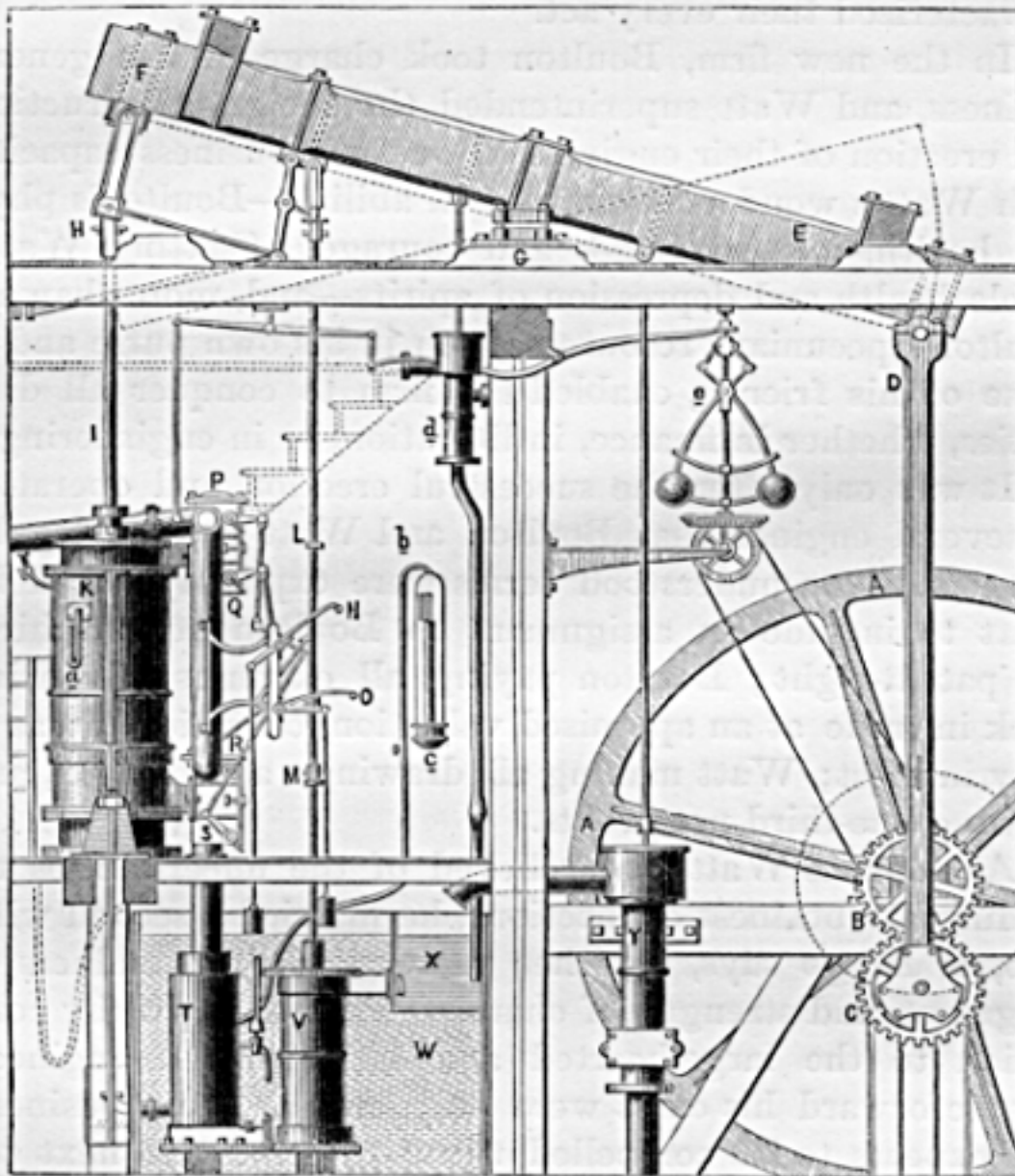
FIG. 27.—Watt's Engine, 1781.
