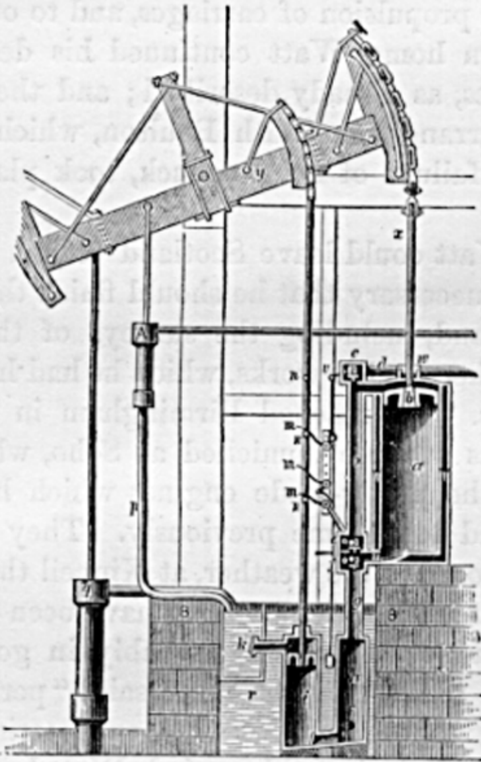
FIG. 26.—Watt's Engine, 1774.
