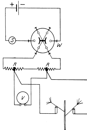
Abb. 20. W = Wippe, R = Widerstand, V = Voltmeter.
