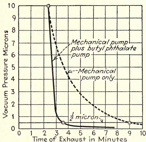
Fig. 70.—Comparison of pumping speeds, showing additional speed obtainable from butyl phthalate pump.
