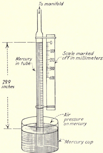
FIG. 65.—Straight gauge.
