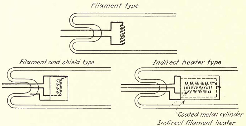
FIG. 14.—Different forms of heater-type (hot-cathode) electrodes.
