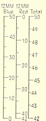
FIG. 104.—Chart for determining the combinations of red and mercury tubing which may be run from a single transformer. The use of the chart is explained in the text on the opposite page.
