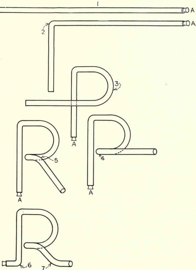
FIG. 50.—Steps in bending the letter "R."
