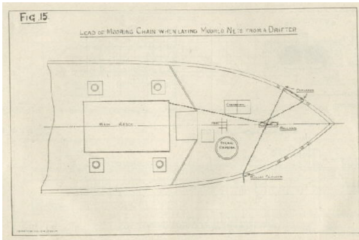
Image of figure 15: Lead of mooring chain when laying moored nets from a drifter.
