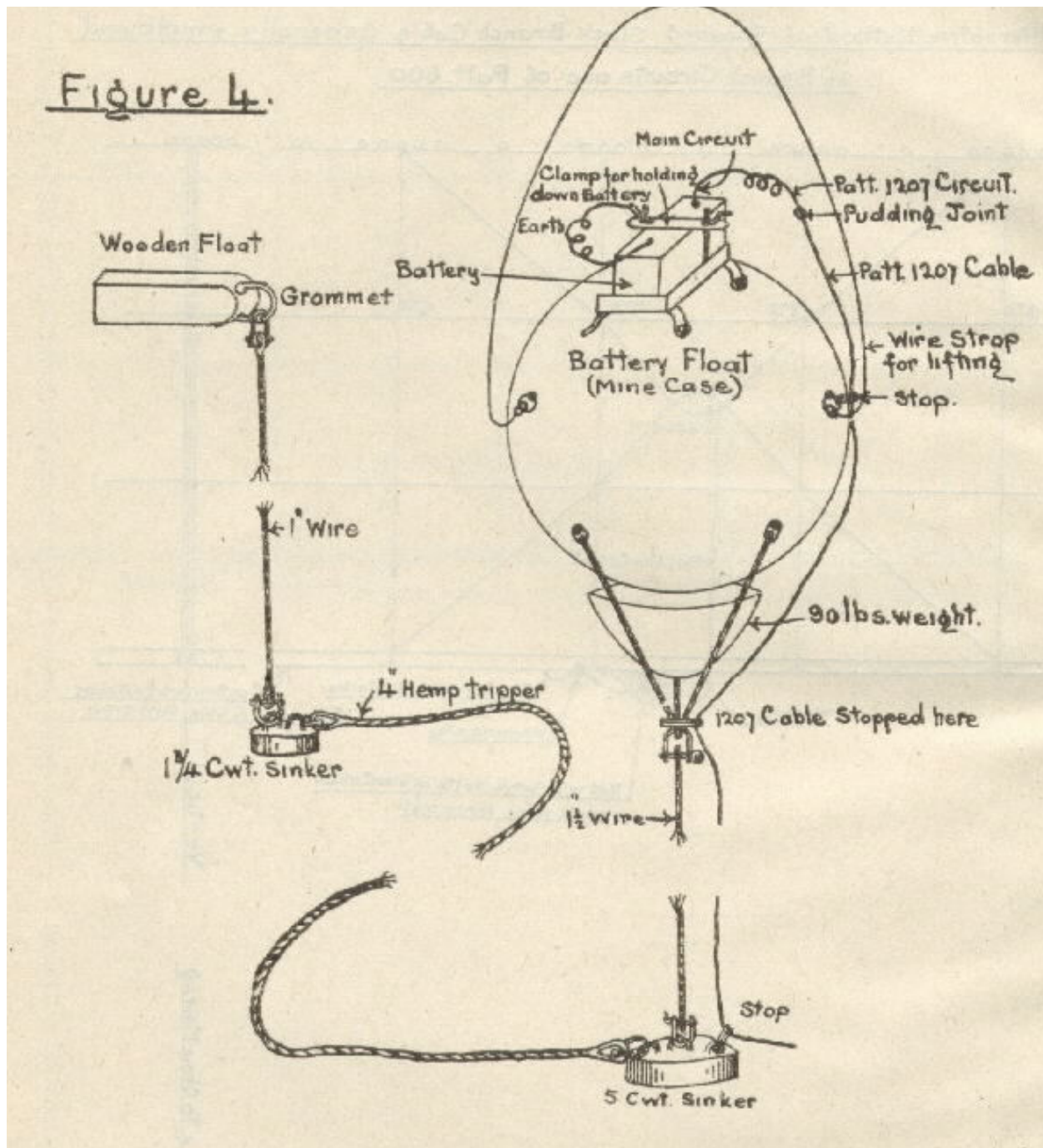
Image of figure 4: Arrangement of battery float and method of attaching Patt. 1207 cable.
