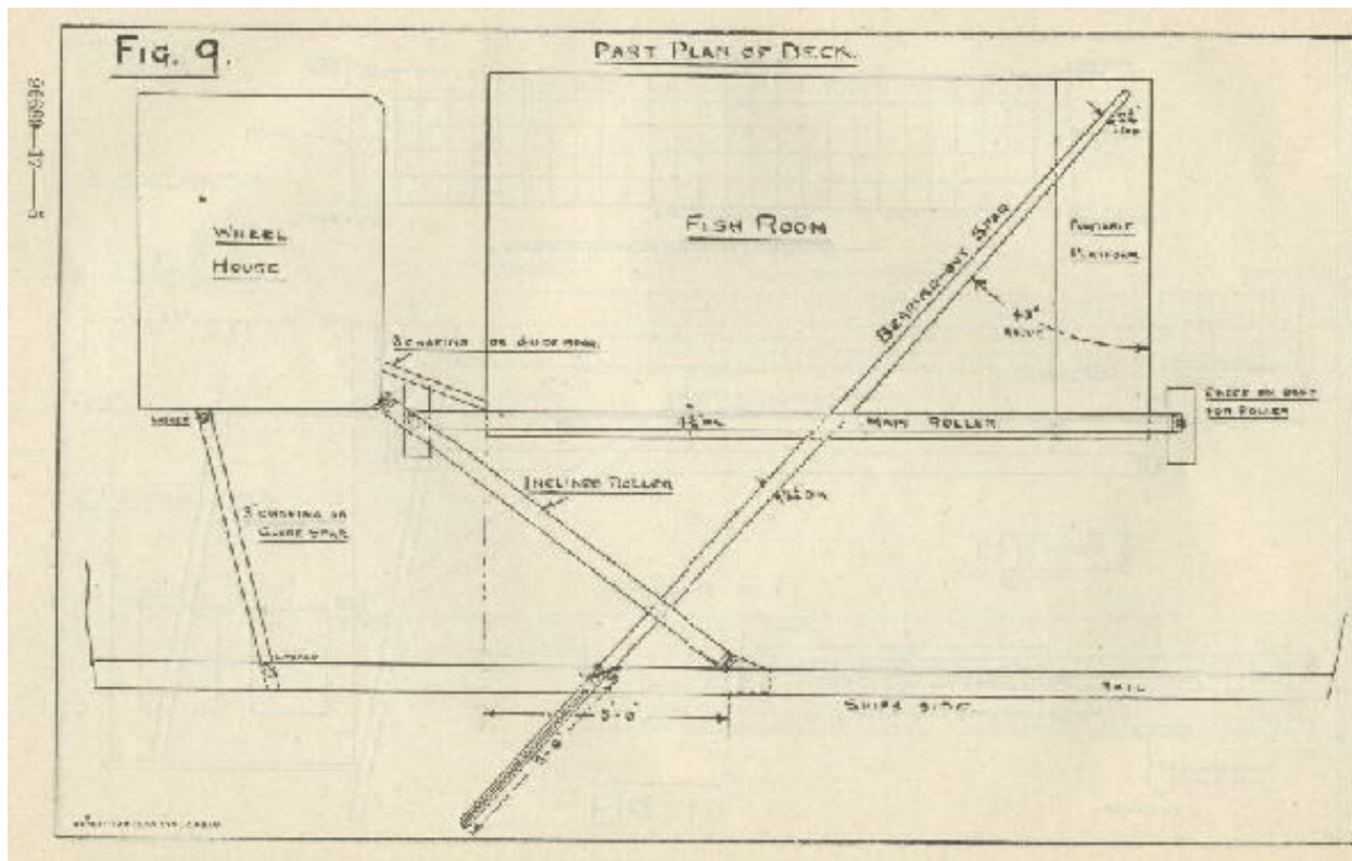
Image of figure 9: Part plans of deck.
