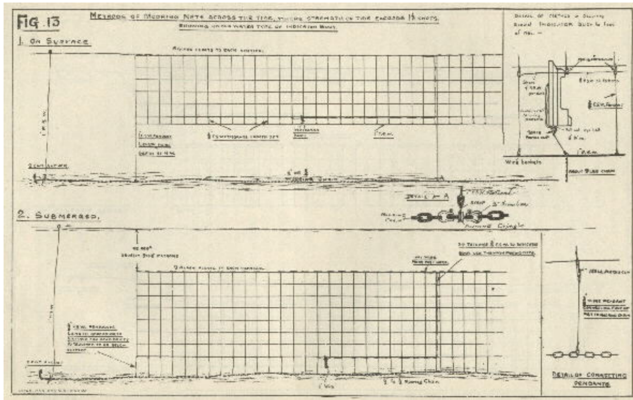
Image of figure 13: Methods of mooring nets across the tide, where strength of tide exceeds 1 1/2 knots. Showing underwater type of indicator buoy; 1. on surface, 2. submerged, and detail of connecting pendants.
