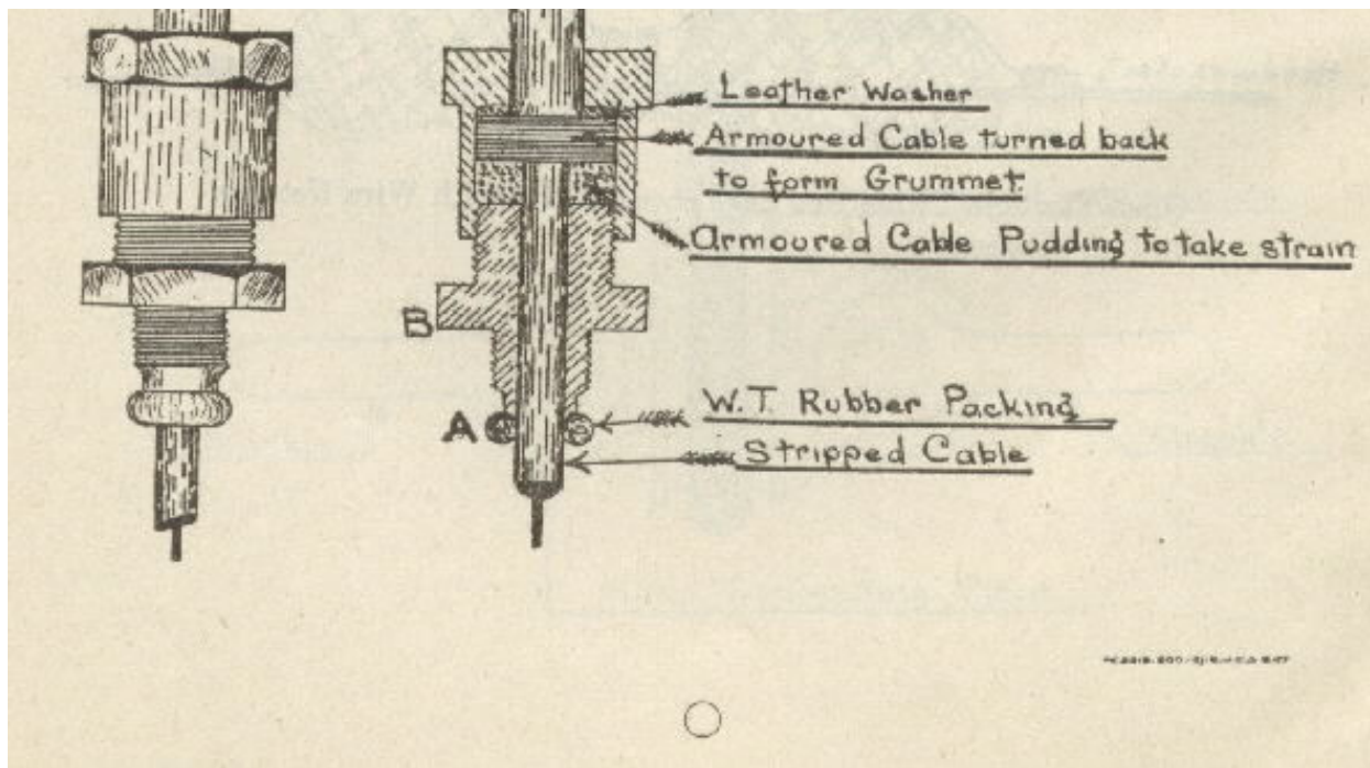
Image of figure 9: Sketch shewing arrangement of electric cable Patt. 1207. Large W.T. gland for Special E.C. mine.
