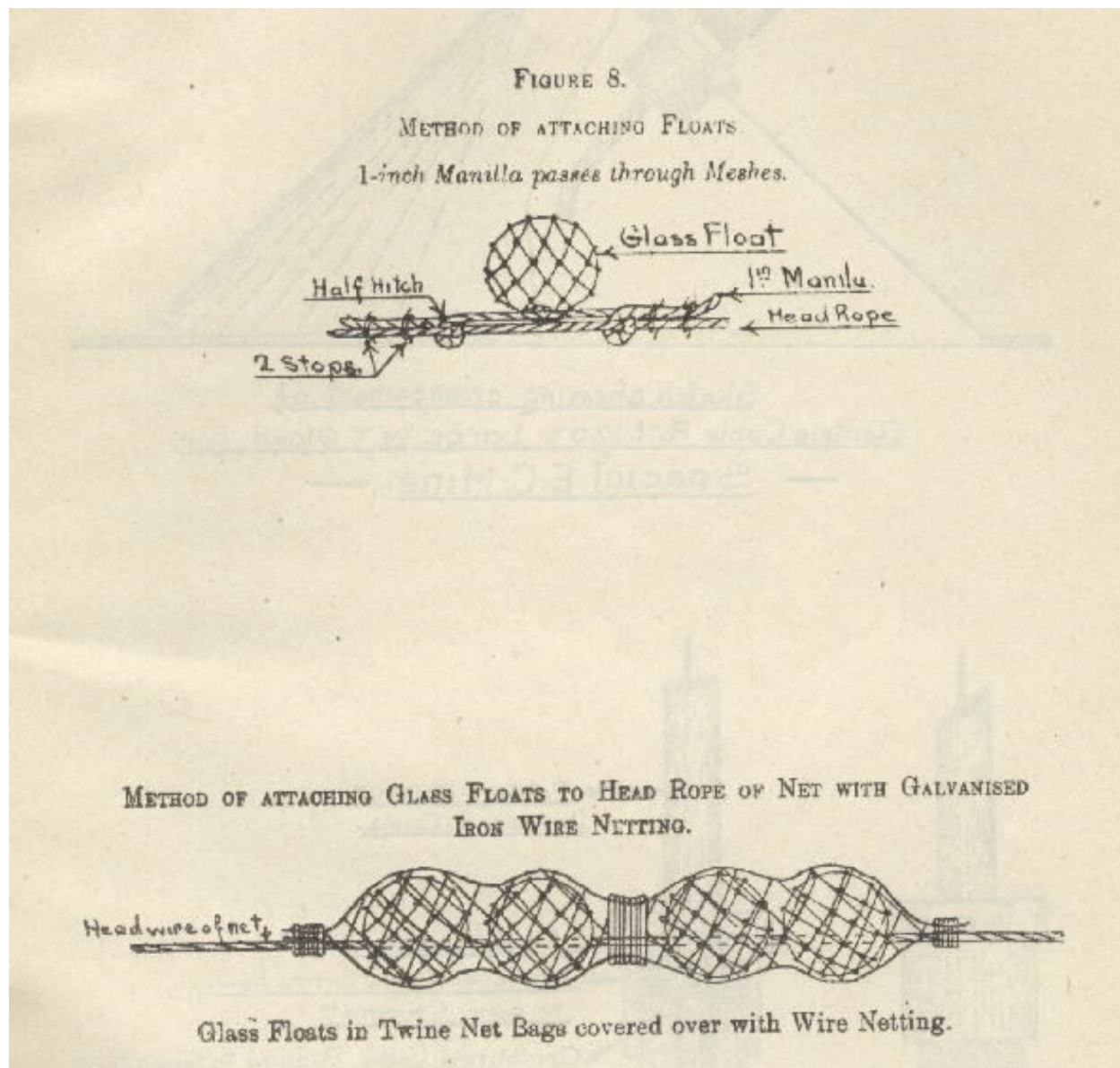
Image of figure 8: Method of attaching floats, and method of attaching glass floats to head rope of net with galvanized iron wire netting (glass floats in twine net bags covered over with wire netting).
