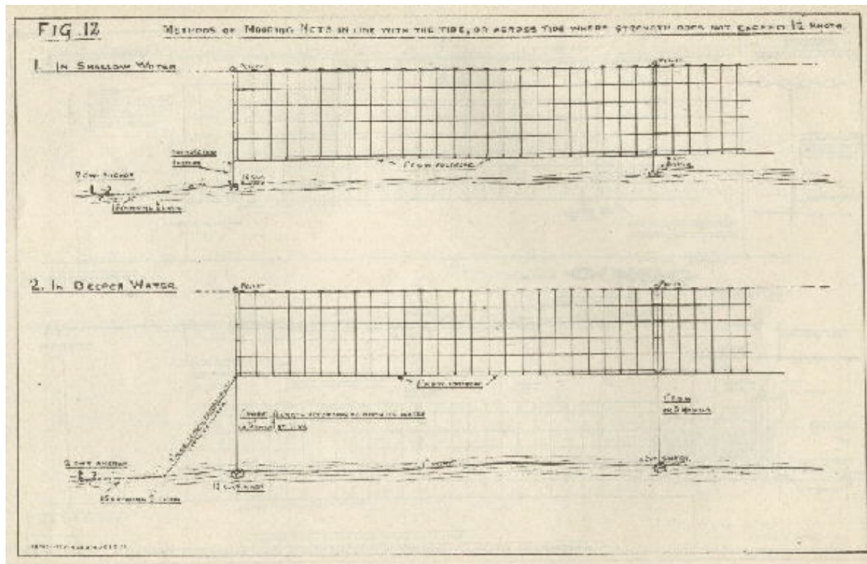
Image of figure 12: Methods of mooring nets in line with the tide, or across tide where strength does not exceed 1 1/2 knots; 1. in shallow water, 2. in deeper water.
