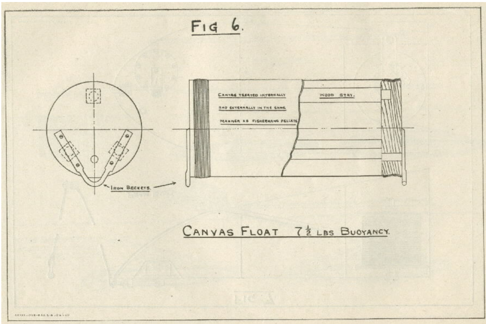
Image of figure 6: Canvas float 7 1/2 lbs. buoyancy.
