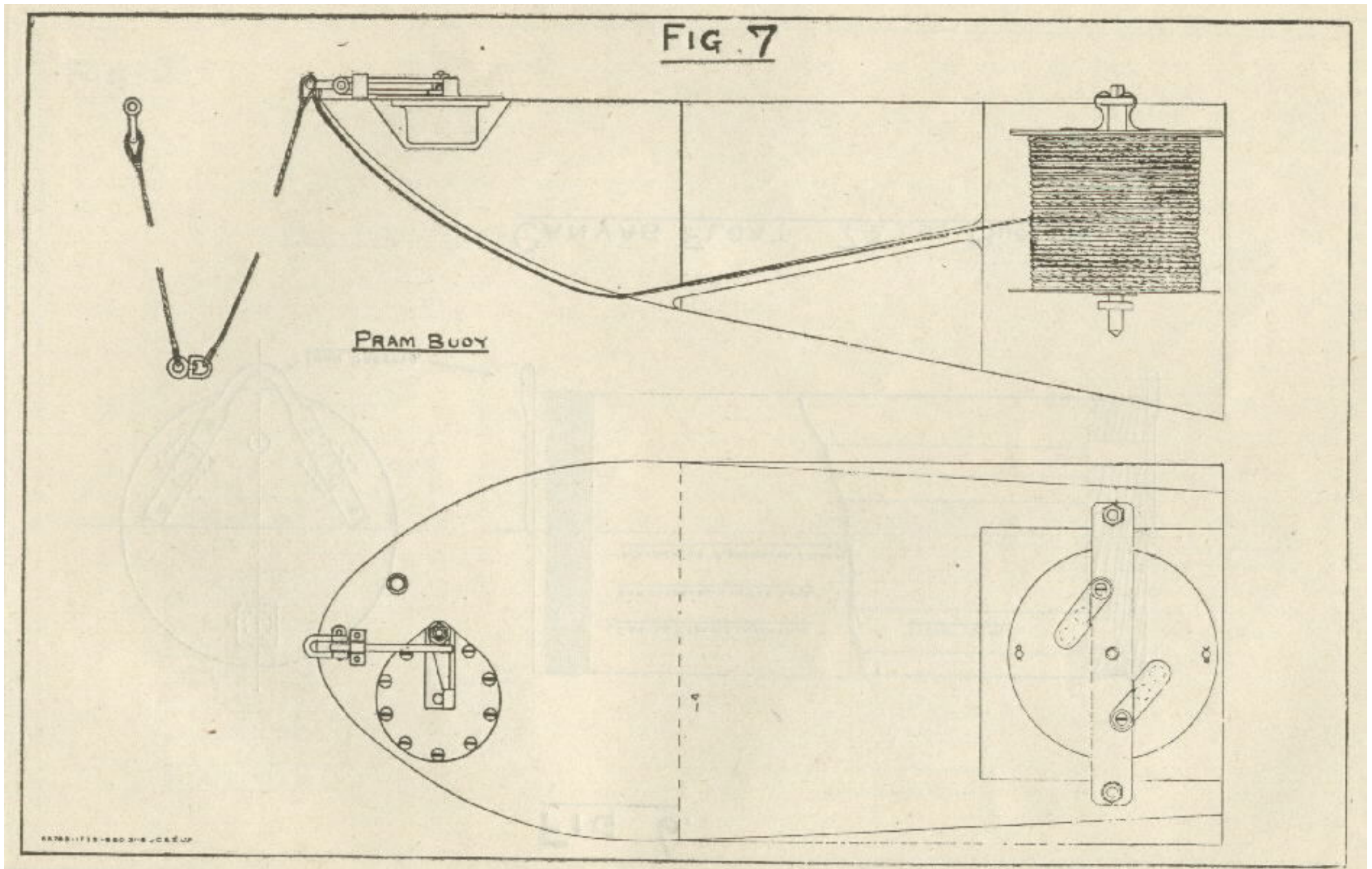
Image of figure 7: Pram buoy.
