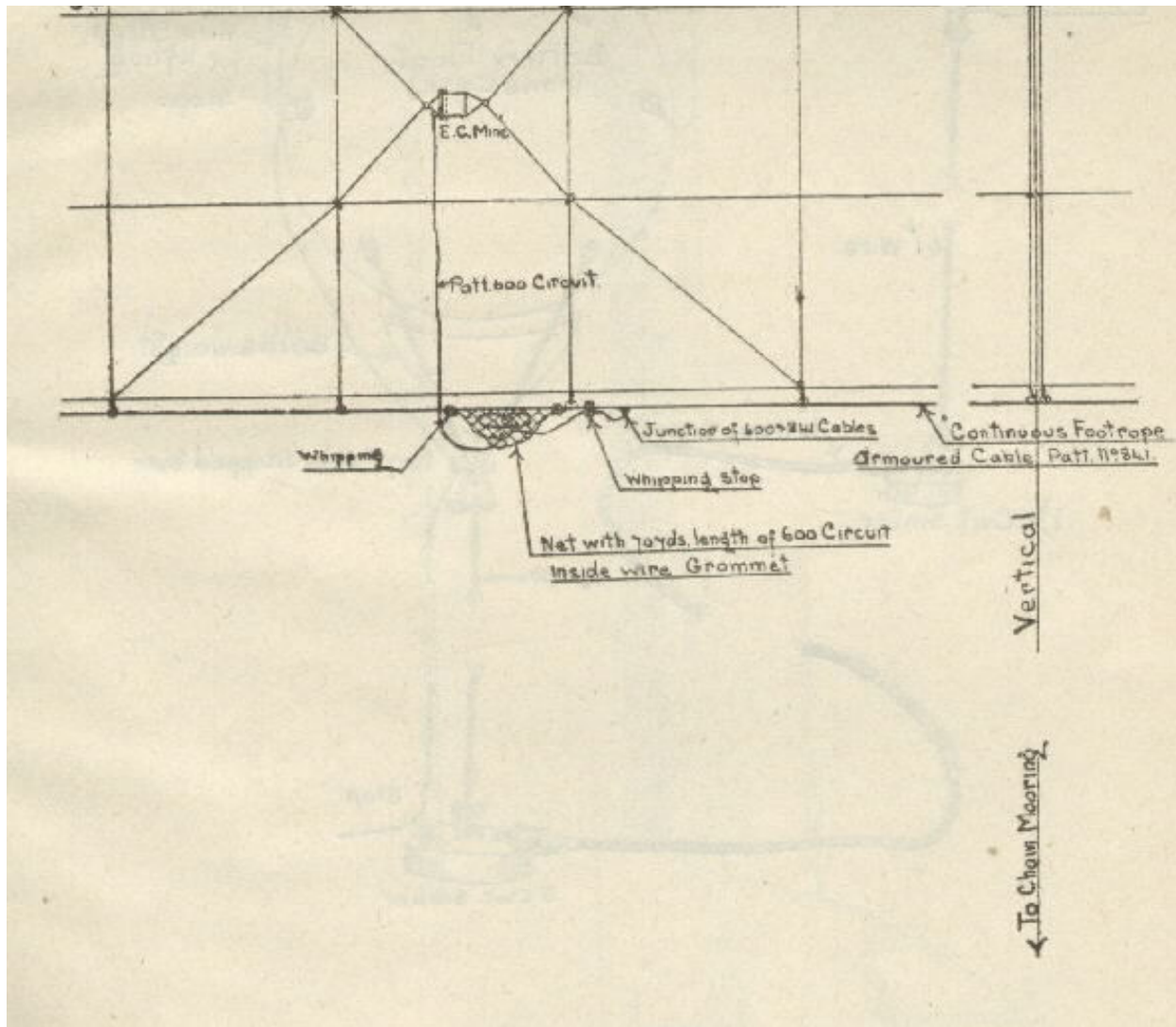
Image of figure 3: Alternative method of stowing slack branch cable generally employed if branch circuits are of Patt. 600.
