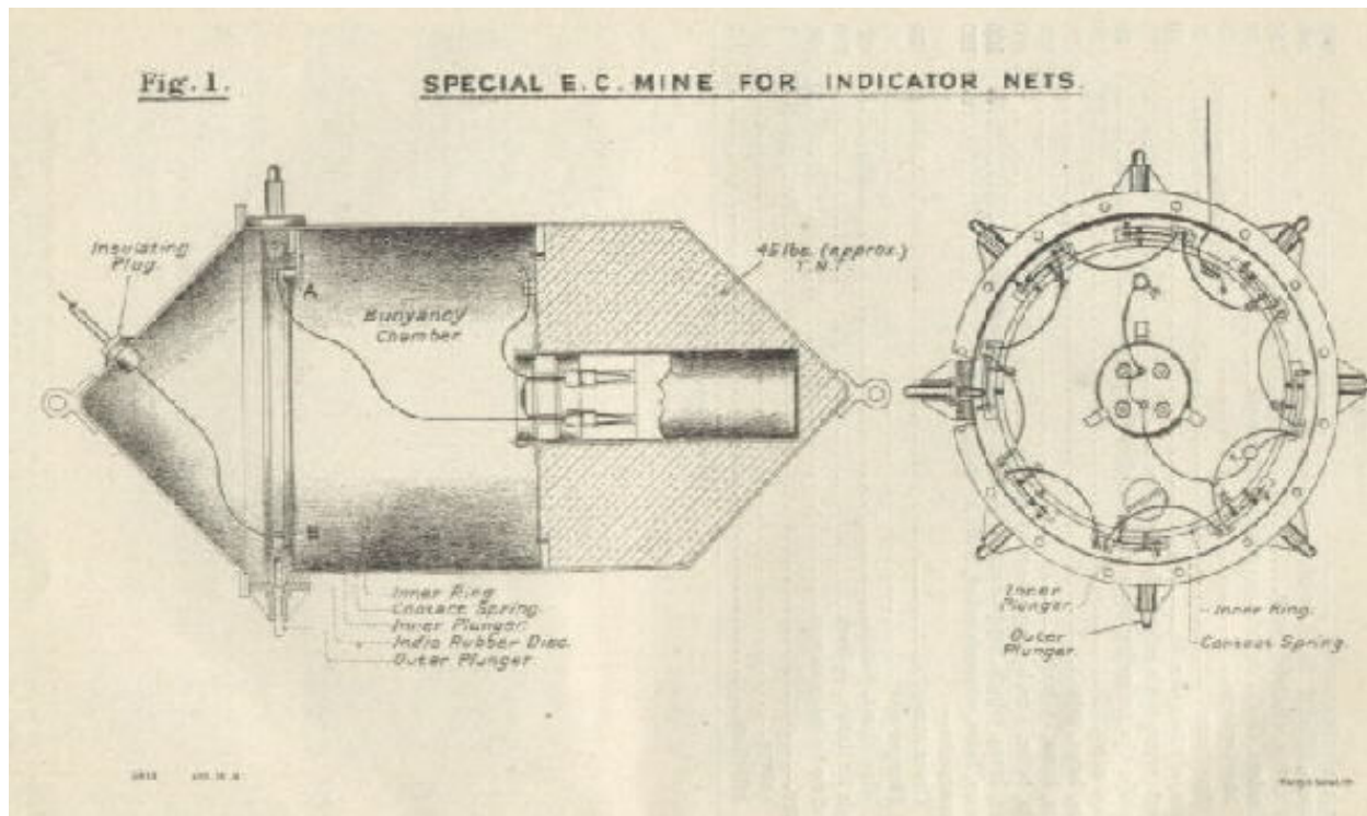
Image of figure 1: Special E.C. mine for indicator nets.
