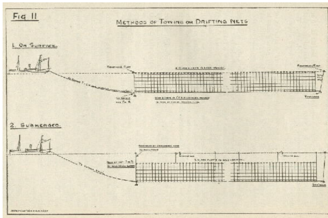
Image of figure 11: Methods of towing or drifting nets; 1. on surface; 2. submerged.
