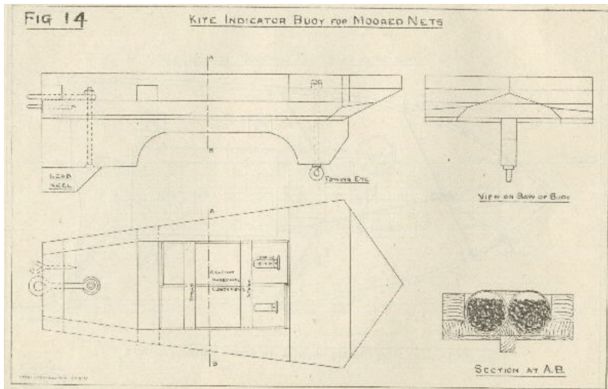
Image of figure 14: Kite indicator buoy for moored nets with view on bow of buoy and section at A.B.
