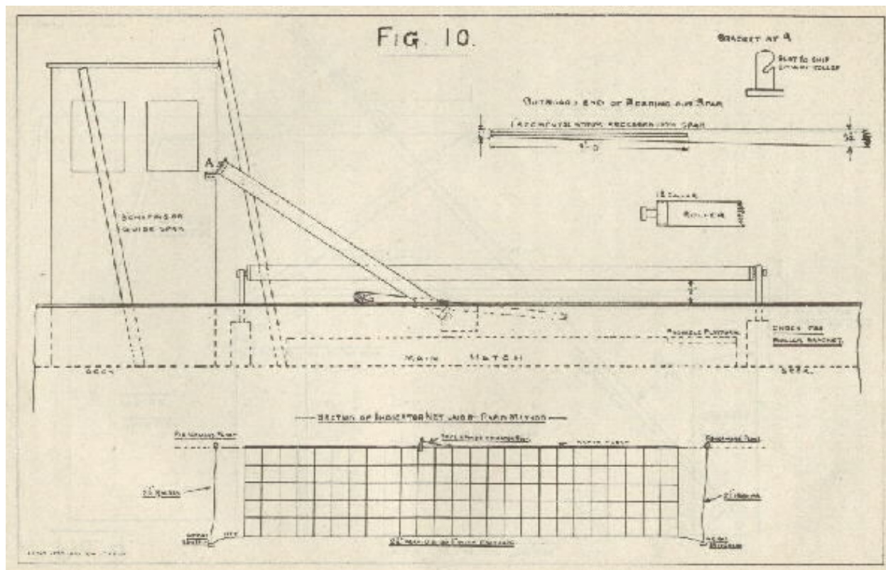
Image of figure 10: Outboard end of bearing-out spar and section of indicator net laid by rapid method.
