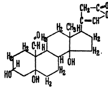
b Strophanthidin
