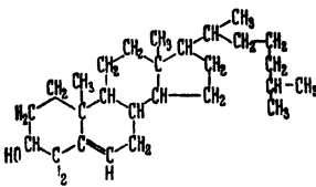
a Cholesterin
