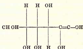
Common 1-2 dienol of D-glucose, D-mannose and D-fructose.
