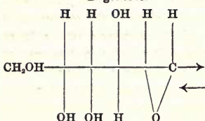
D-glucose.
