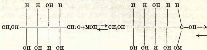
D-glucose.
