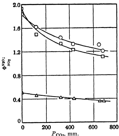
FIG. 30.—Effect of carbon dioxide in reducing the quantum yield \phi_{NO_2}^{NO_2} (corrected for screening by nitrogen tetroxide): \Delta —4,050, \circ —3,660, \square —3,130 Å.
