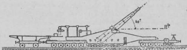
FIG 5.—Sliding-carriage pieces, 32-caliber gun.
