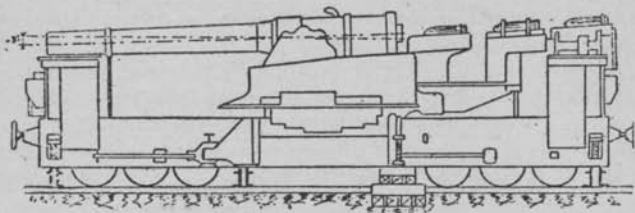
FIG. 2.—1870-1887 model 24-cm. gun on Batignolles truck mount. Fire in direction of the track (gun in loading position).
