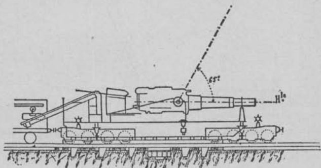
FIG. 8.—370-mm. howitzer.
