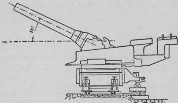
FIG. 3.—Fire in the direction perpendicular to the track. (Gun at the maximum angle of which it is capable, +30^{\circ} .)
