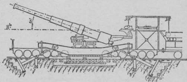
FIG. 6.—305-mm. gun on railway truck mount.
