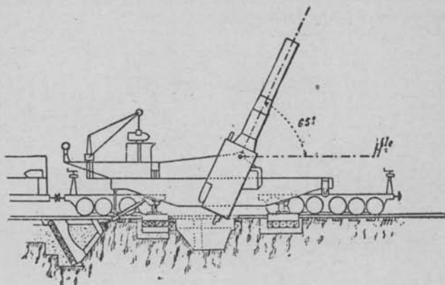
FIG. 9.—400-mm. howitzer.
