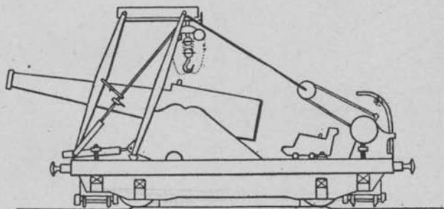
FIG. 10.—Rapid-fire 240-mm. gun on railway truck—Firing position.
