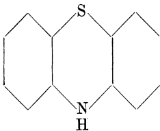
Thiodiphenylamin.
