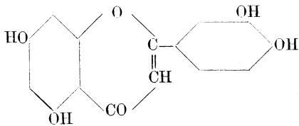
Luteolin (14).
