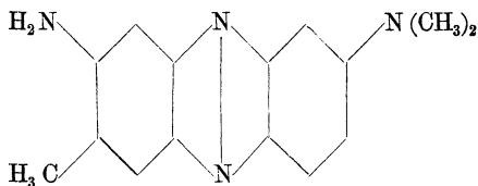
Toluylenroth (55).
