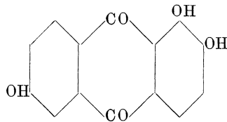
Flavopurpurin. 1:2:6.
