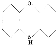
Phenoxazin.
