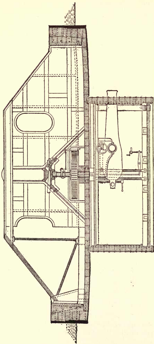
TRANSVERSE SECTION THROUGH TURRET OF ORIGINAL MONITOR
