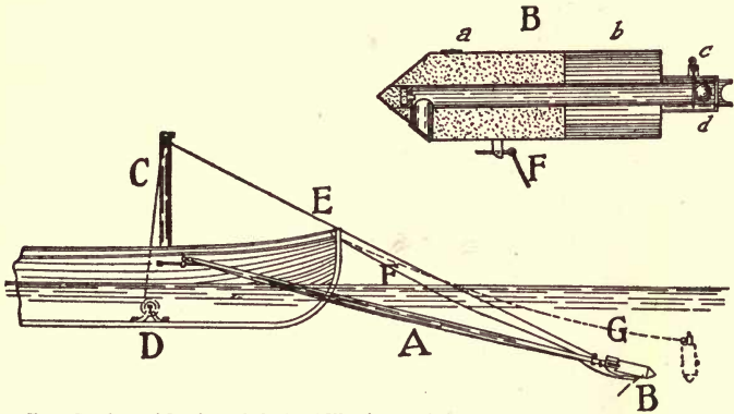
CUSHING'S LAUNCH AND TORPEDO
