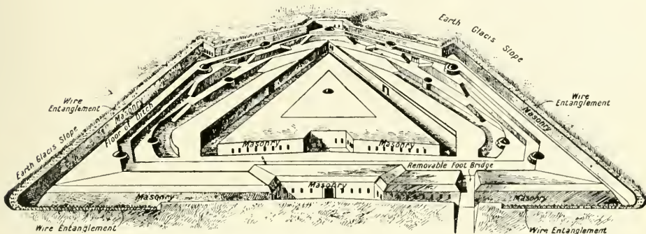
Pentagonal Brialmont fort.
