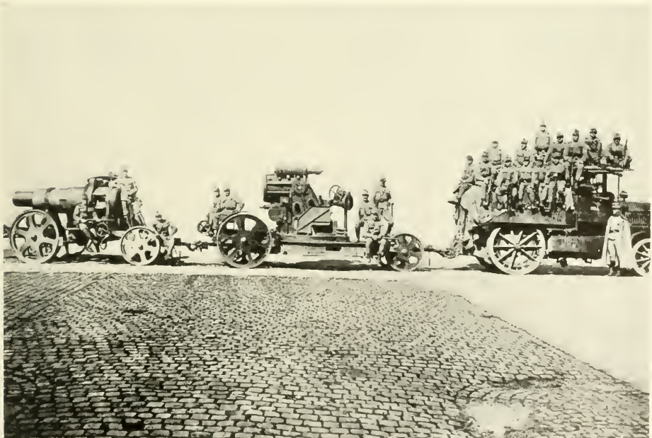
Siege gun used in the Austrian army. On the right is the motor-tractor, on the left, the gun, and in the center is the mount, which must be placed on a concrete base before the gun can be used.
