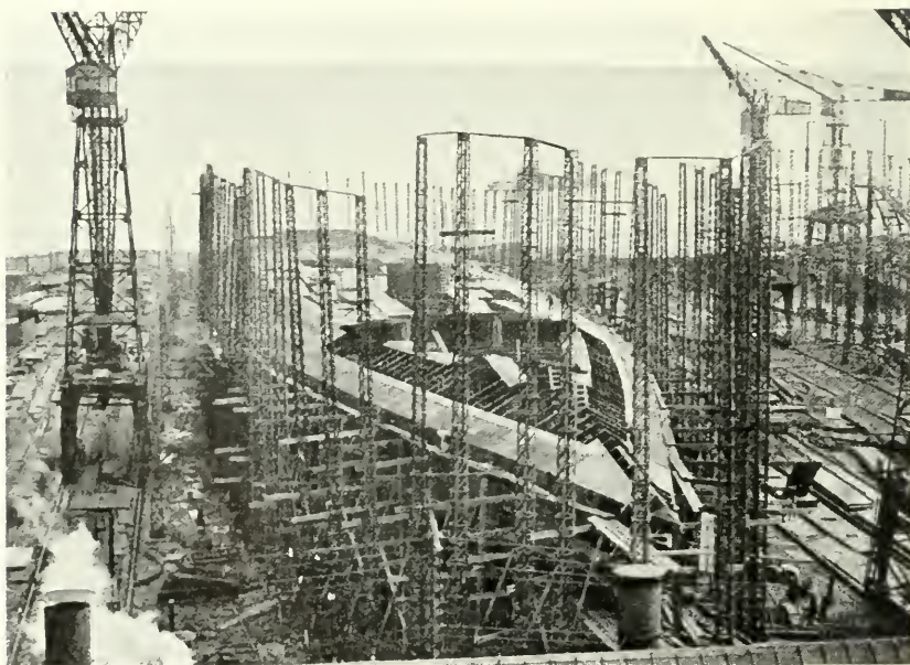
The French first class battleship Normandie in construction at Saint-Nazaire.
