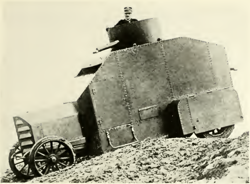
Italian armored automobile.
