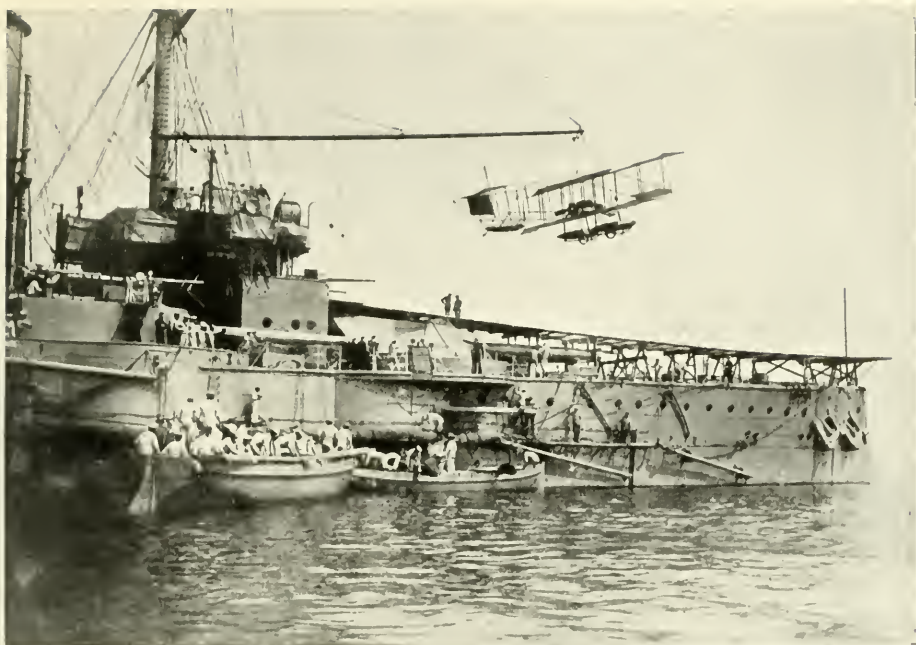
British warship with starting platform for aëroplane.
