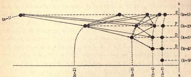
Diagram of the series spectrum of sodium.
