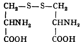
Cystin
