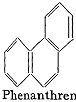
Phenanthren
