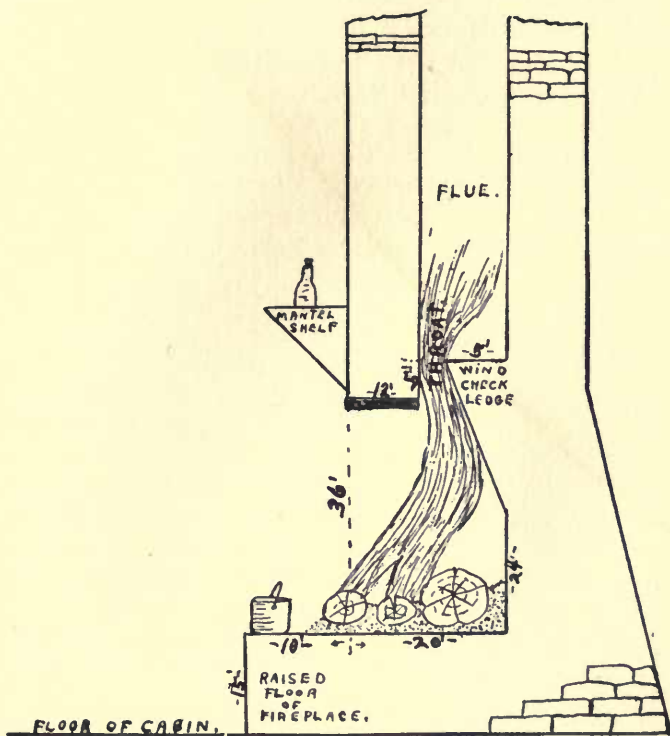
Fig. 6. DIAGRAM OF CONSTRUCTION OF FIREPLACE
