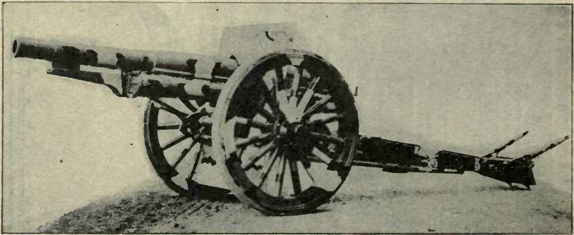
LEFT FRONT VIEW OF CARRIAGE EQUIPPED WITH BAND BRAKES.
