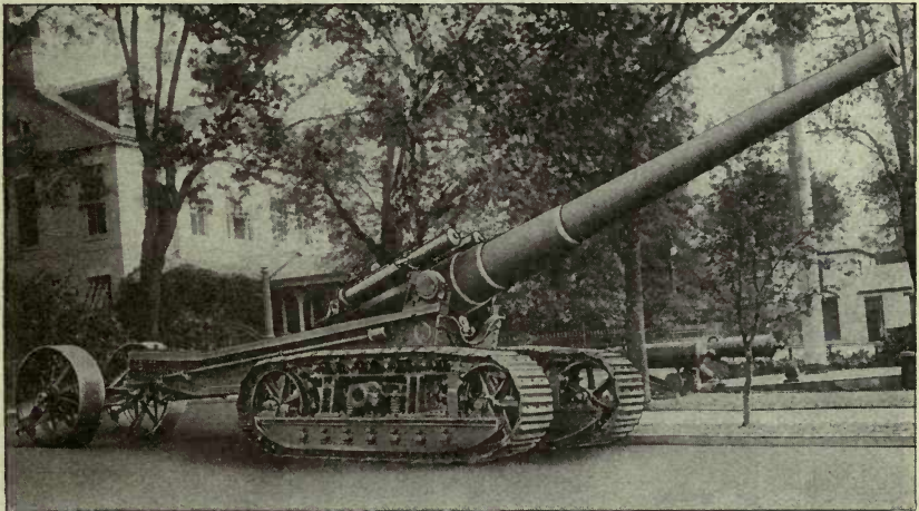
CARRIAGE AND LIMBER IN TRAVELING POSITION (REAR VIEW).
