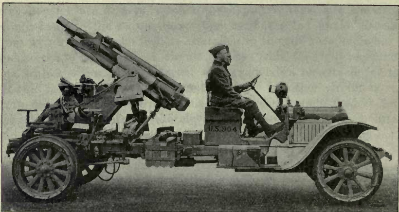
TRUCK IN TRAVELING POSITION (RIGHT SIDE VIEW).
