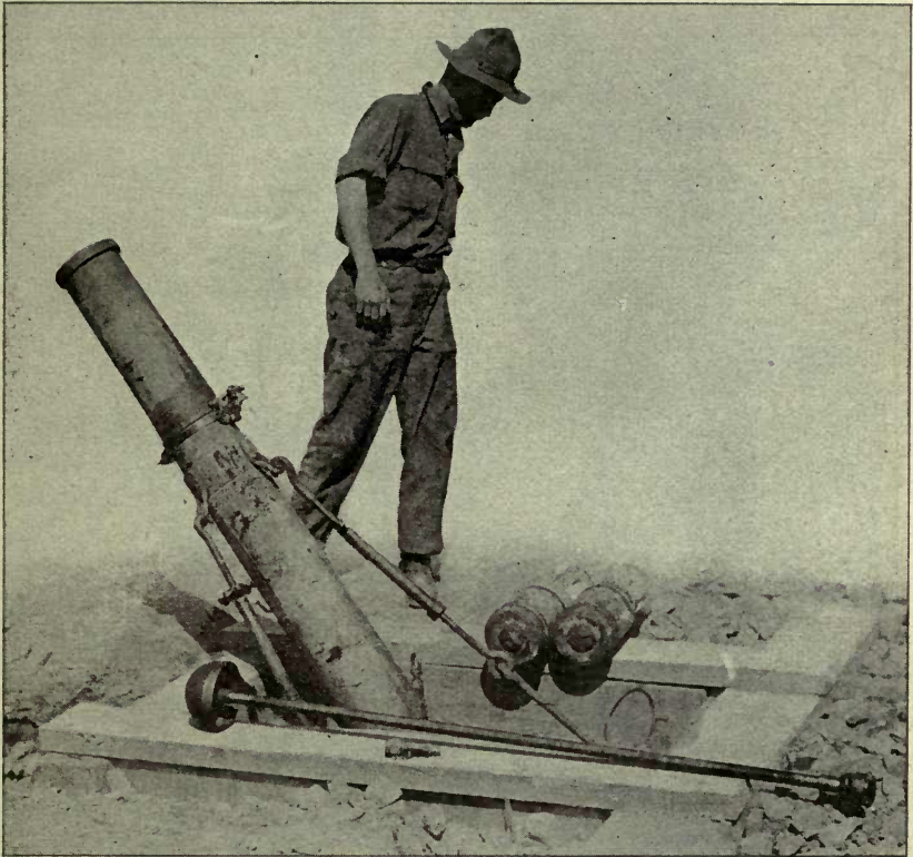
LEFT SIDE VIEW OF 6-INCH TRENCH MORTAR.
