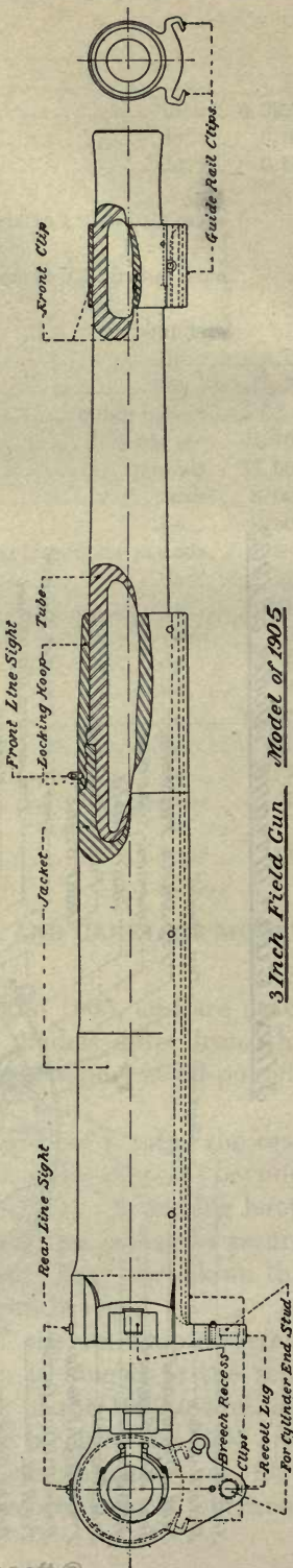
3 Inch Field Gun Model of 1904
