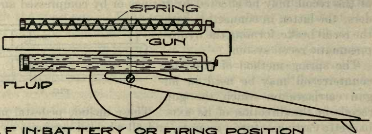
FIG. F IN BATTERY OR FIRING POSITION
