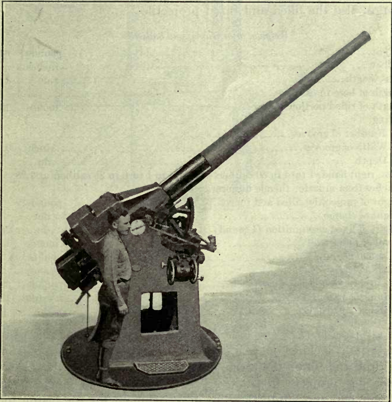
VIEW SHOWING RIGHT SIDE OF MOUNT.
