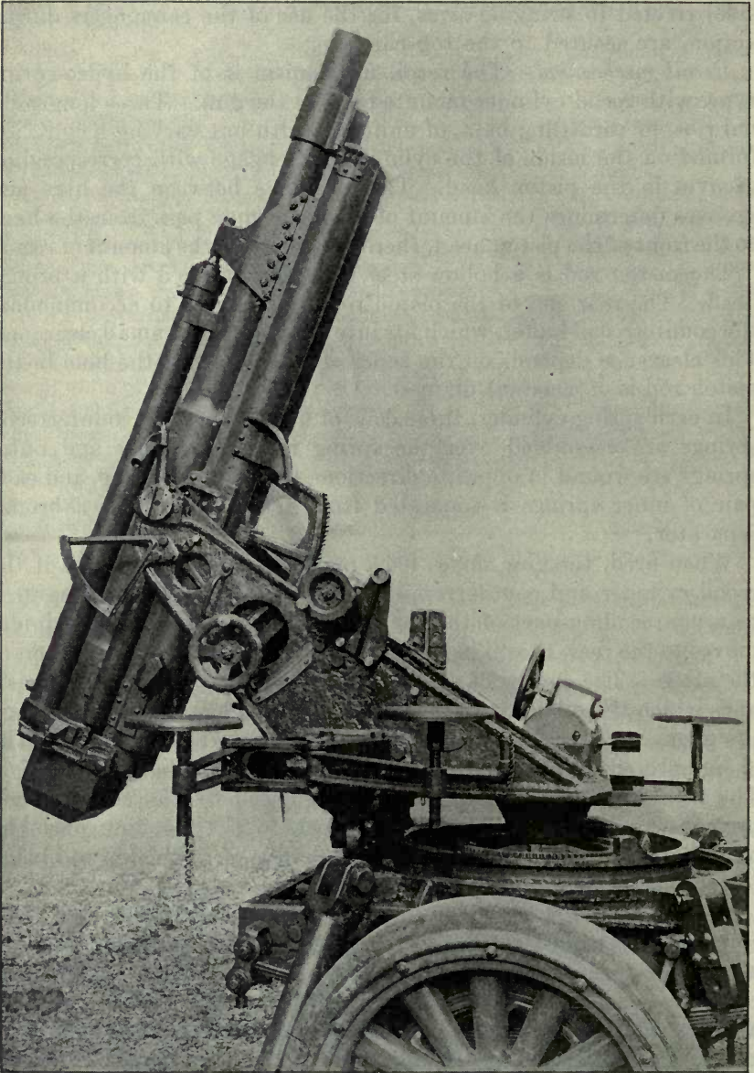
GUN MOUNT SHOWING GUN AT MAXIMUM ELEVATION.
