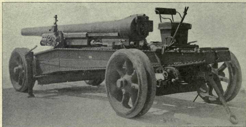
FRONT VIEW OF LIMBER EN ROUTE.
