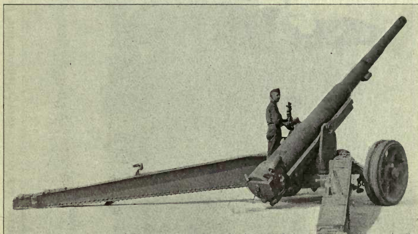
CARRIAGE IN FIRING POSITION.
