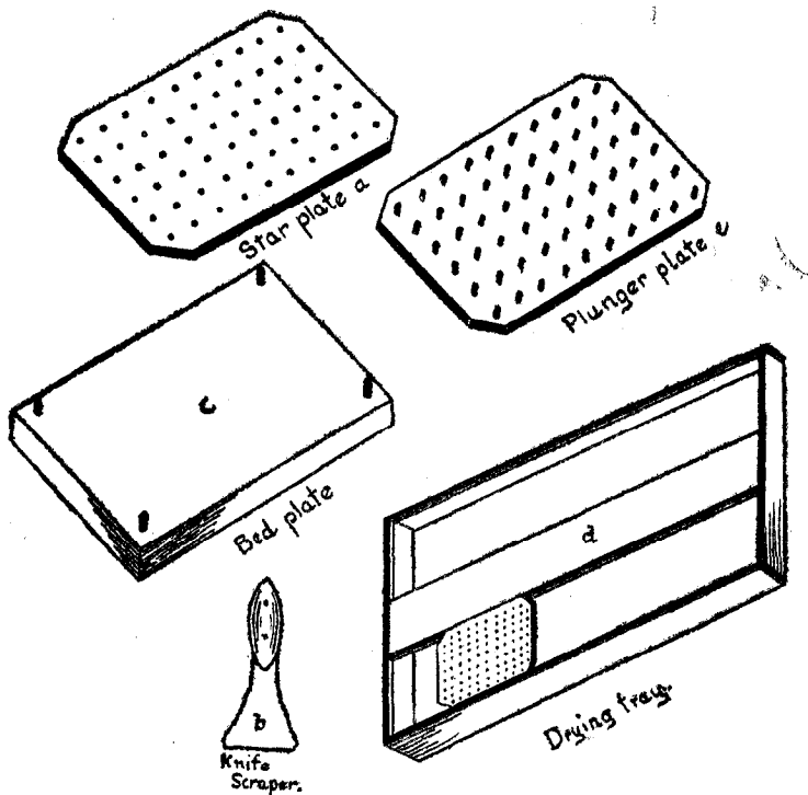
Star plate assembly Fig. 55.
