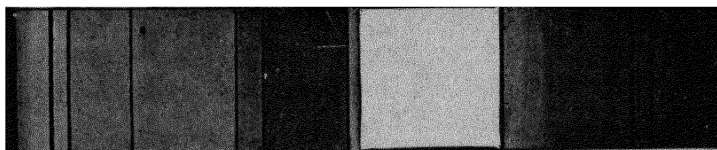
Fig. 8.—Spectrum Reflected From Blue Silk.
