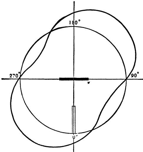
Fig. 30.—Distribution of Light from Flat Filament.
