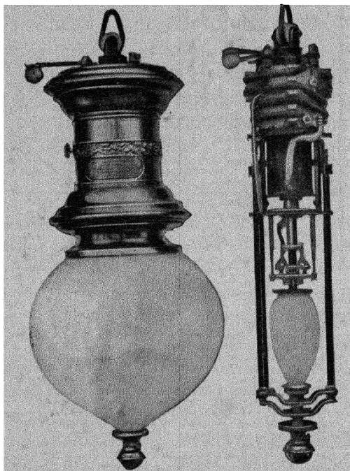
Fig. 48.—Typical Enclosed Arc Lamp.
