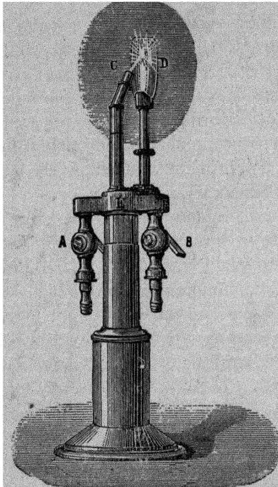
Fig. 25. Oxy-hydrogen burner.
