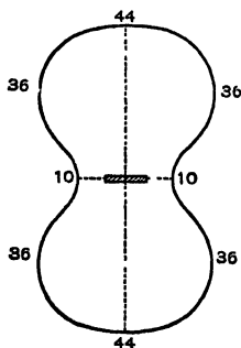
Fig. 44.—Horizontal Distribution from Nernst Lamp.
