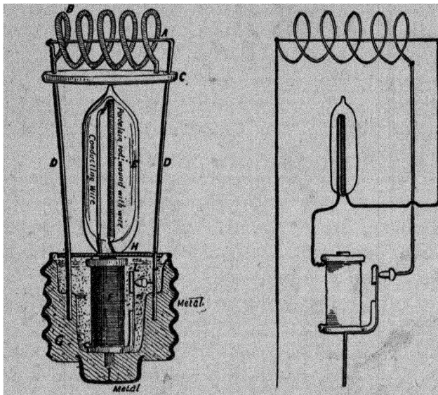
Fig 39 and 40.—Connections of Nernst Lamp.
