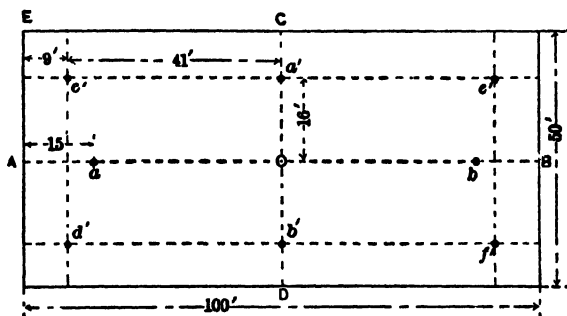
Fig 89.—Plan of Hall
