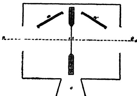
Fig. 121.—Bunsen Photometer Screen.
