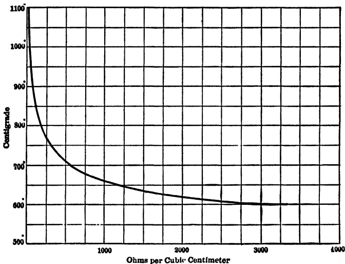
Fig. 38.—Curve of Resistance Variation.
