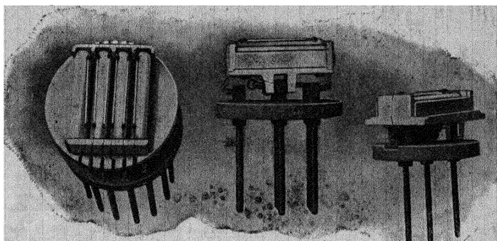
Fig. 42.—Glowers and Heaters of American Nernst Lamp.
