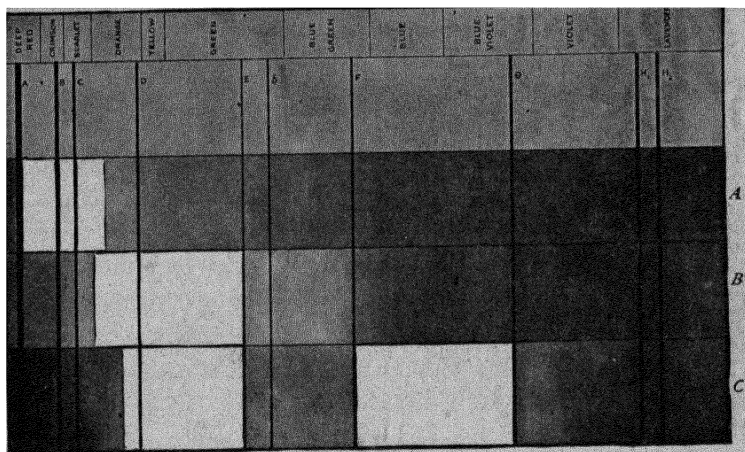
Fig. 7.—Solar and Reflected Spectra.
