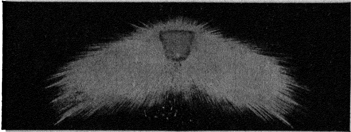
Fig. 76.—Holophane, Outward Distribution.
