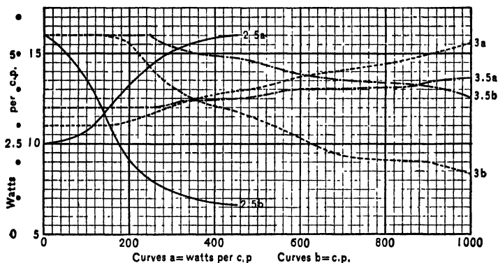
Fig. 36.—Curves Showing Life, Candle-power and Watts per Candle.
