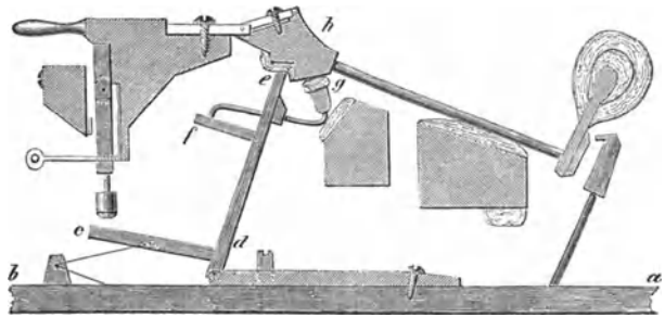
Fig. 508. Repetitionsmechanik.
