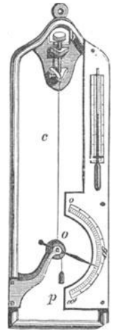
Fig. 554. Saure'sches Saurehygrometer.
