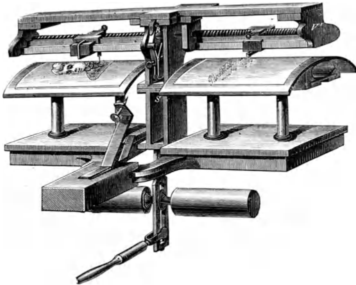
Fig. 434. Casellis Pantelegraph.
