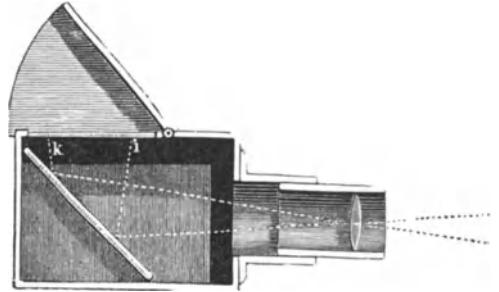
Fig. 258. Transportable Camera obscura.
