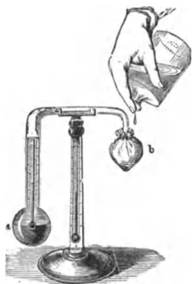
Fig. 555. Daniell's Hygrometer.
