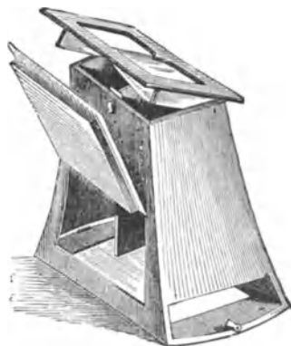
Fig. 281. Wheatstone'sches Prismenstereoskop.
