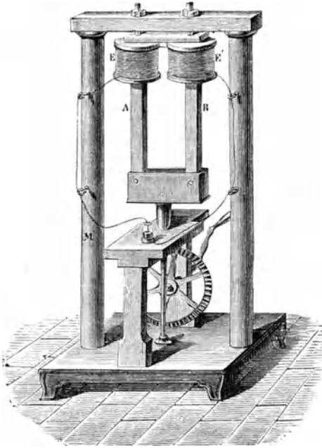
Fig. 394. Poggendorff's Rotationsmaschine.
