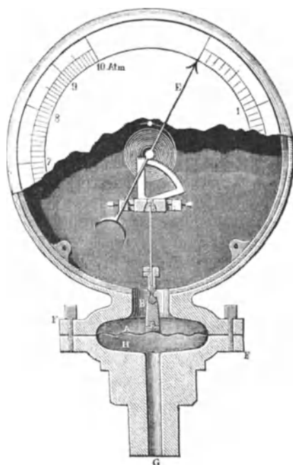
Fig. 108. Schäffer's Metallmanometer.
