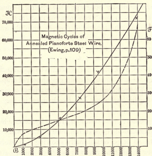
FIG. 38.—CURVE OF HYSTERESIS OF ANNEALED PIANOFORTE STEEL WIRE.
