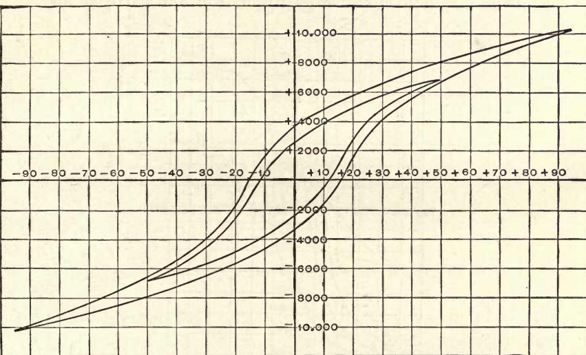
FIG. 32.—MAGNETIC CYCLES OF CAST-IRON.
