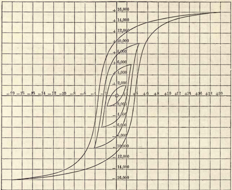
FIG. 31.—MAGNETIC CYCLES OF SOFT SHEET-IRON OR SHEET-STEEL.
