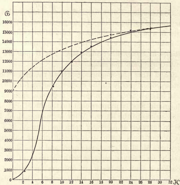
FIG. 29.—RISING AND DECREASING MAGNETIC CHARACTERISTIC.
