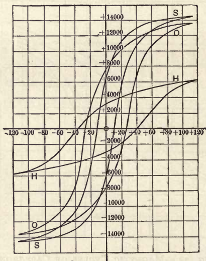
FIG. 33.—MAGNETIC CYCLES OF WELDED STEEL AT DIFFERENT DEGREES OF HARDNESS.
