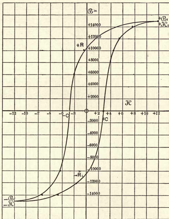
FIG. 30.—HYSTERETIC LOOP OR MAGNETIC CYCLE.
