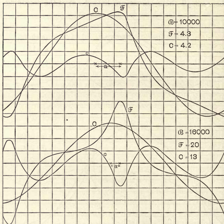
FIGS. 41 AND 42.—DISTORTION OF CURRENT WAVE BY HYSTERESIS.
