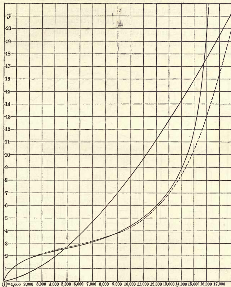
FIG. 35.—MAGNETIC CHARACTERISTIC FROM BALLISTIC AND ALTERNATING CURRENT TESTS, AND MOLECULAR MAGNETIC FRICTION CURVE.
