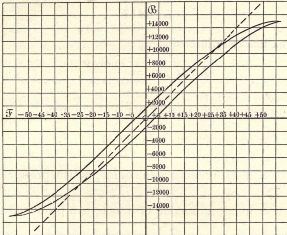
FIG. 34.—MAGNETIC CYCLE OF CIRCUIT CONTAINING AN AIR-GAP.
