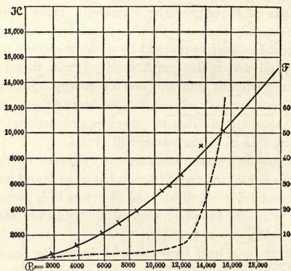
FIG. 37.—CURVE OF HYSTERESIS OF SOFT IRON WIRE.
