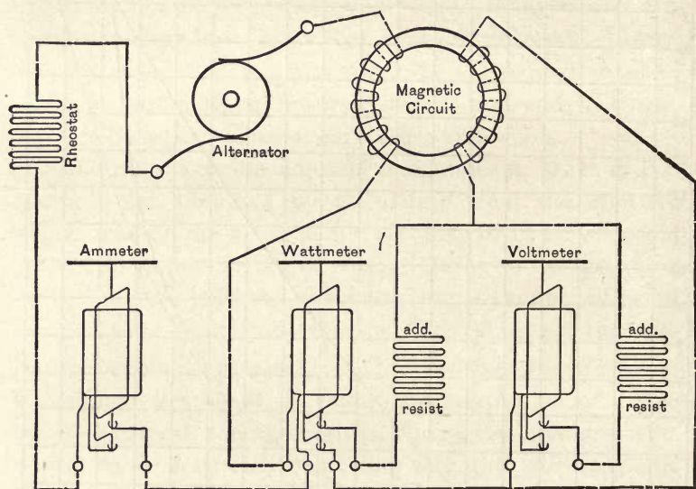
FIG. 36.—INSTRUMENT CONNECTIONS FOR ALTERING CURRENT HYSTERESIS TESTS.
