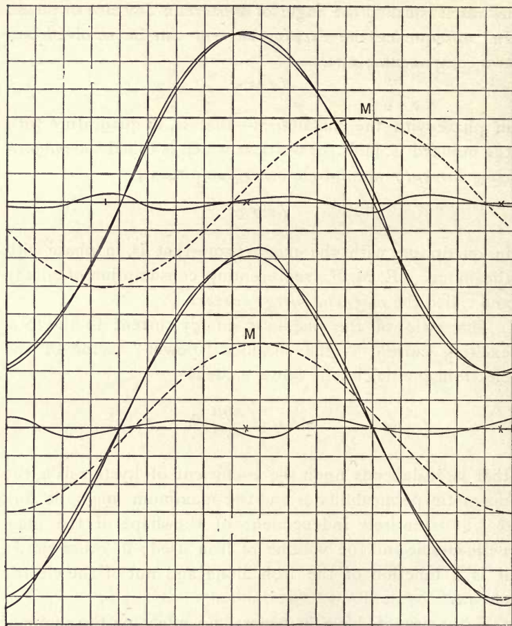
FIGS. 43 AND 44.—DISTORTION OF CURRENT WAVE BY HYSTERESIS.
