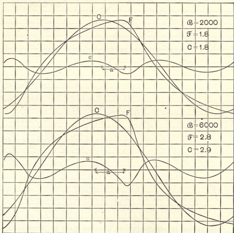
FIGS. 39 AND 40.—DISTORTION OF CURRENT WAVE BY HYSTERESIS.
