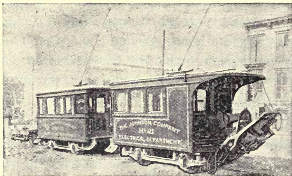
FIG. 74.—TRACK-WELDING CAR.
