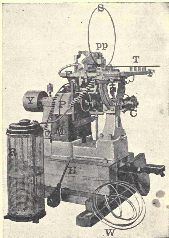
FIG. 59.—DIRECT-WELDING APPARATUS.
