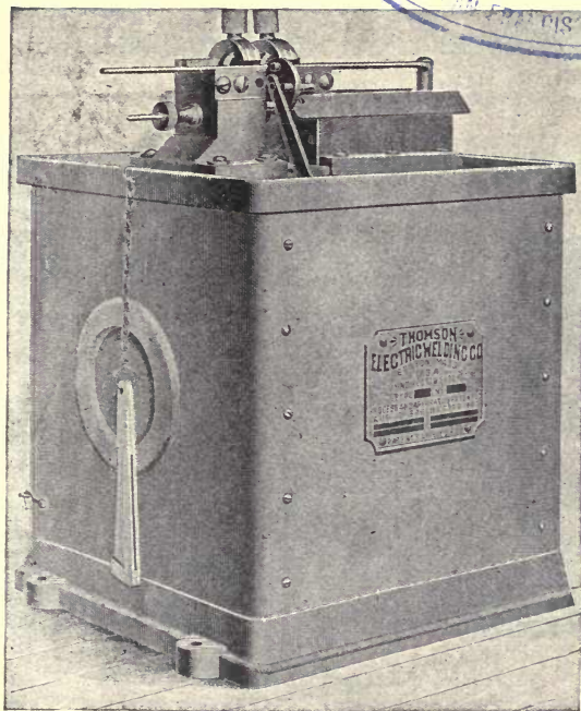
FIG. 65.—AUTOMATIC WELDER.
