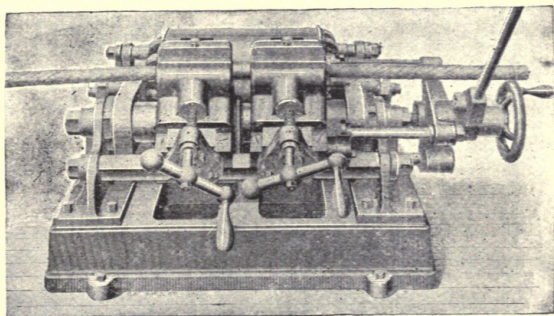
FIG. 69.—WELDER FOR CABLE OR BARS.
