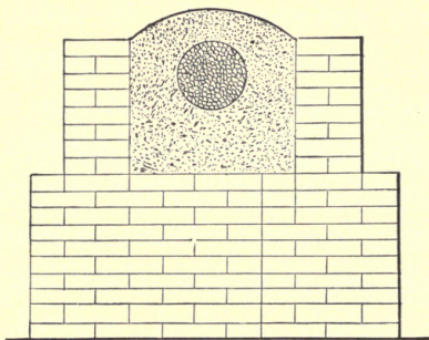
FIG. 79.—SECTION THROUGH FURNACE BEFORE PASSAGE OF CURRENT.
