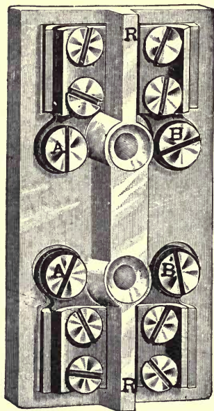
FIG. 11.—PORCELAIN FUSE-BOX.
