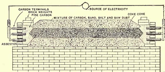
FIG. 78.—LONGITUDINAL SECTION OF CARBORUNDUM FURNACE.
