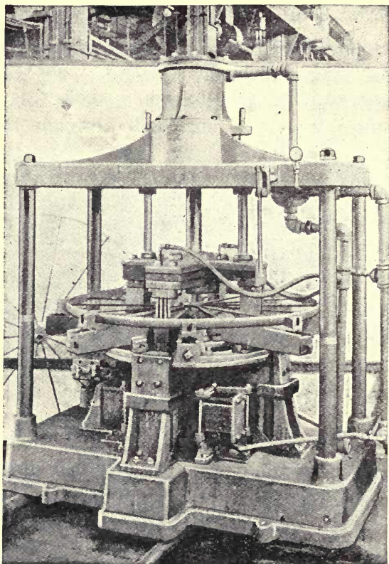
FIG. 70.—WELDER FOR WHEEL-SPOKES.
