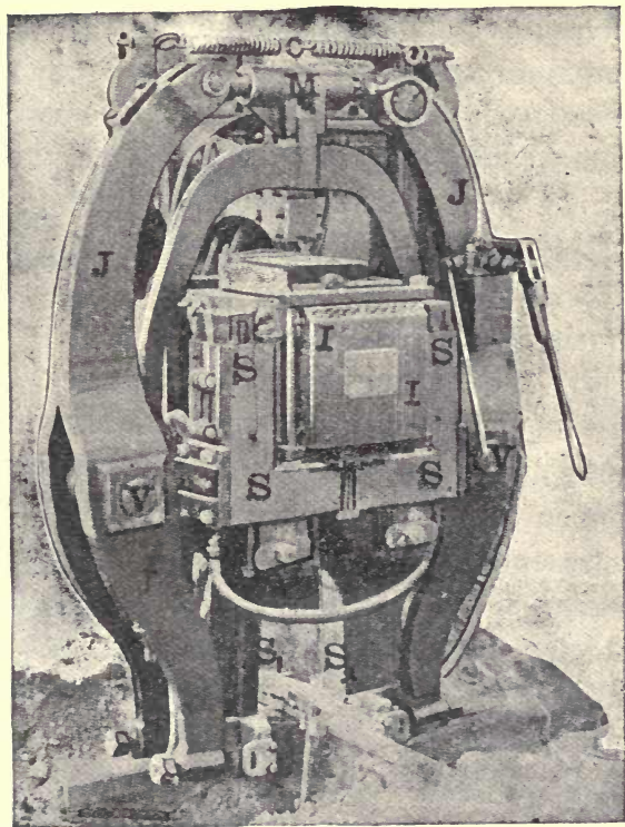
FIG. 75. —TRACK WELDER AT WORK.
