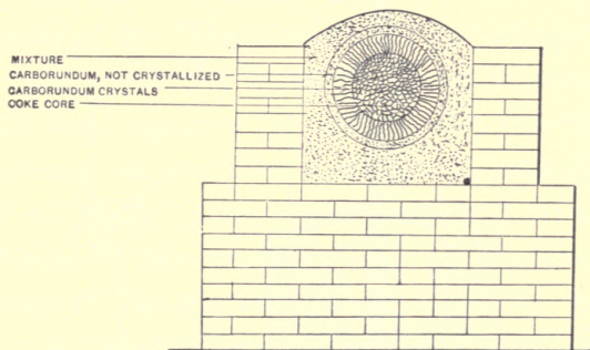
FIG. 80.—SECTION THROUGH FURNACE AFTER PASSAGE OF CURRENT.
