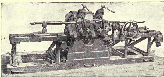
FIG. 68.—WELDER FOR CARRIAGE AXLES.
