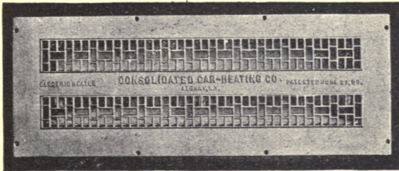
FIG. 23.—ELECTRIC CAR-HEATER.
