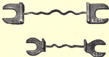
FIG. 7.—COPPER-TIPPED FUSE WIRES.
