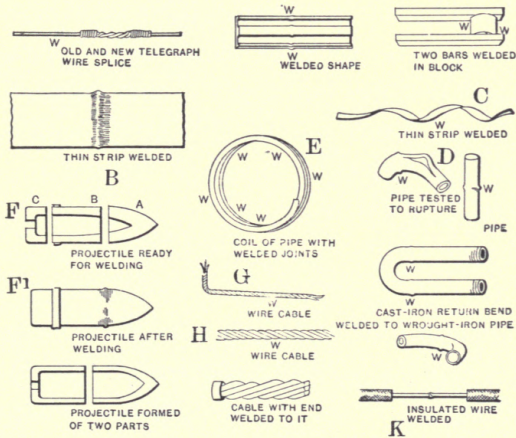
FIG. 71.—SPECIMENS OF ELECTRIC WELDING.
