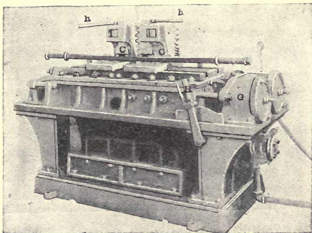
FIG. 67.—UNIVERSAL WELDER.
