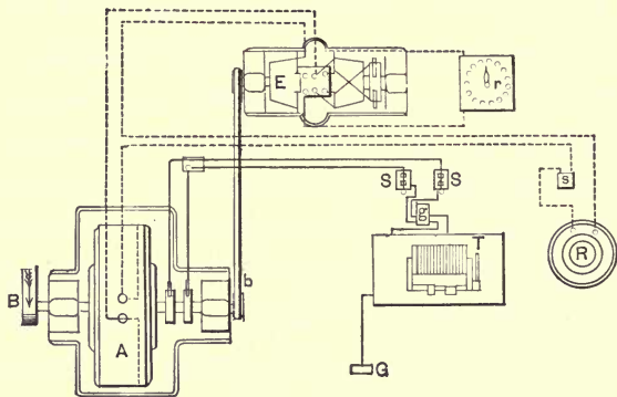
FIG. 60. — CONNECTIONS OF INDIRECT WELDING.
