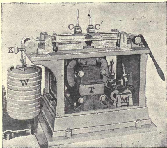
FIG. 64.—AUTOMATIC WELDER.
