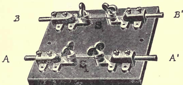
FIG.10.—PAIR OF SAFETY STRIPS, MOUNTED ON FUSE-BLOCK. and B, B' . The two supply mains A and B are electrically separated from each other by the porcelain projecting ridge RR , provided for this purpose. The pressure between these leads may be 100 or 200 volts, according to circumstances, and
