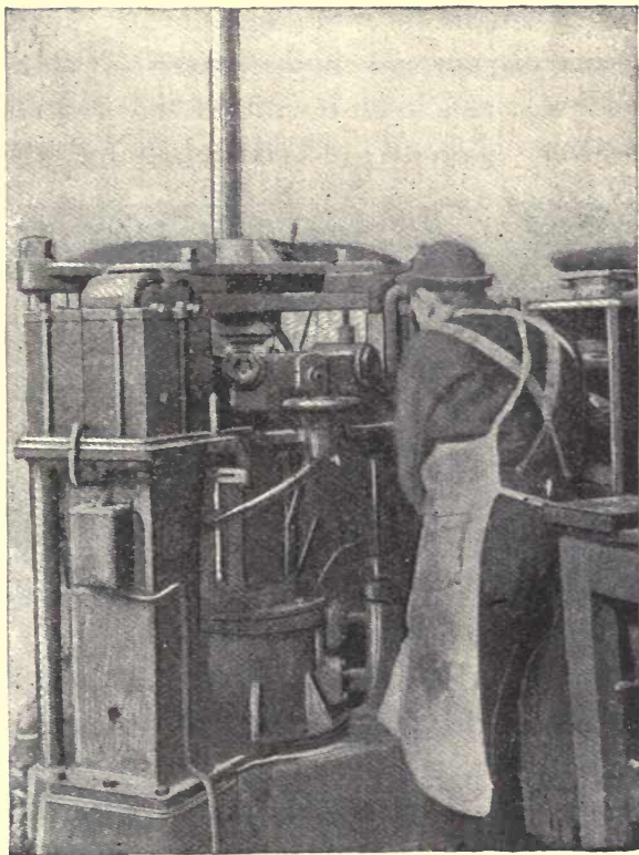
FIG. 72.—WELDER FOR SHRAPNEL SHELLS.
