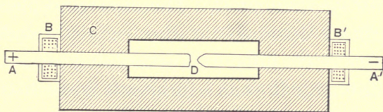
FIG. 82. —ELECTRIC FURNACE FOR THE PRODUCTION OF ALUMINIUM ALLOYS.
