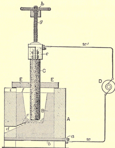
FIG. 81.—FURNACE FOR PRODUCTION OF CALCIUM CARBIDE.
