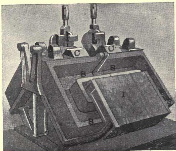
FIG. 62.—WELDING TRANSFORMER.
