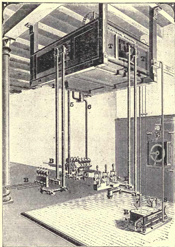
FIG 83.--ELECTRIC FORGE AND ELECTRIC COOKING RANGE.
