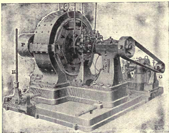
FIG. 61.—CONSTANT POTENTIAL DYNAMO.
