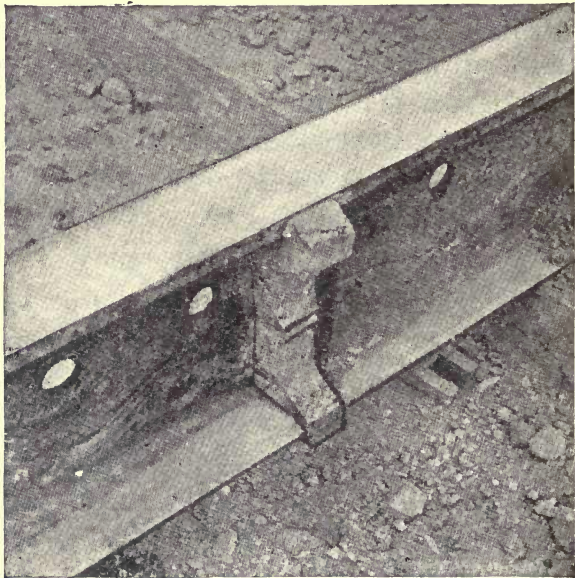
FIG. 76.—WELDED RAILS.
