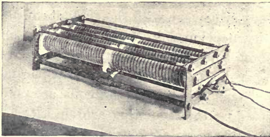
FIG. 38 —TANK HEATER.
