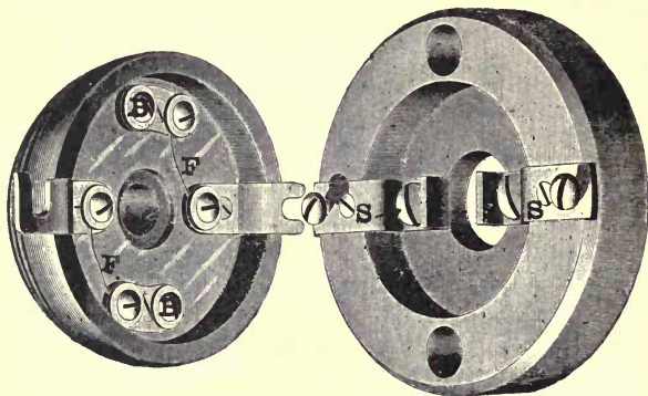
FIG. 16.—CEILING-FIXTURE FUSE-BLOCK.
