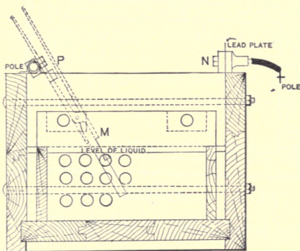
FIG. 85.—END VIEW OF HEATING TANK.
