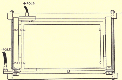
FIG. 86. —PLAN OF HEATING TANK.
