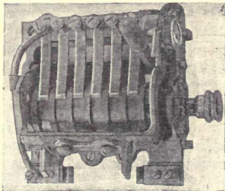
FIG. 27.—FRONT INTERIOR VIEW OF CAR-HEATING REGULATING SWITCH.
