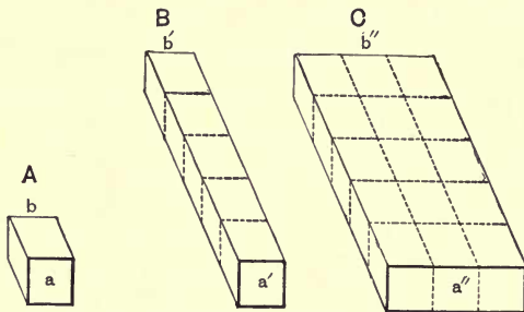
FIG. 3.—DIAGRAM REPRESENTING RELATION BETWEEN RESISTIVITY AND RESISTANCE.
