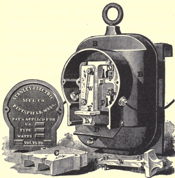
FIG. 20.—TRANSFORMER SAFETY FUSE-BOX
