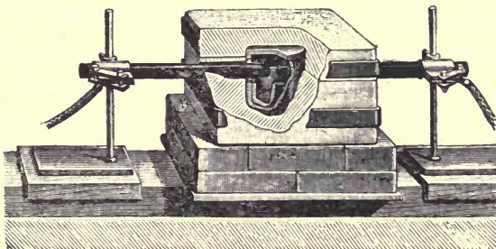
FIG. 77. —ELECTRIC FURNACE.
