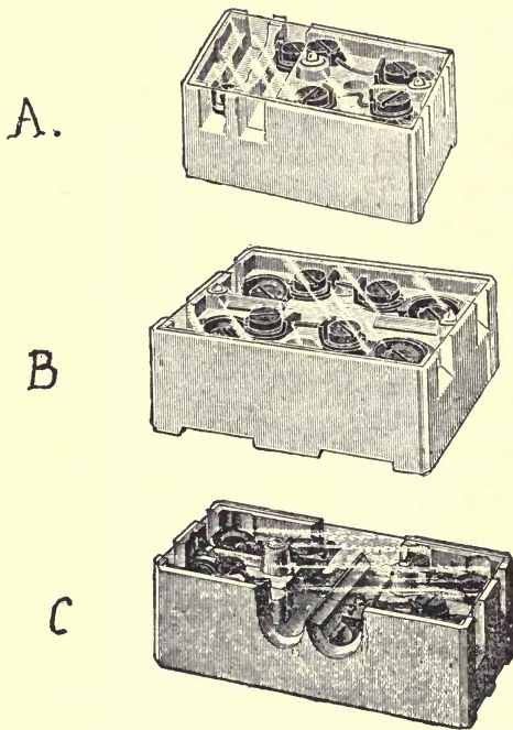
FIG. 12.—MICA-COVERED FUSE-BOXES.
