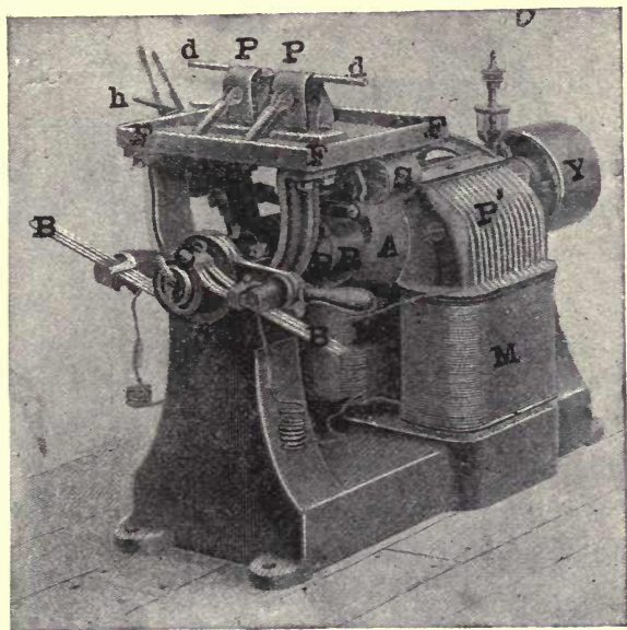
FIG. 58. —DIRECT WELDER FOR WELDING BABY CARRIAGE TIRES AT THE RATE OF 1500 TO 2000 IN TEN HOURS.
