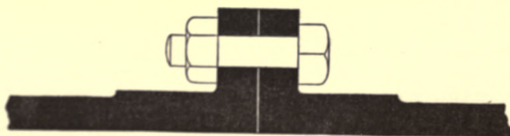
Fig. 120.—Flanged Joint in Cast-iron Pipes.
