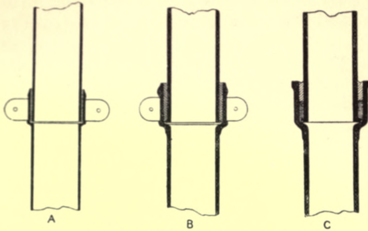
Fig. 222.—Joints of Iron Soil-pipes. A, light; B, medium; C, strong.
