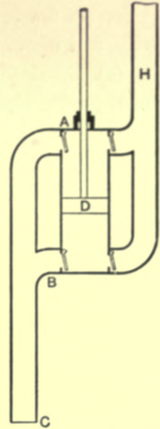
Fig. 119.—Section of Improved Double-acting Force-pump.
