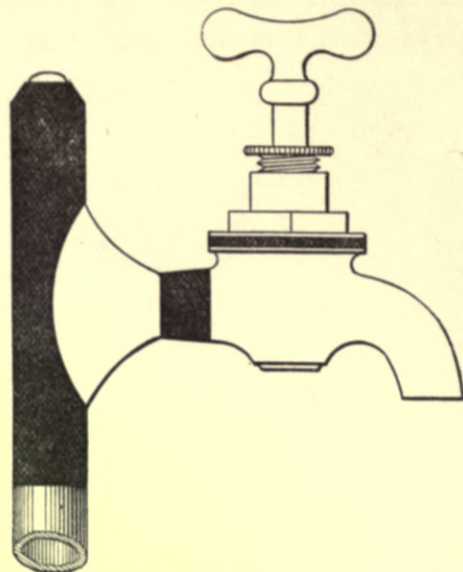
Fig. 142.—Bib-tap "Wiped" to a Lead Pipe
