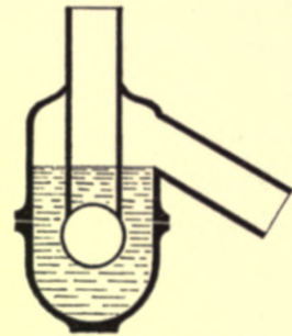
Fig. 199. — Section of the Bower Trap.
