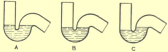
Fig. 200.—Sections of Traps to Illustrate Syphonage.
