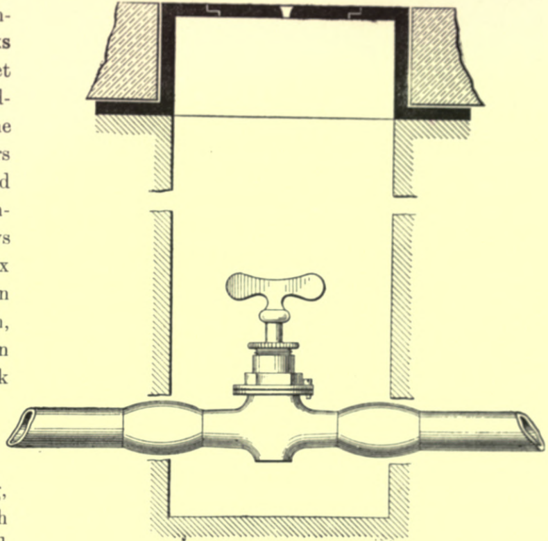
Fig. 134.—Stop-cock and Box.
