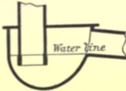
Fig. 189.—Section of Old D-trap.
