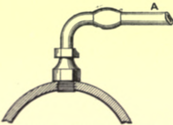
Fig. 132.—Connection of Lead Service-pipe with Iron Main.
