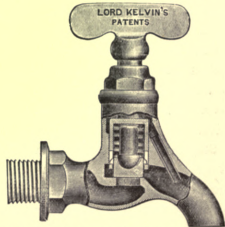
Fig. 156.—Section through Lord Kelvin's Patent Bib-tap.
