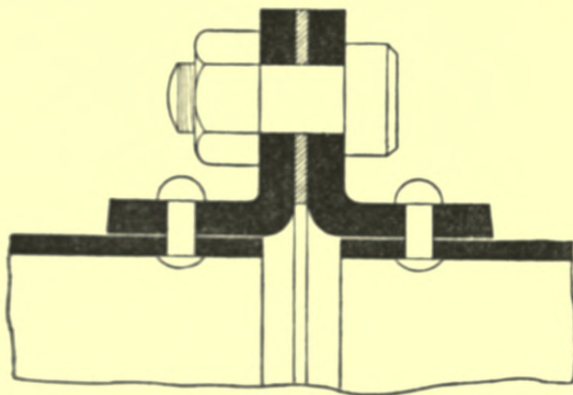
Fig. 123.—Flanged Joint for Wrought-iron and Steel Pipes
