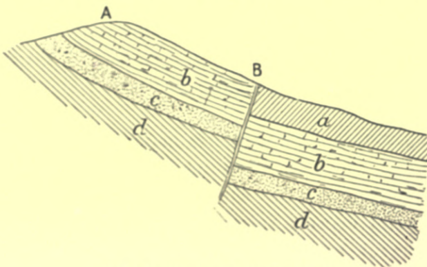
Fig. 99.—Section of Strata showing a Fault.
