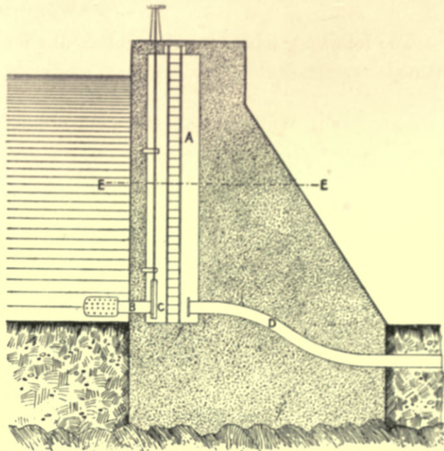
Fig. 107.—Vertical Section of Valve-chamber.
