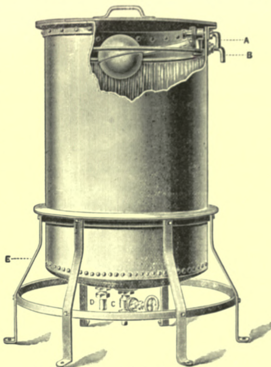
Fig. 149.—Durrans's "Kallo" Self-cleansing Cistern.
