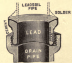
Fig. 249. — Robinson's "Enable" Connection between Lead Soil-pipe and Earthenware Drain.
