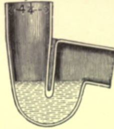
Fig. 193.—Section of Large-size Anti-D Trap.
