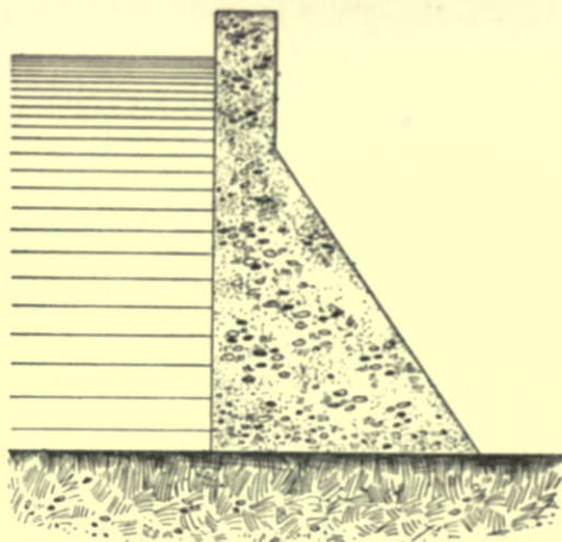
Fig. 105.—Transverse Section of Concrete Dam.
