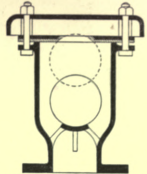
Fig. 124.—Air-valve for Water-pipes.
