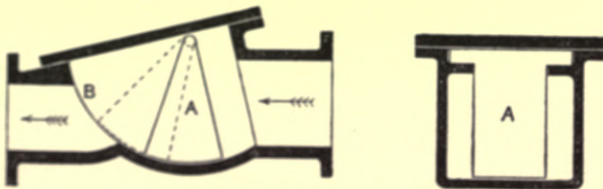
Fig. 126.—Longitudinal and Transverse Sections through Simple Reducing-valve.
