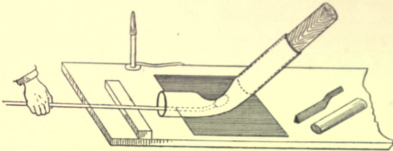
Fig. 225.—Bending Drawn-lead Pipe: 1st stage.
