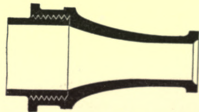
Fig. 129.—Section through Hose-nozzle.
