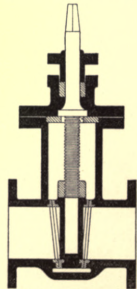
Fig. 127.—Section through Sluice-valve.
