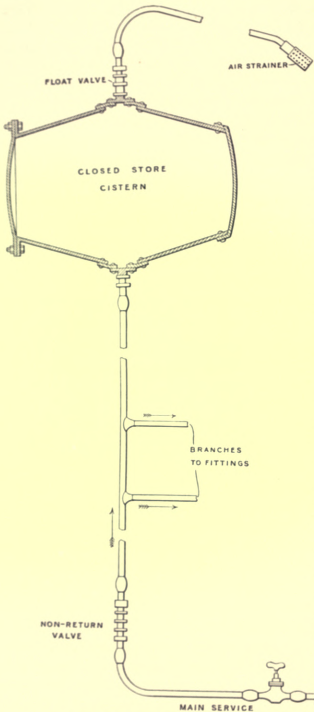
Fig. 148.—Harding's Closed Water-cistern.
