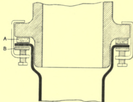
Fig. 243.—Socketed and Flanged Joint with India-rubber Ring, &c.
