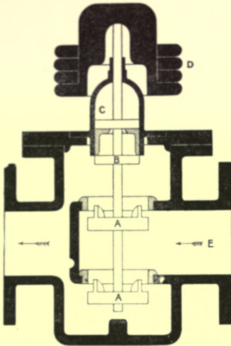
Fig. 125.—Section through Equilibrium Reducing-valve.
