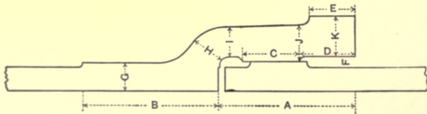
Fig. 122.—Turned-and-bored Joint in Cast-iron Pipes.
