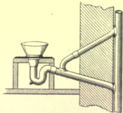
Fig. 214.—Waste-pipe from Slop-hopper.
