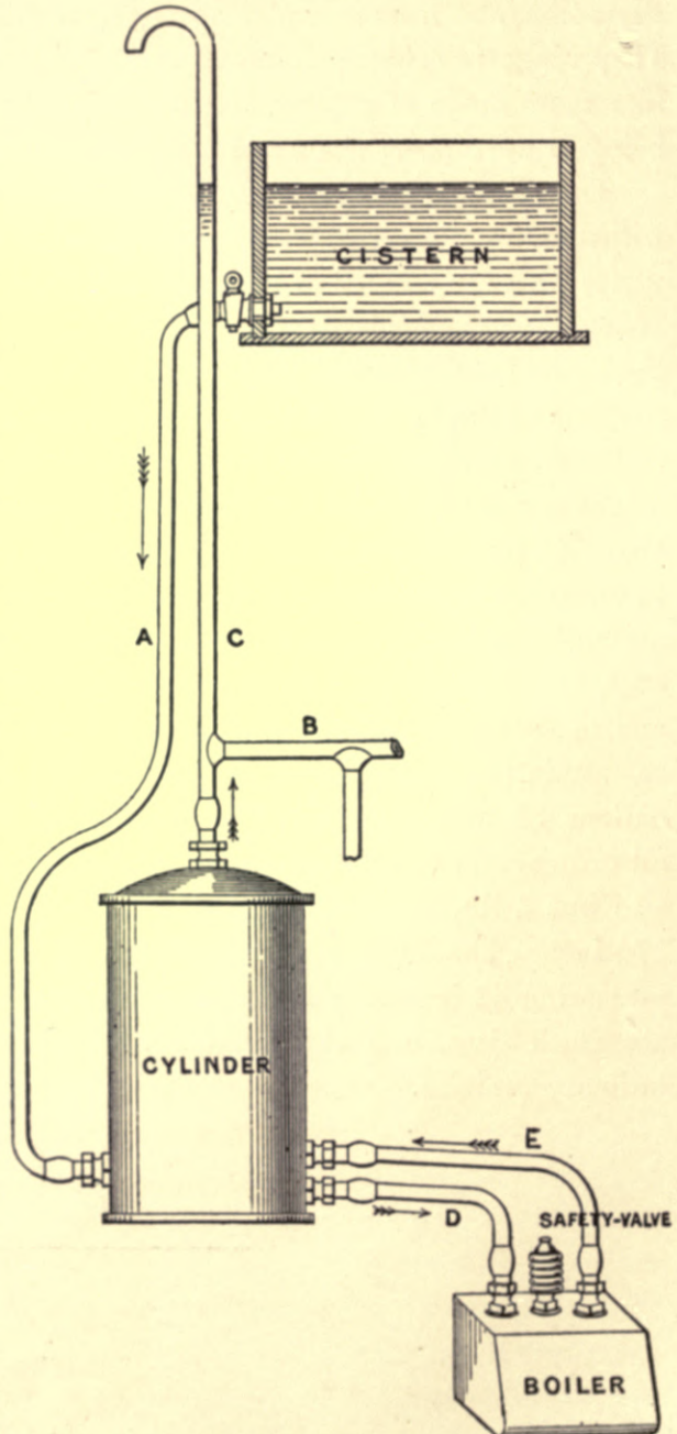
Fig. 167.—Ordinary Hot-water Apparatus: Cylinder-system.
