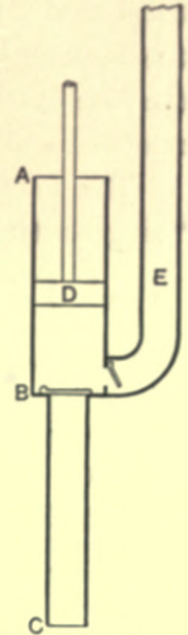
Fig. 115.—Section of Force-pump.
