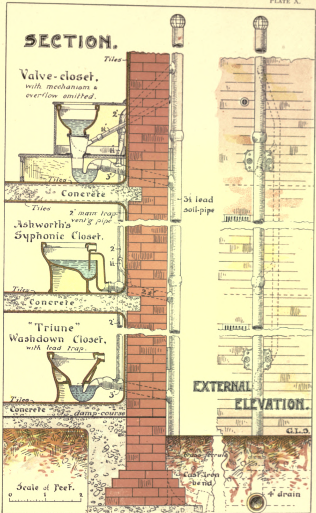
SOIL-PIPE AND TRAP-VENTILATING PIPES FOR A TIER OF THREE CLOSETS.
