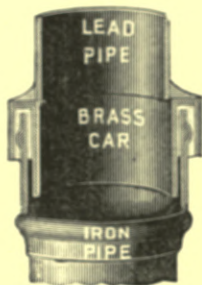
Fig. 247. — Robinson's "Enable" Connecting Collar for joining Iron and Lead Pipes.
