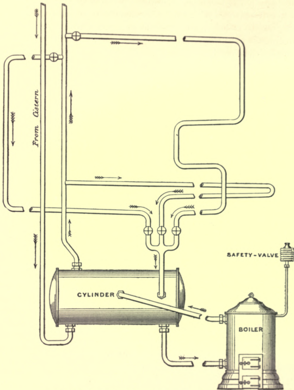
Fig. 168.—Hot-water Apparatus, with Independent Boiler and Horizontal Cylinder.
