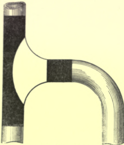
Fig. 141.—Side-branch Wiped Joint.
