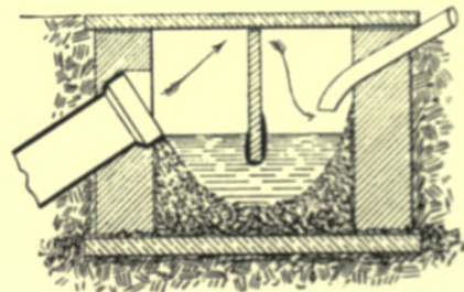
Fig. 188.—Section of Mid-feather Trap.
