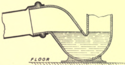
Fig. 242.—Improved Socketed Joint between Earthenware Trap and Lead Soil-pipe.
