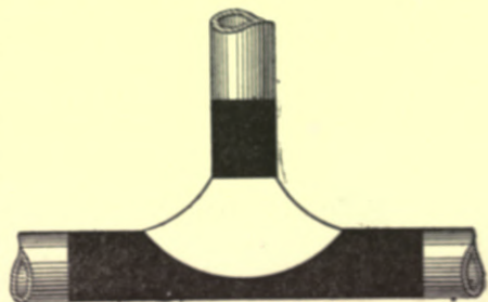
Fig. 140.—Equal-branch Wiped Joint.
