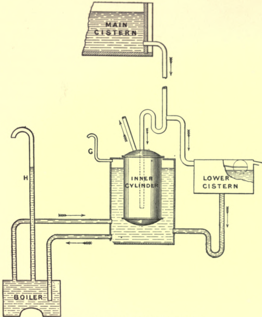
Fig. 171.—Double-cylinder Hot-water Apparatus: System 2.
