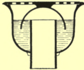
Fig. 198. — Section of Bell-trap for Sink.
