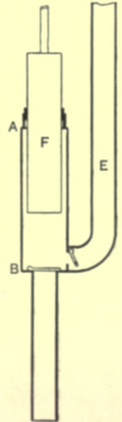
Fig. 116.—Section of Force-pump, with Plunger.
