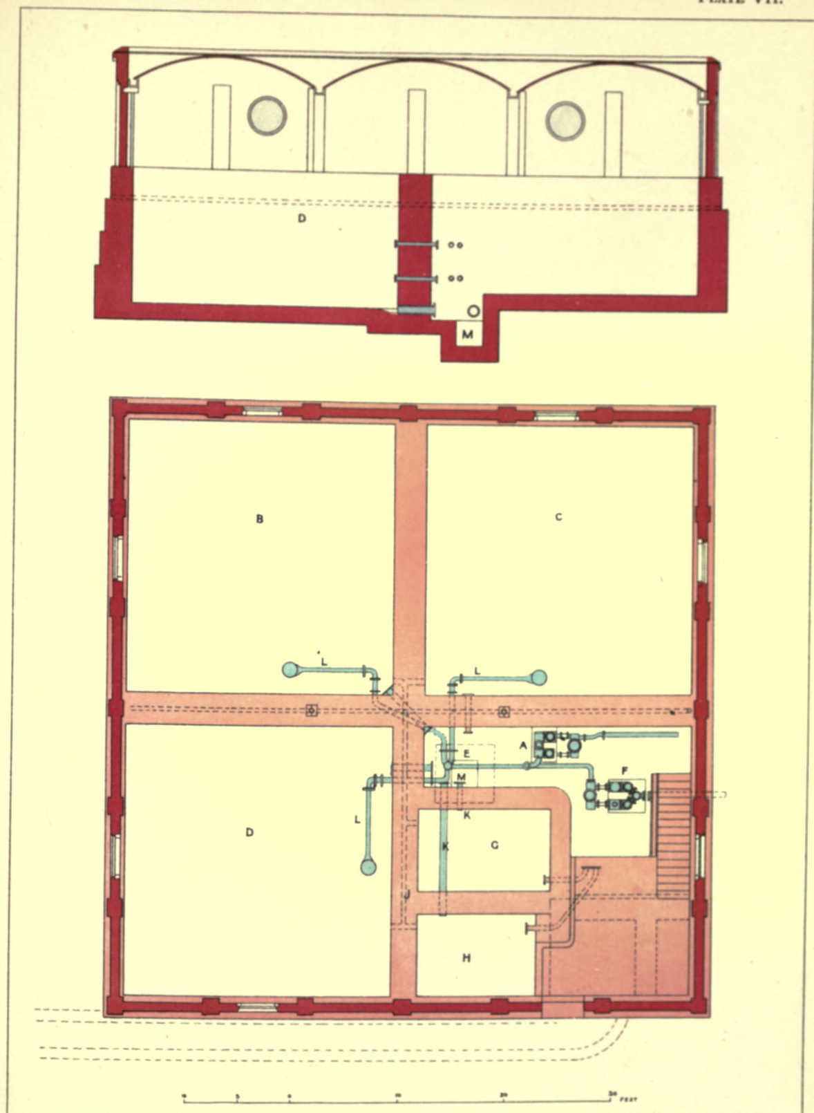
PLAN AND SECTION OF THE WATER-SOFTENING INSTALLATION AT LUTON HOO.
