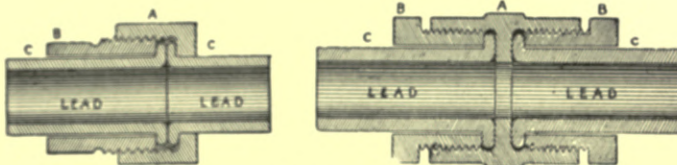
Fig. 146.—Two Methods of Joining Lead-encased Tin Pipes.
