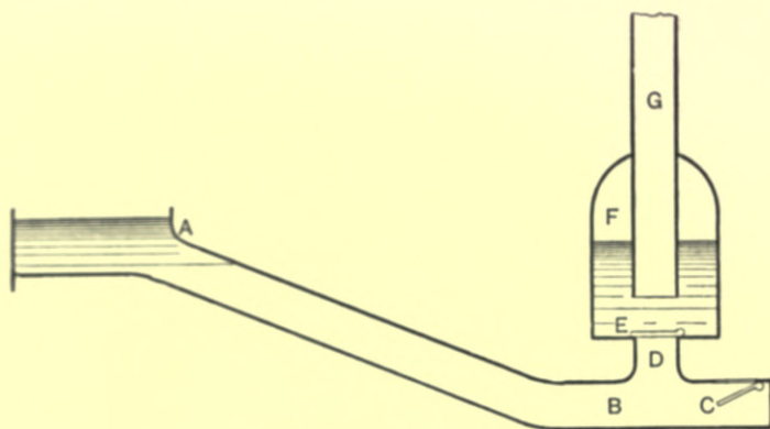
Fig. 112.—Section of Hydraulic Ram.
