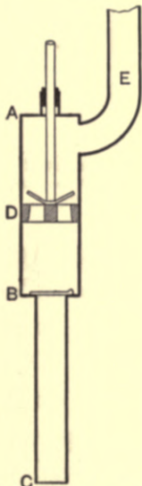
Fig. 114.—Section of Lifting-pump, with high Delivery-pipe.
