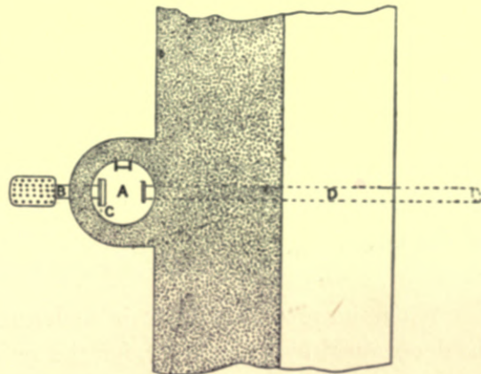
Fig. 108.—Horizontal Section of Valve-chamber on line E-E.
