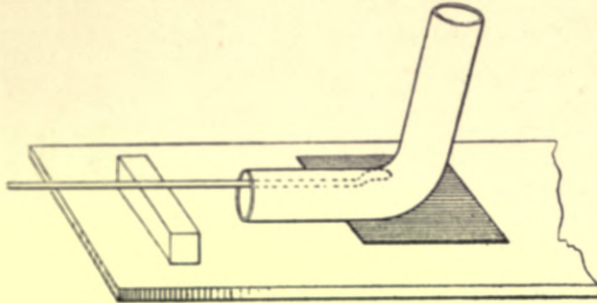
Fig. 227. - Bending Drawn-lead Pipe: 3rd stage.
