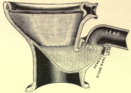
Fig. 246.—Robinson's "Adaptable" Joint.
