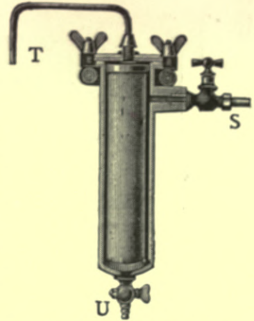
Fig. 183.—Berkefeld Single-tube Filter. s, water-supply; T, filtered-water outlet; U, flushing tap.
