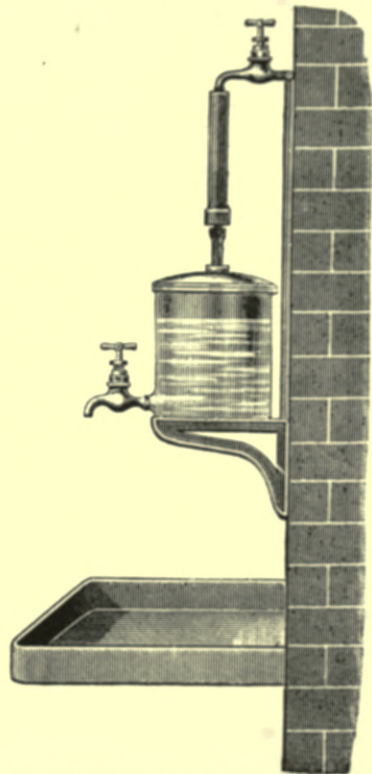
Fig. 186.—Pasteur (Chamberland) Filter, with Stoneware Reservoir.
