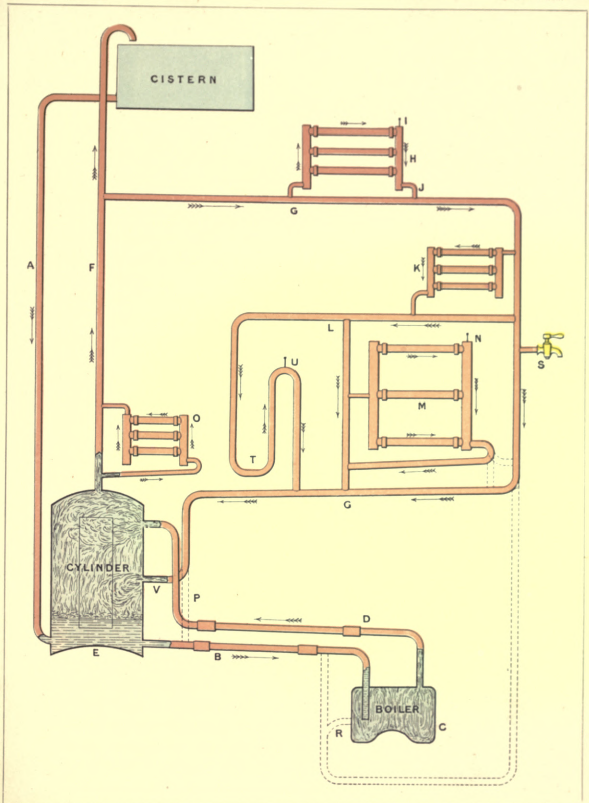
DIAGRAM OF HOT-WATER CIRCULATION—CYLINDER SYSTEM.
