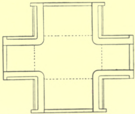
Fig. 211.—Lead for Small Sink, ready for folding and putting in position.
