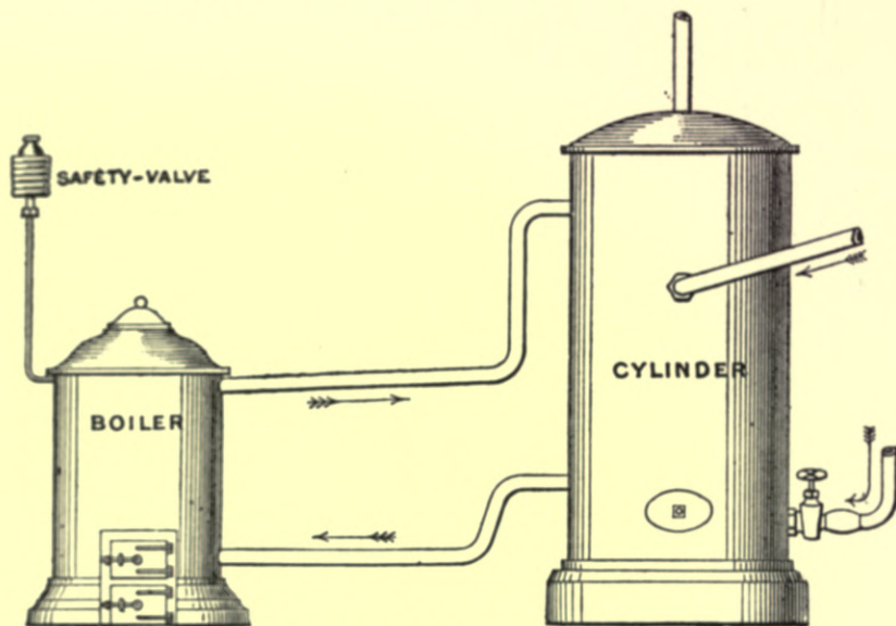
Fig. 169. — Hot-water Apparatus, with Independent Boiler and Vertical Cylinder.
