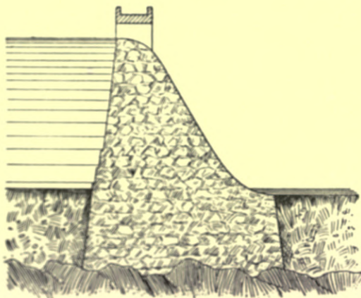
Fig. 106.—Section of Rubble Dam, Vyrnwy Reservoir.
