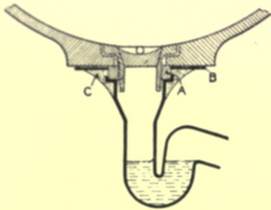
Fig. 206.—Connection of Lavatory Basin and Trap.
