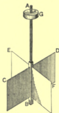
Fig. 104.—Float for Measuring the Velocity of a Stream below the Surface.
