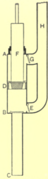
Fig. 117.—Section of Plunger-and-bucket Pump.
