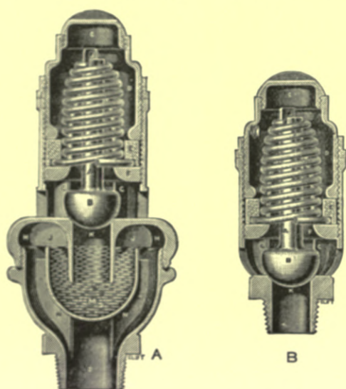
Fig. 181.—Keith's Tension-spring Safety-valves. A, With liquid seal. B, Without liquid seal.
