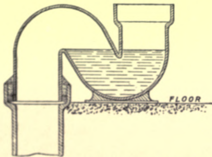
Fig. 239.—Connection of Earthenware Trap to Earthenware Drain.
