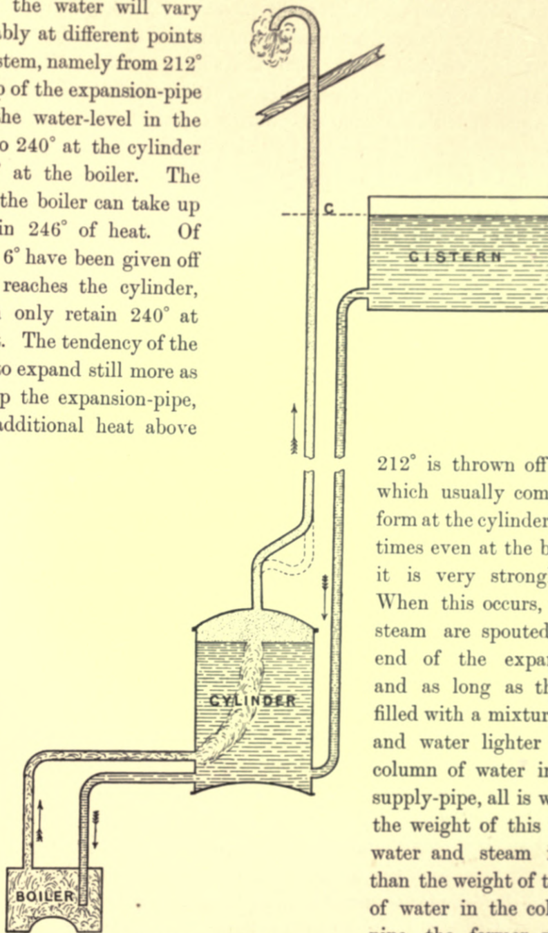
Fig. 176.—Hot-water Apparatus: Cylinder-system.
