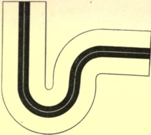
Fig. 251. —Hand-made Round-pipe P-trap.
