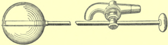
Fig. 151.—Side-screw Ball-cock, with Stuffing-box and loose Valve.
