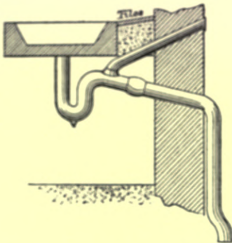
Fig. 201.—Waste-pipe and Air-pipe to Sink.
