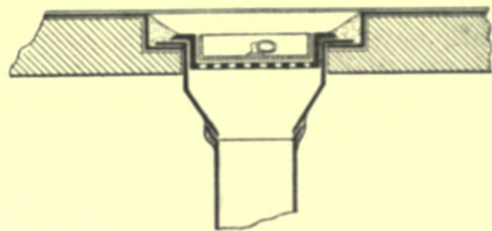
Fig. 205.—Connection of Lead-lined Sink and Trap (sunk-plug outlet).
