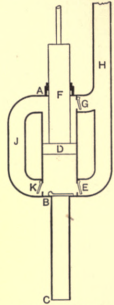
Fig. 118.—Section of Double-acting Force-pump, with Solid Piston.
