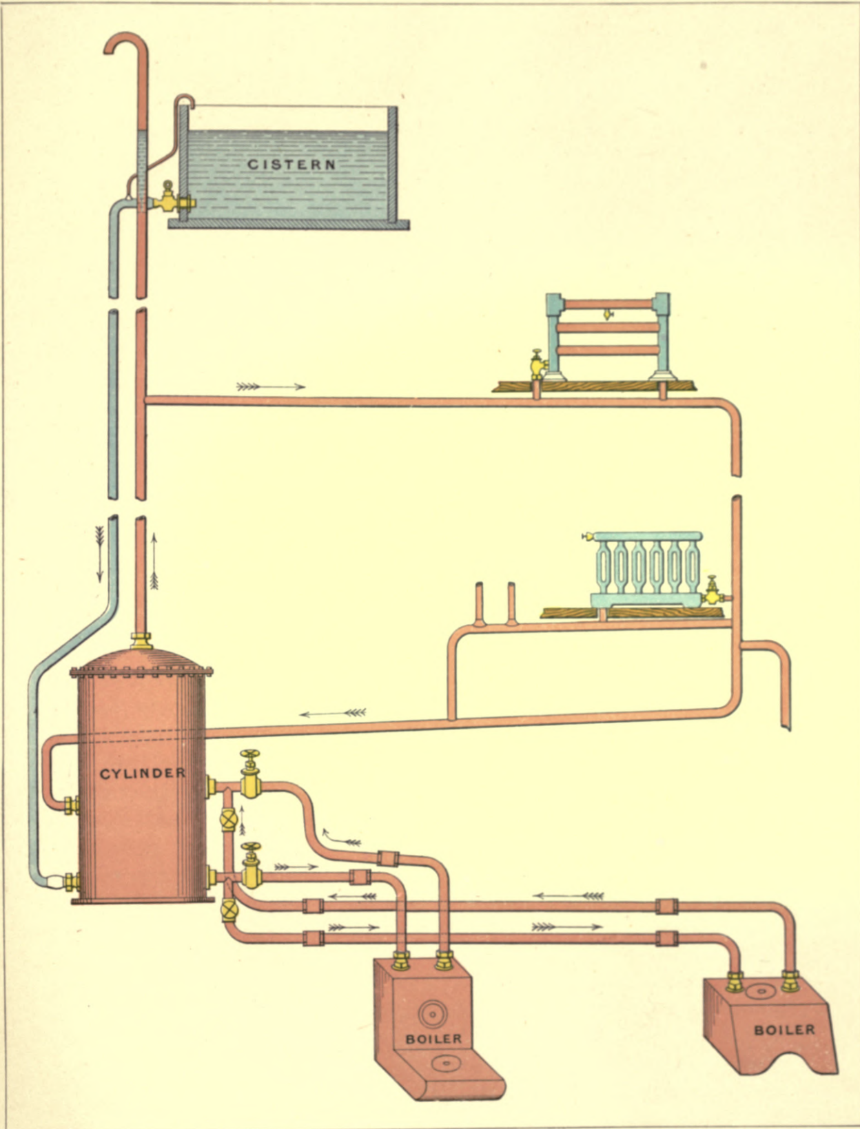
HOT-WATER APPARATUS WITH TWO BOILERS—CYLINDER SYSTEM.
