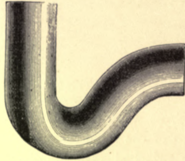
Fig. 252. —Cast-lead P-trap, with too easy Outgo.
