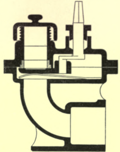
Fig. 128.—Section through Hydrant-valve.
