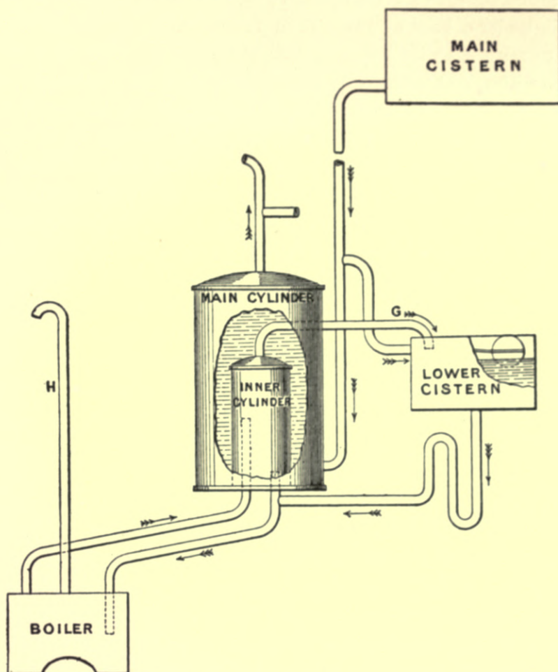
Fig. 170.—Double-cylinder Hot-water Apparatus: System 1.
