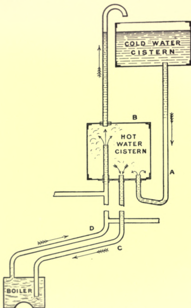
Fig. 172.—Hot-water Apparatus: Tank-system.
