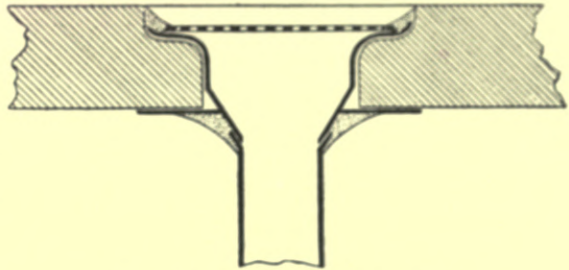
Fig. 203.—Connection of Stone Sink and Trap.
