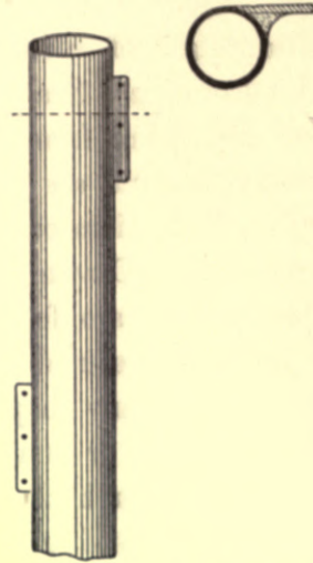
Fig. 209.—Waste-pipe secured by Single Lead Tacks.
