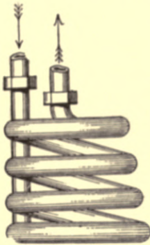
Fig. 166.—Coiled-pipe Boiler.
