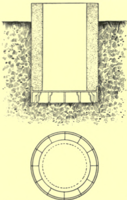
Fig. 110.—Plan and Section of Well constructed of Concrete.
