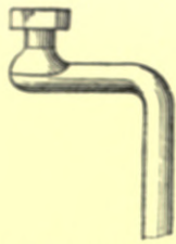
Fig. 215.—Bad Form of Joint between Syphon-cistern and Flush-pipe.
