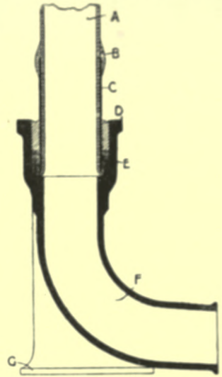
Fig. 221.—Cast-iron Bend with Foot-rest, and Connection with Lead Soil-pipe.
