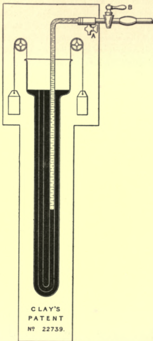
Fig. 182.—Mercury Regulator for Hot-water Apparatus.
