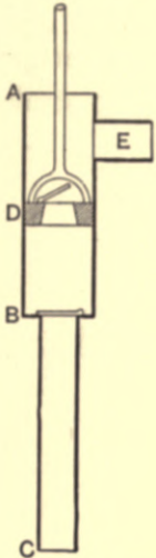
Fig. 113.—Section of Lifting-pump.
