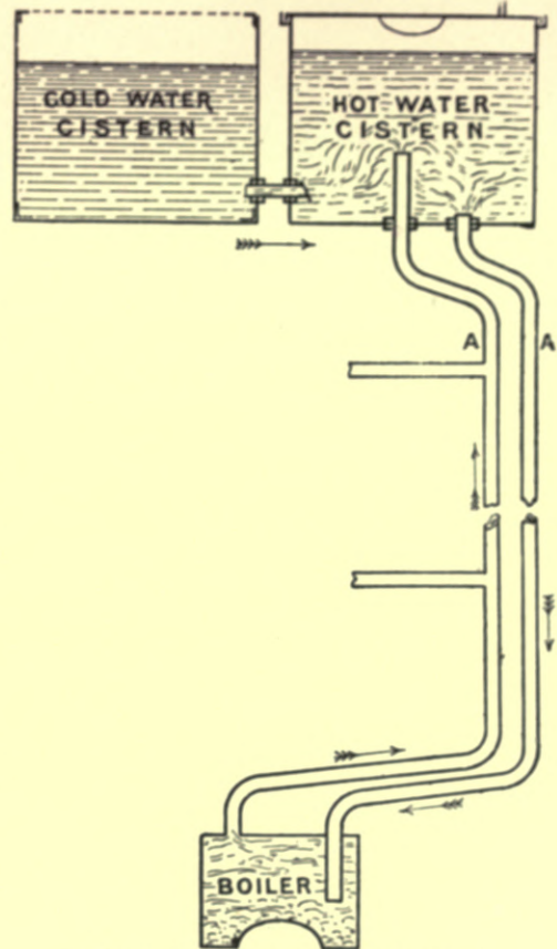
Fig. 173.—Hot-water Apparatus: Hot-cistern Circulation-system.
