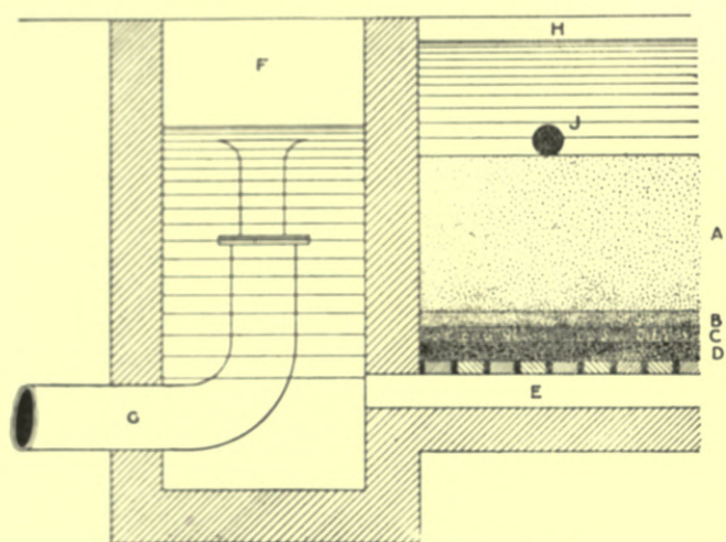
Fig. 131. —Section of Sand Filter and Outlet-chamber.
