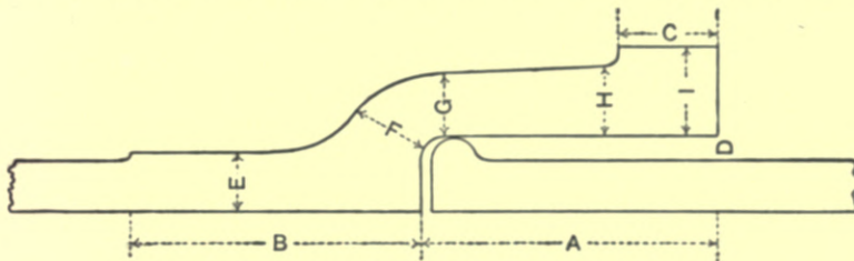
Fig. 121.—Spigot-and-socket Joint in Cast-iron Pipes.
