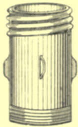
Fig. 244.—Freeman's "Grip" Joint.
