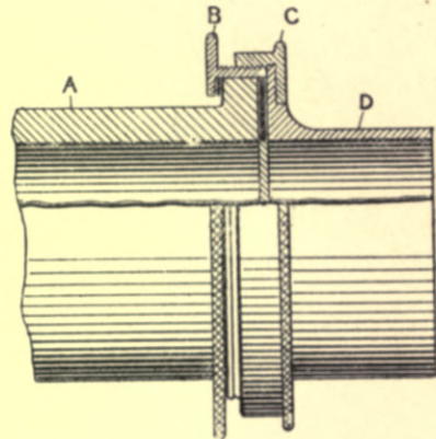
Fig. 245.—Quirk, Sharp, & Co.'s Joint.
