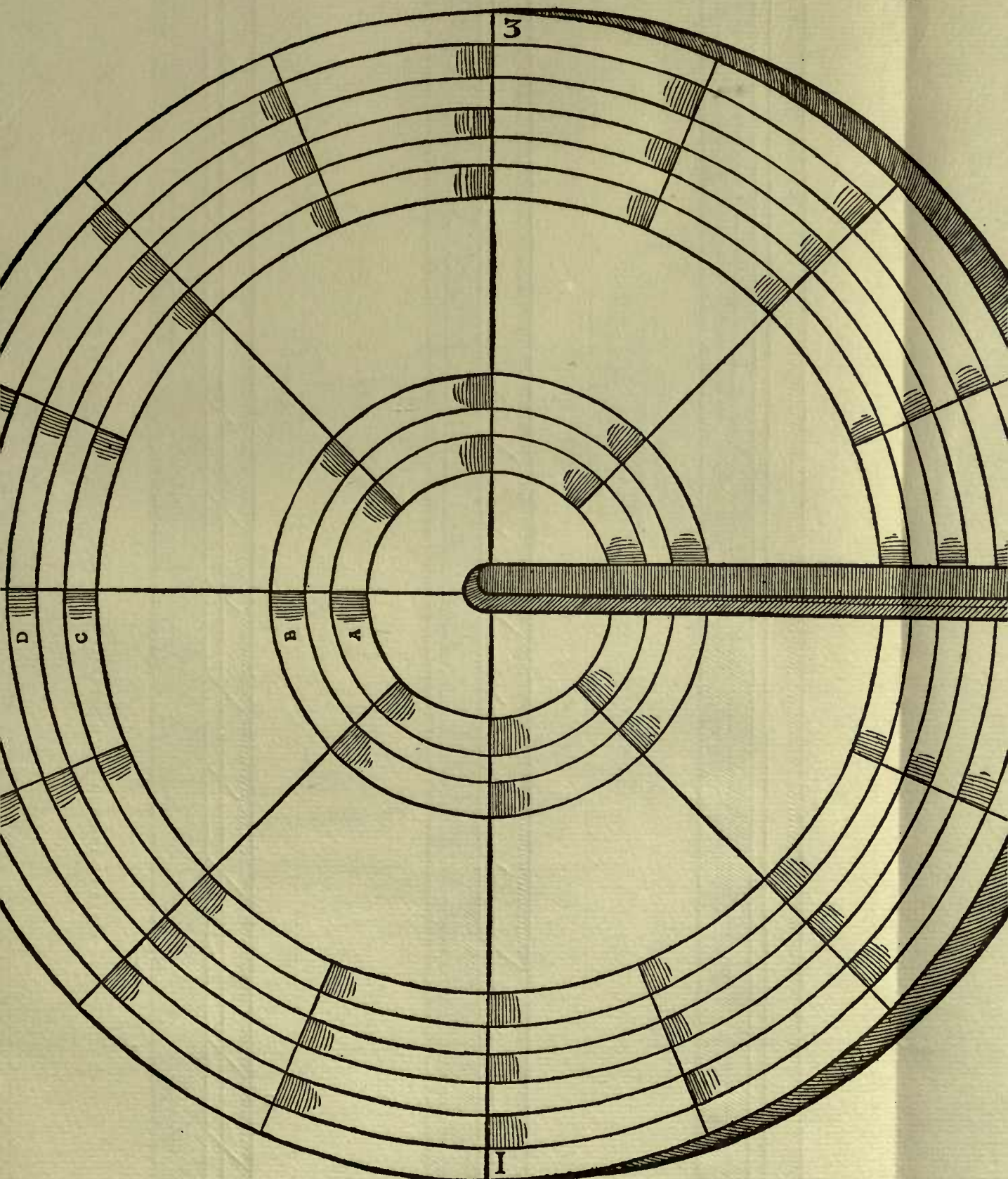
A, B, C, D, E—FIVE WAXED CIRCLES OF THE orbis. F—OPENING OF SAME. G—SCREW. H—PERFORATED IRON.
