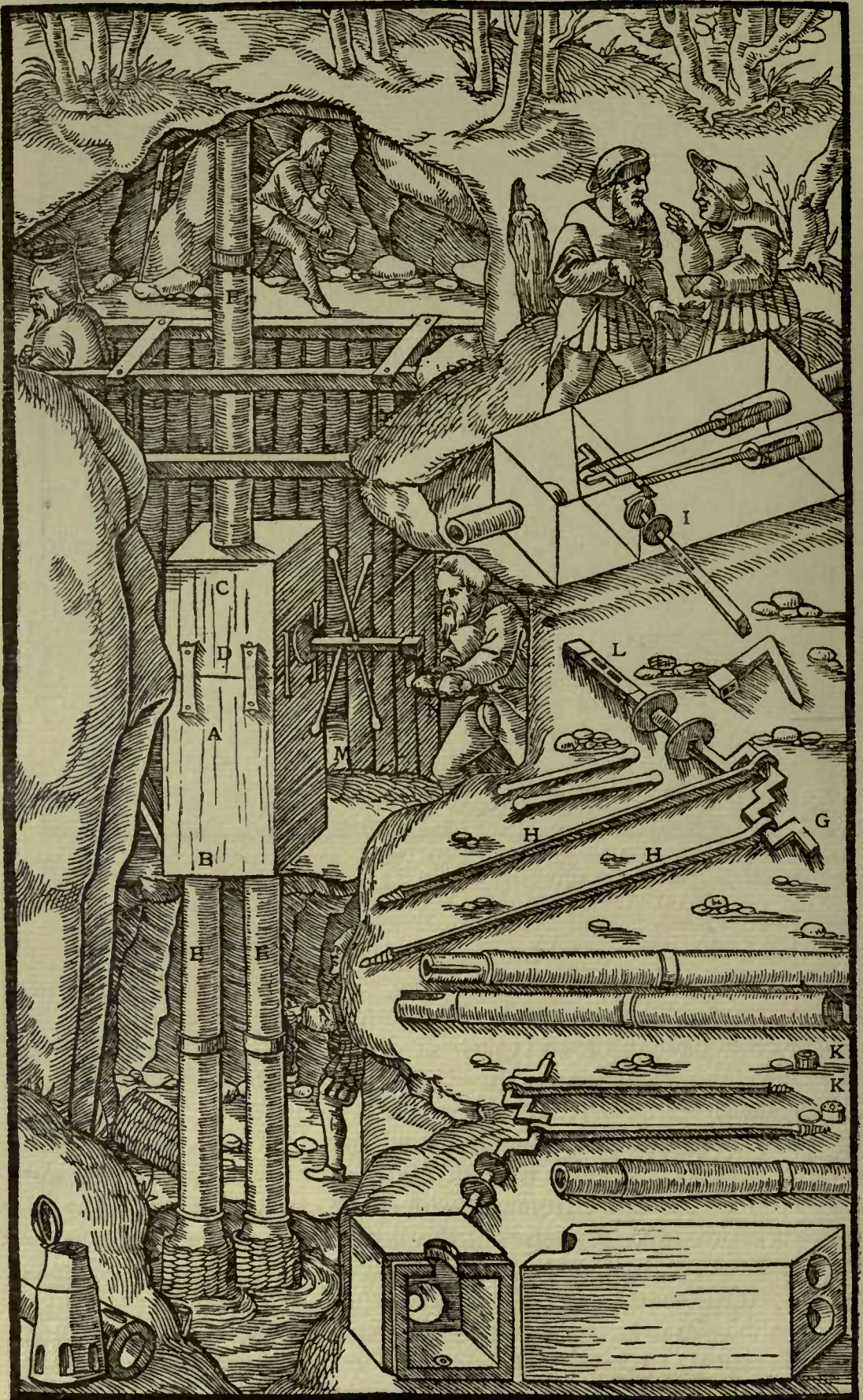
A—Box. B—LOWER PART OF BOX. C—UPPER PART OF SAME. D—CLAMPS. E—PIPES BELOW THE BOX. F—COLUMN PIPE FIXED ABOVE THE BOX. G—IRON AXLE. H—PISTON-RODS. I—WASHERS TO PROTECT THE BEARINGS. K—LEATHERS. L—EYES IN THE AXLE. M—RODS WHOSE ENDS ARE WEIGHTED WITH LUMPS OF LEAD. N—CRANK.
