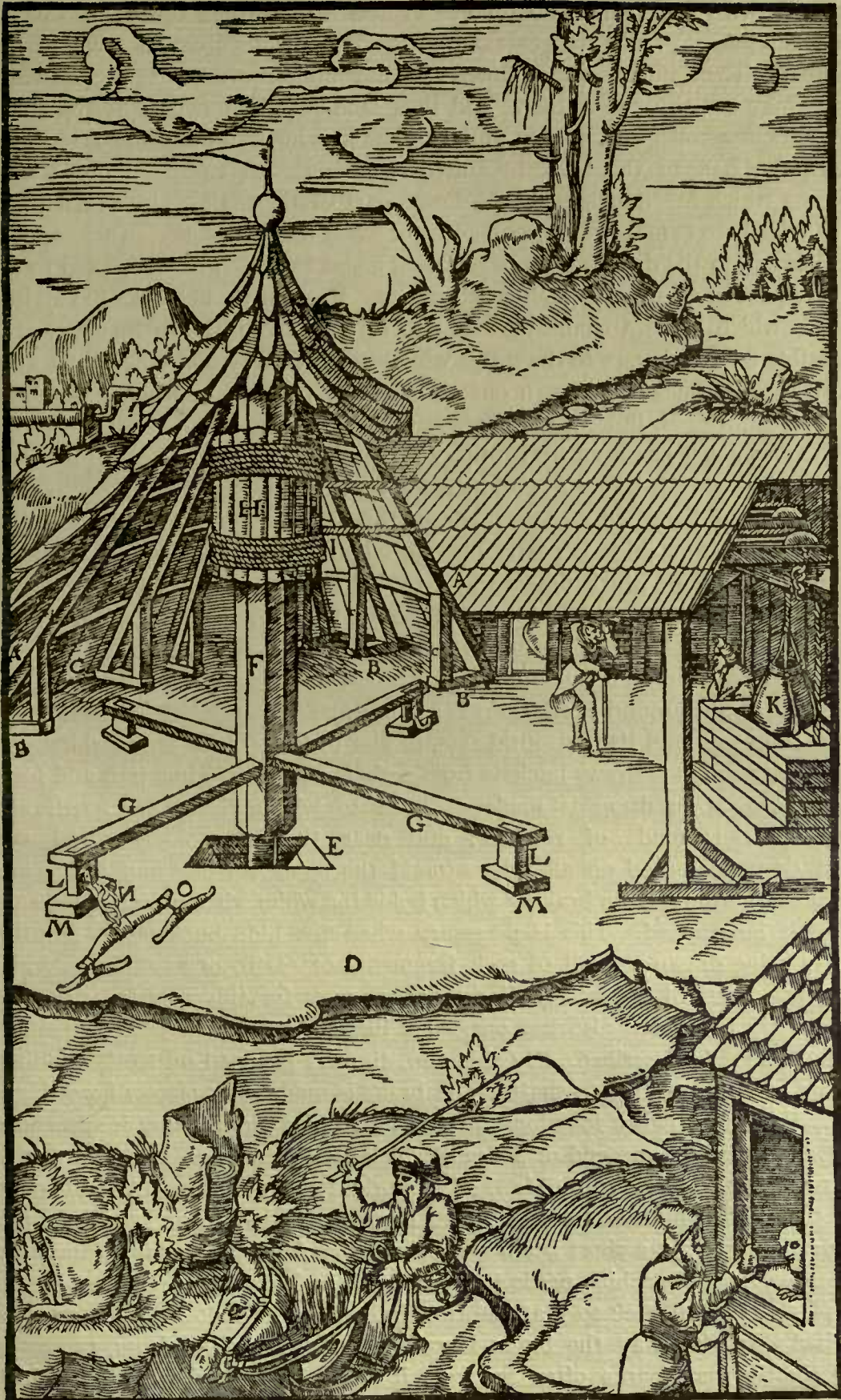
A—UPRIGHT BEAMS. B—SILLS LAID FLAT UPON THE GROUND. C—POSTS. D—AREA. E—SILL SET AT THE BOTTOM OF THE HOLE. F—AXLE. G—DOUBLE CROSS-BEAMS. H—DRUM. I—WINDING-ROPES. K—BUCKET. L—SMALL PIECES OF WOOD HANGING FROM DOUBLE CROSS-BEAMS. M—SHORT WOODEN BLOCK. N—CHAIN. O—POLE BAR. P—GRAPPLING HOOK. (Some members mentioned in the text are not shown).
