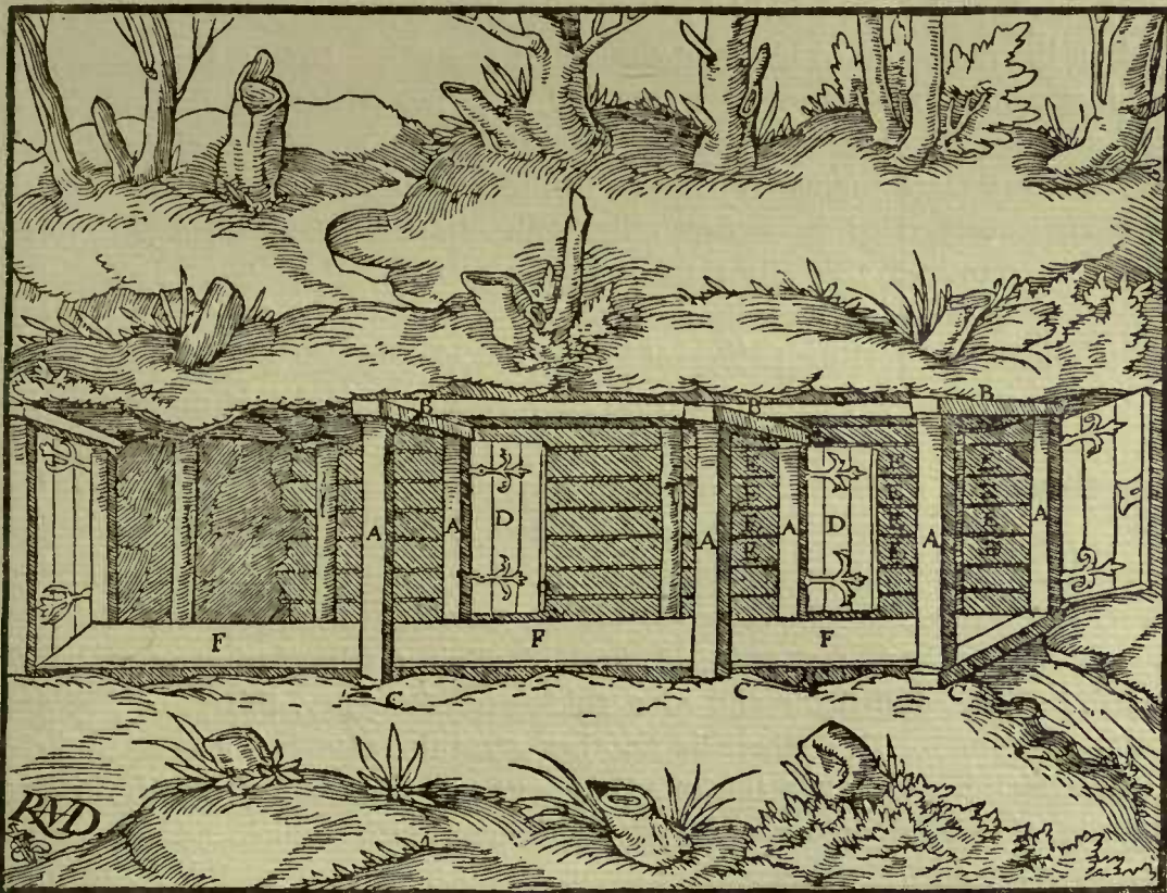
A—POSTS. B—CAPS. C—SILLS. D—DOORS. E—LAGGING. F—DRAINS.
