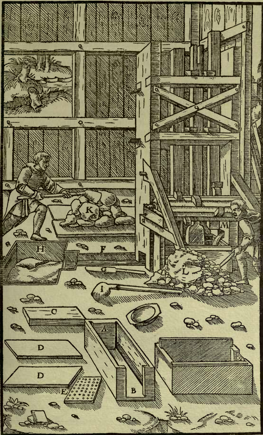
A—MORTAR. B—OPEN END OF MORTAR. C—SLAB OF ROCK. D—IRON SOLE PLATES. E—SCREEN. F—LAUNDER. G—WOODEN SHOVEL. H—SETTLING PIT. I—IRON SHOVEL. K—HEAP OF MATERIAL WHICH HAS SETTLED. L—ORE WHICH REQUIRES CRUSHING. M—SMALL LAUNDER.
