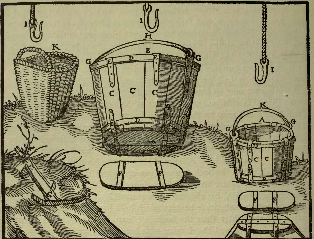
A—SMALL BUCKET. B—LARGE BUCKET. C—STAVES. D—IRON HOOPS. E—IRON STRAPS. F—IRON STRAPS ON THE BOTTOM. G—HAFTS. H—IRON BALE. I—HOOK OF DRAWING-ROPE. K—BASKET. L—HIDE BUCKET OR SACK.
