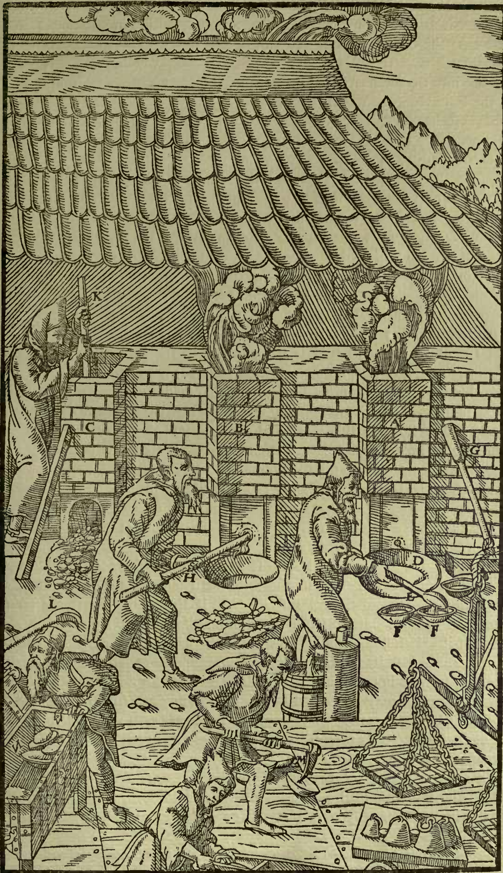
A, B, C—THREE FURNACES. AT THE FIRST STANDS THE SMELTER, WHO WITH A LADLE POURS THE ALLOY OUT OF THE FOREHEARTH INTO THE MOULDS. D—FOREHEARTH. E—LADLE. F—MOULDS. G—ROUND WOODEN RAMMER. H—TAPPING-BAR. AT THE SECOND FURNACE STANDS THE SMELTER, WHO OPENS THE TAP-HOLE WITH HIS TAPPING-BAR. THE ASSISTANT, STANDING ON STEPS PLACED AGAINST THE THIRD FURNACE WHICH HAS BEEN BROKEN OPEN, CHIPS OFF THE ACCRETIONS. I—STEPS. K—SPATULA. L—THE OTHER HOOKED BAR. M—MINE CAPTAIN CARRYING A CAKE, IN WHICH HE HAS STUCK THE PICK, TO THE SCALES TO BE WEIGHED. N—ANOTHER MINE CAPTAIN OPENS A CHEST IN WHICH HIS THINGS ARE KEPT.
