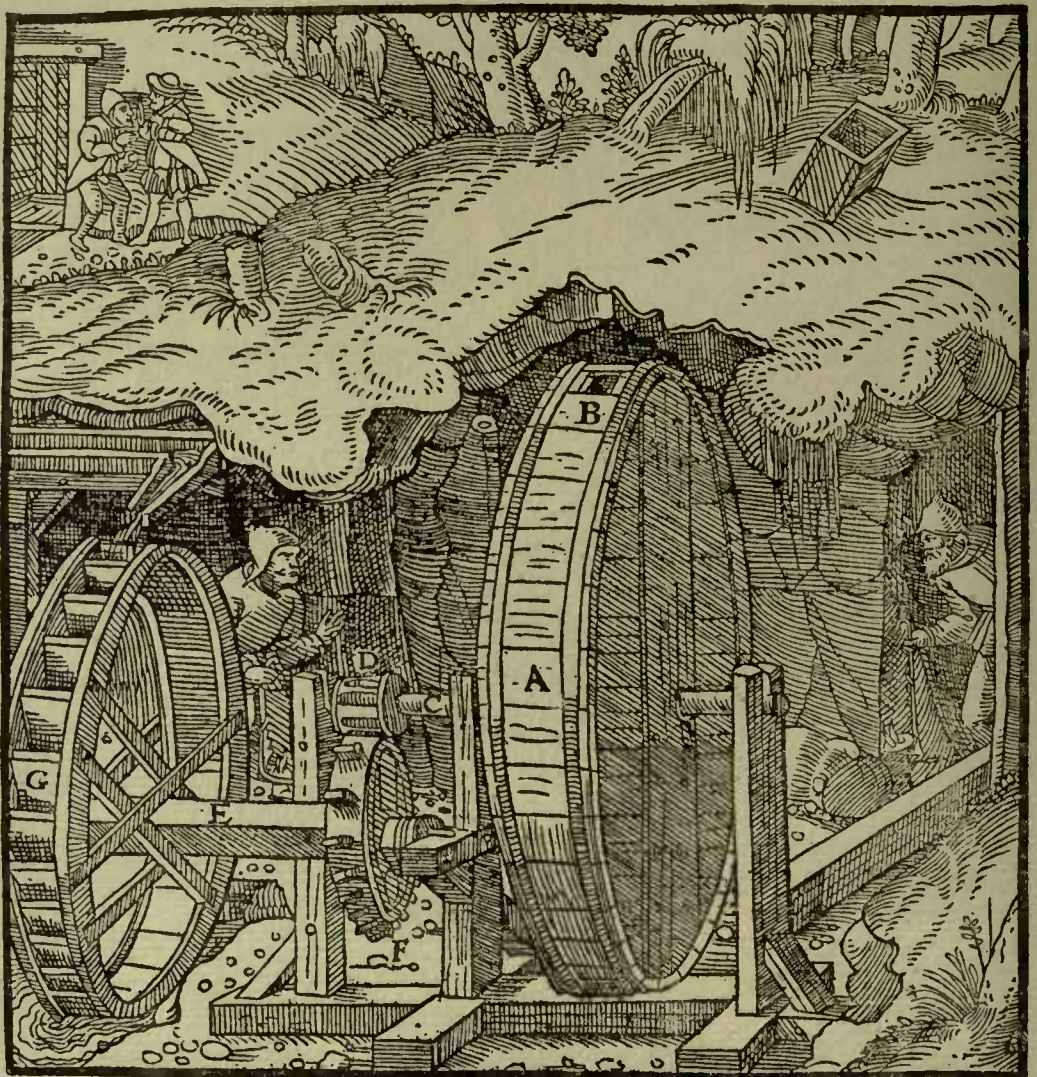
A—HOLLOW DRUM. B—ITS BLOW-HOLE. C—AXLE WITH FANS. D—DRUM WHICH IS MADE OF RUNDLES. E—LOWER AXLE. F—ITS TOOTHED WHEEL. G—WATER WHEEL.
