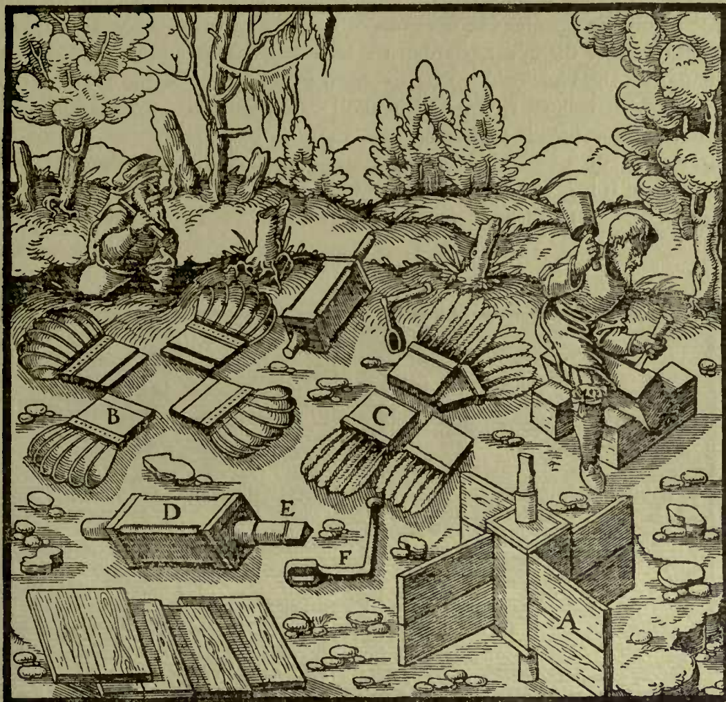
A—FIRST KIND OF FAN. B—SECOND KIND OF FAN. C—THIRD KIND OF FAN. D—QUADRANGULAR PART OF AXLE. E—ROUND PART OF SAME. F—CRANK.
