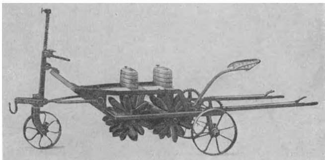
c) Spitzenbergs Wühllegge.
