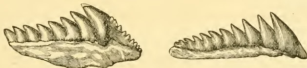
FIG. 16.—Teeth of Notidanus gigas , Red Crag, Suffolk.
