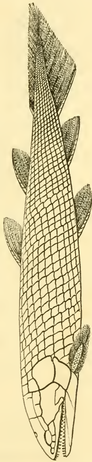
FIG. 51.— Osteolepis (restored outline after Fander), Old Red Sandstone, Scotland.
