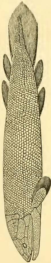
FIG. 50.— Glyptoptichius , Old Red Sandstone, Scotland.
