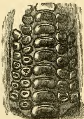
FIG. 66.—Upper dentition of Calodus ellipticus , Gault, Folkestone.
