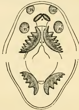
FIG. 44.—Mouth of Ceratodus . nn , narial openings; x , vomerine teeth; xx , palatopterygoid teeth; xxx , mandibular teeth.
