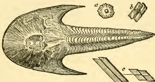
FIG. 41.— Cephalaspis Lyelli (dorsal aspect), from the Old Red Sandstone, Glammis, Forfarshire (about one-third the size of the original specimen). a , one of the peculiar tesserae into which the middle layer of the shield is divided by the blood-vessels (drawn natural size); b and c , scales from different parts of the body and tail.
