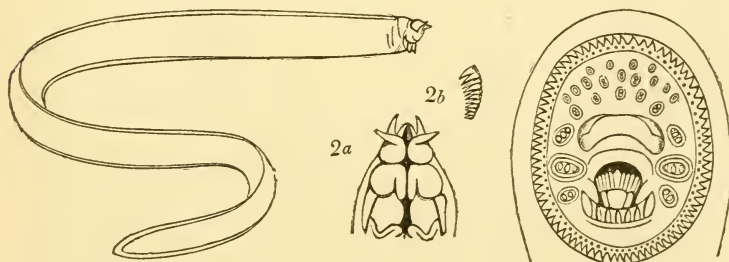
FIG. 2.—The “Hag-fish,” Myxine australis (recent). 2a , Lower aspect of head. 2b , A single detached tooth of Myxine .
