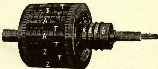
FIG. 68.—MONOCYCLIC ARMATURE.
