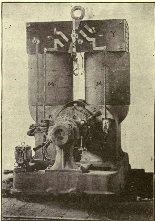
FIG. 15.—BIPOLAR CONTINUOUS-CURRENT GENERATOR.
