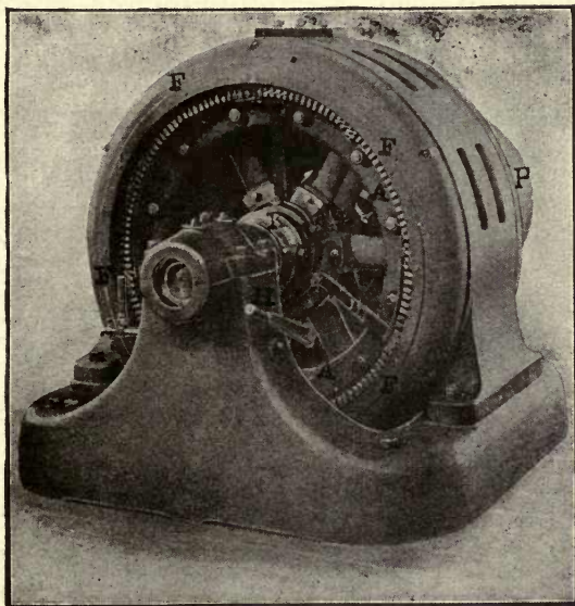
FIG. 72.—125-HORSE-POWER INDUCTION MOTOR.
