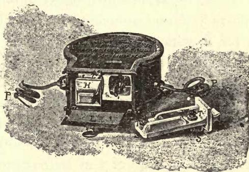
FIG. 36.—DETAILS OF TRANSFORMER FUSE-BOX.
