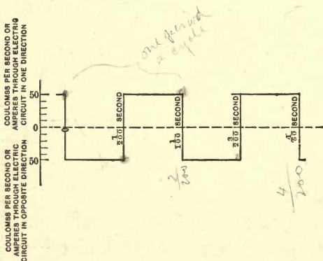
FIG. 5.—CURVE OF ALTERNATING-CURRENT FLOW.
