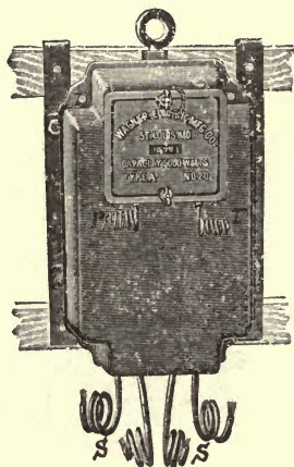
FIG. 34.—100-LIGHT STANDARD TRANSFORMER.
