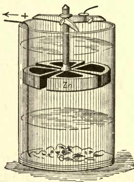
FIG. 7.—GRAVITY CELL.
