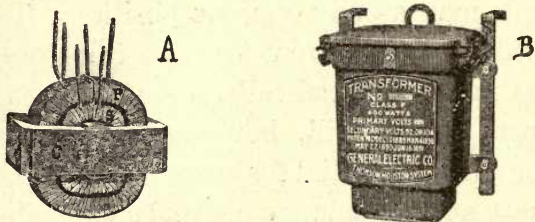
FIG. 31.—TRANSFORMER SHOWING INTERNAL CONSTRUCTION.
