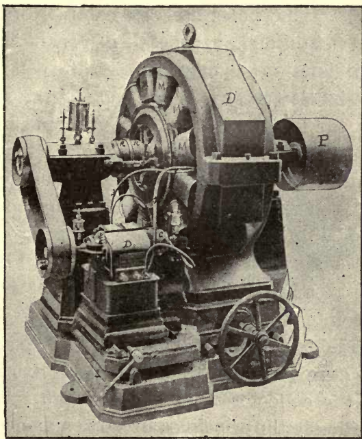
FIG. 17.—SEPARATELY-EXCITED ALTERNATOR.
