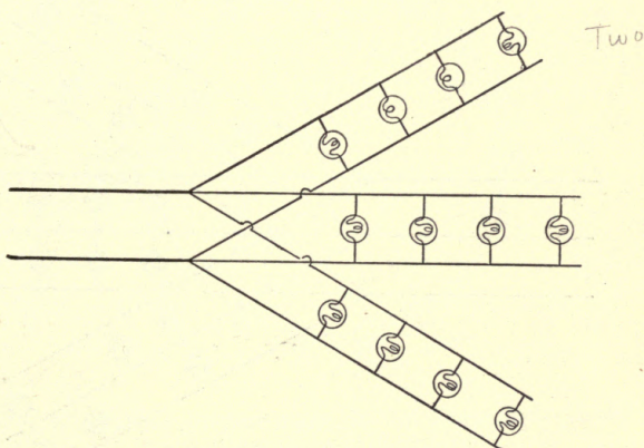
FIG. 45.—TWO-WIRE SYSTEM OF MULTIPLE CONNECTED LAMPS.
