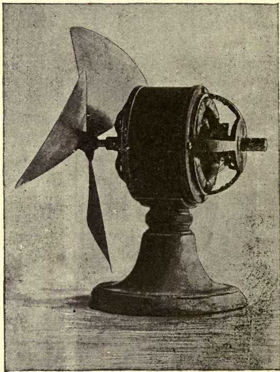
FIG. 56.—ONE-EIGHTH H.P. ALTERNATING-CURRENT FAN MOTOR.
