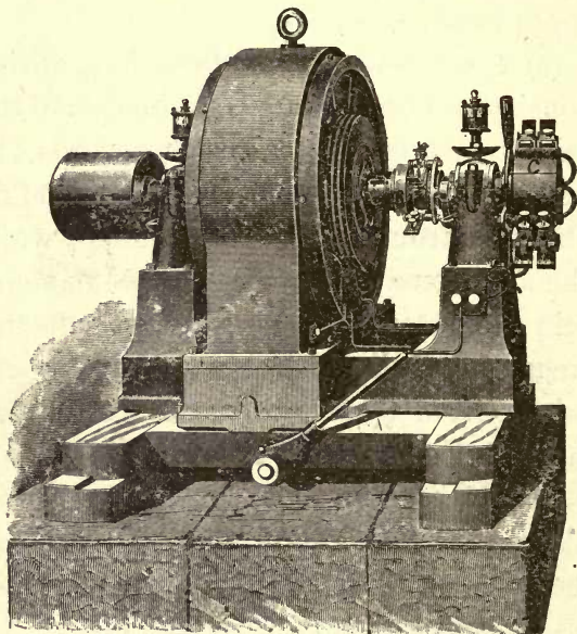
FIG. 21.—SELF-EXCITING ALTERNATOR.
