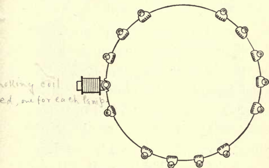
FIG. 47.—SERIES DISTRIBUTION OF INCANDESCENT LAMPS WITH ALTERNATING CURRENTS.
