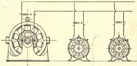
FIG 54.--ALTERNATOR WITH SYNCHRONOUS MOTORS.
