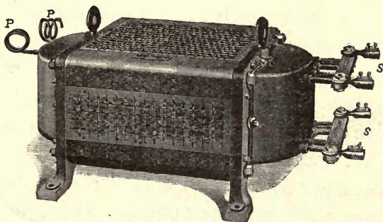
FIG. 39.—500-LIGHT TRANSFORMER, INDOOR TYPE.
