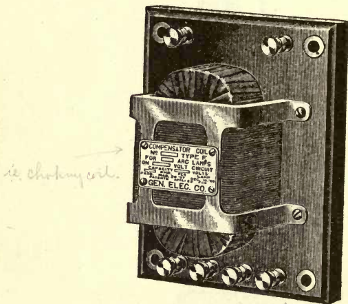
FIG. 51.—REACTIVE COIL OR COMPENSATOR FOR ARC LAMPS ON ALTERNATING-CURRENT CIRCUIT.
