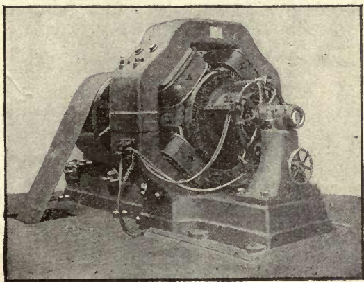
FIG. 16.—QUADRIPOLAR CONTINUOUS-CURRENT GENERATOR.
